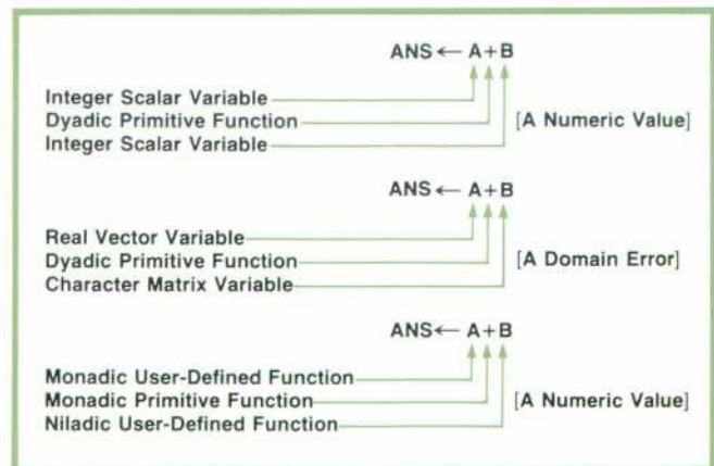
Fig. 1. APL is dynamic. Attributes of names may be arbitrarily changed by the programmer or by a program. For this reason, APL has been considered impossible to compile.
