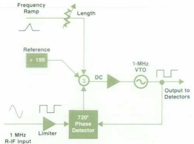
Fig. 14. Phase shifter consists of a 1-MHz voltage-tuned oscillator (VTO) that is phase-locked to the R-channel signal with a phase offset.
