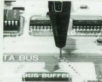
Figure 16-10. Logic Probe Inserted into D0 Test Hole
