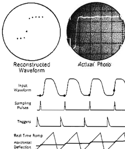
Figure 1. Waveforms pertinent to operation of sampling oscilloscope. Actual photo has 1000 samples which blend into continuous line.
