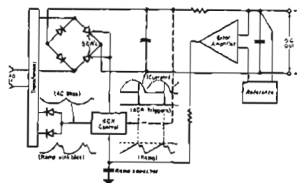
Figure 4. SCR regulated power supply.
