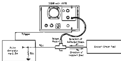
Figure 1. Basic time domain reflectometry setup.
