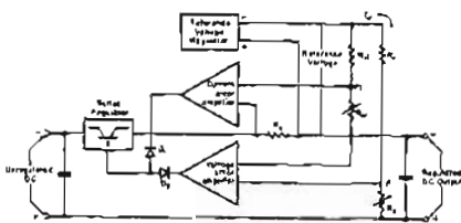
Figure 3. Constant voltage/constant current regulated power supply.
