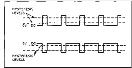
Figure 3. To enable a count on these waveforms the trigger level control must be out of PRESET to shift the hysteresis positive (upper waveform) or negative (lower waveform).
