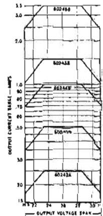
12 V Output Ratings 24V
