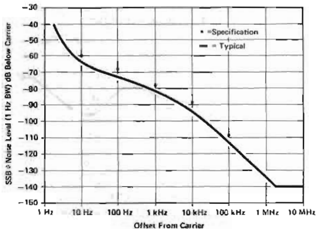
Figure 2. Typical 8672A single-sideband phase noise performance, 2.0–6.2 GHz. Add 8 dB for 6.2–12.4 GHz and 10 dB for 12.4–18 GHz.
