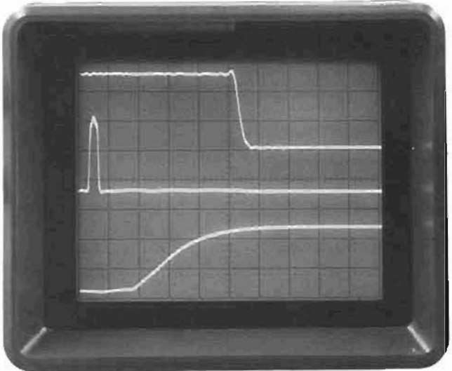
Time relationship of two very low rap rate signals is clearly shown with the variable persistence capability of the 1741A. The stable triggers required for this alternate sweep display to maintain time relationship were generated by the 1600A Logic State Analyzer.
