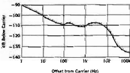
Typical single-sideband phase noise measured at output of Model 3330B Automatic Synthesizer in 1-Hz bandwidth with instrument operating at 12 MHz.
