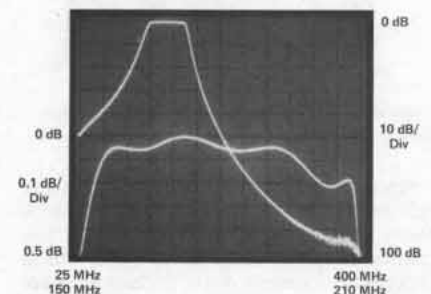
Figure 4. Automatic alternate sweep for coincident measurement of filter passband and skirts
