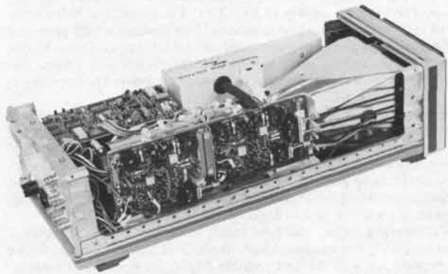
The well-designed interior layout and use of plug-in boards, multi-conductor cables, and multi-pin connectors make the 1332A, 1333A, 1335A, and 1336S very serviceable.
