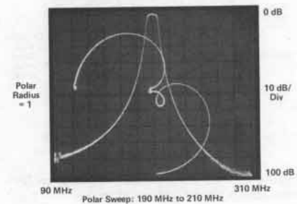
Figure 3. Simultaneous measurement of transmission response and passband reflection coefficient
