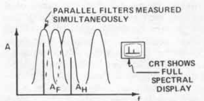
Figure 1c. Fourier analyzer
