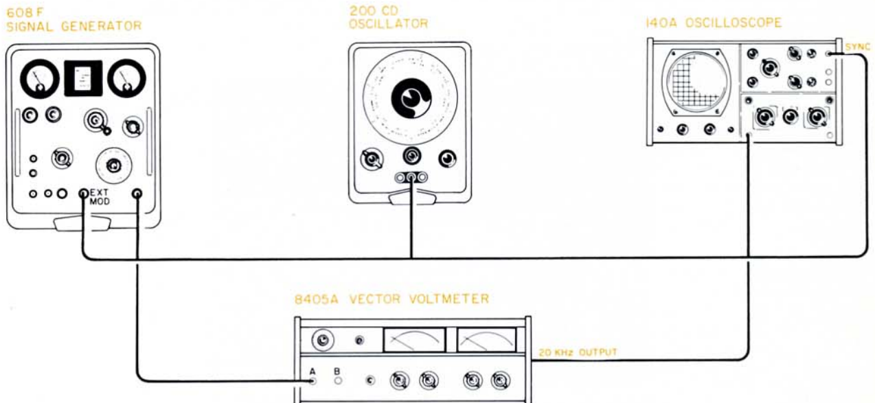
Figure 19. Test setup is used to check percent AM modulation of signal generators from 1 to 1,000 MHz by displaying 20-kHz IF signal of vector voltmeter on oscilloscope.
