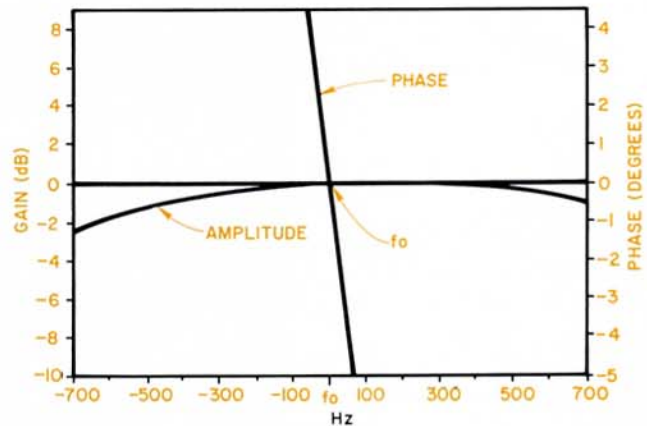
Figure 17. Plot of crystal filter of Figure 16 is greatly expanded near resonant frequency. Note the high phase versus frequency sensitivity which allows determination of resonant frequency with exceptional resolution.
