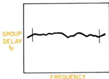
Figure 11. Phase response of device tested in Figure 10 has delay line or line stretcher inserted in reference channel. This allows higher phase resolution and accuracy in making relative group delay measurements.
