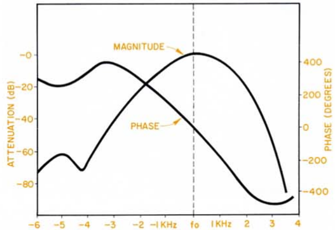
Figure 16. Amplitude and Phase Response of Narrow Band 20-MHz Crystal Filter.
