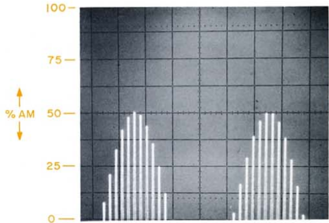
Figure 21. Oscilloscope offset technique allows percent AM to be read directly off oscilloscope graticule.
