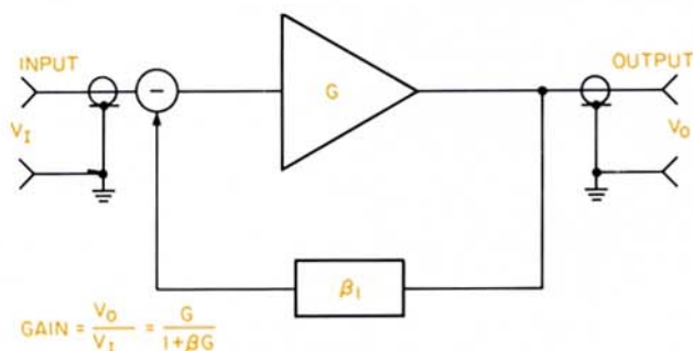
Figure 2a. Schematic Diagram of Typical Feedback Circuit.
