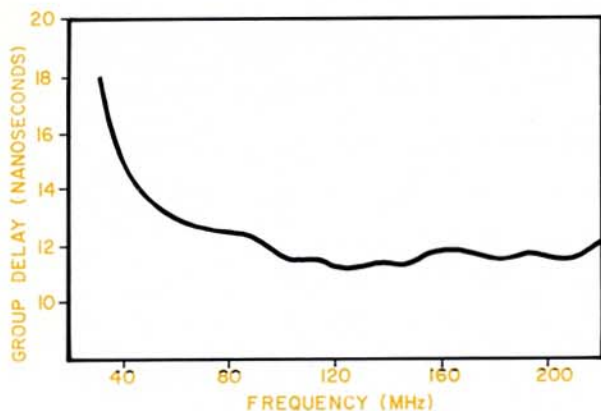
Figure 9. Group delay of a CATV amplifier is plotted directly from measurements of phase shift in degrees with frequency in 2.778-MHz steps. Group delay in nano-seconds is thus read directly from phase meter scale in degrees.
