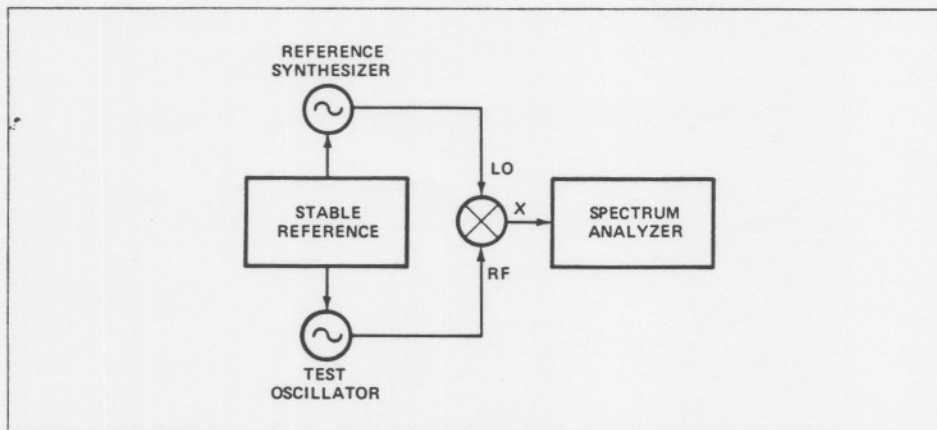
Figure 23. Block diagram for phase modulation tests on a phase-lock oscillator.
