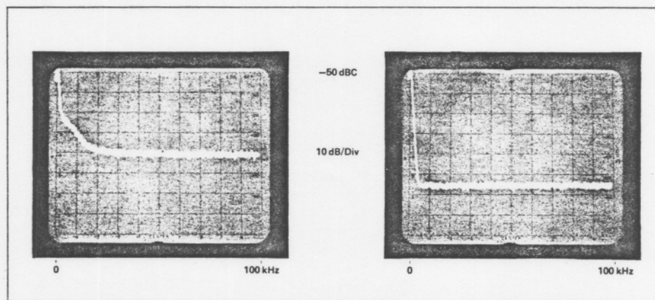
Figure 27. Residual phase modulation on a synthesized signal generator. In the left photo, the log reference level was calibrated at -50 \text{ dB} referred to the carrier. The IF bandwidth was 1 kHz. Then, the noise level is -118.3 \text{ dB/Hz} at 50 kHz ( -90 \text{ dB} + 2.5 \text{ dB} - 30.8 \text{ dB} ). The rise in the noise response below 20 kHz is caused by the synthesizer's phase-lock loop. The photo to the right shows the spectrum analyzer sensitivity.
