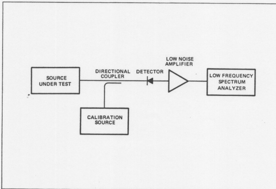
Figure 19. Block diagram for residual AM measurements.
