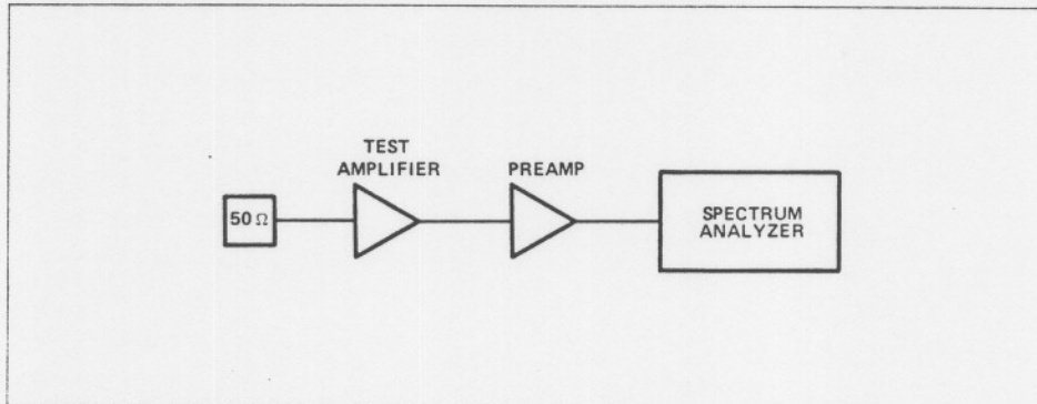
Figure 15. Noise figure test setup.
