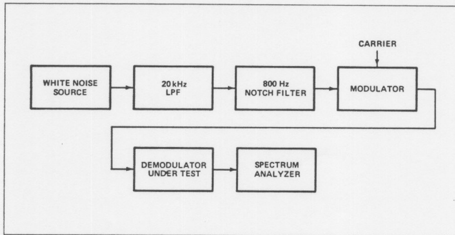
Figure 17. Basic white noise loading test.
