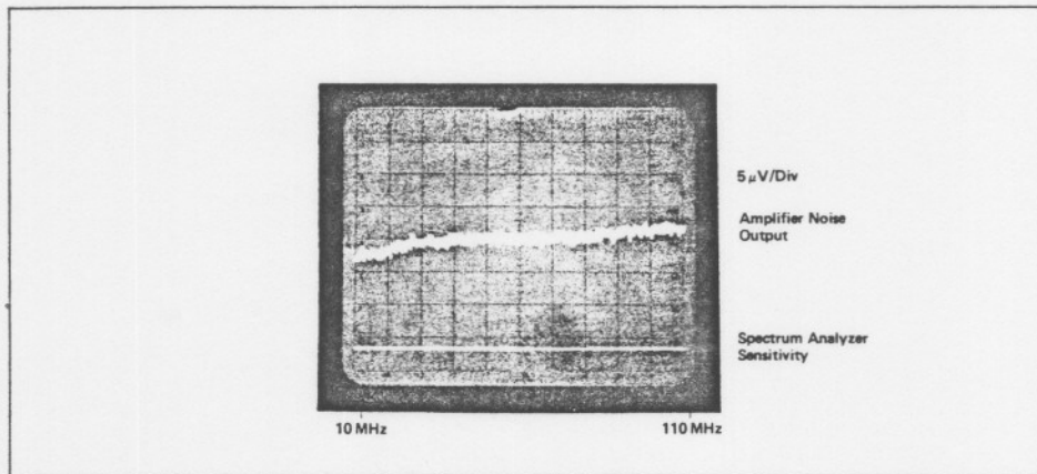
Figure 16. Example for noise figure measurement.
