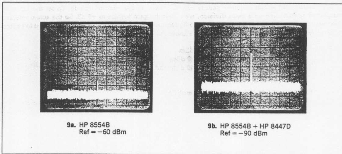
Figure 9. Enhancement of the sensitivity of the HP 8554B Spectrum Analyzer (0.1 to 1250 MHz) with the HP 8447D Preamplifier (Gain = 26 dB; 0.1 to 1300 MHz). The same power signal is displayed in both photos. The sensitivity is improved by 20 dB in Figure 9b.
