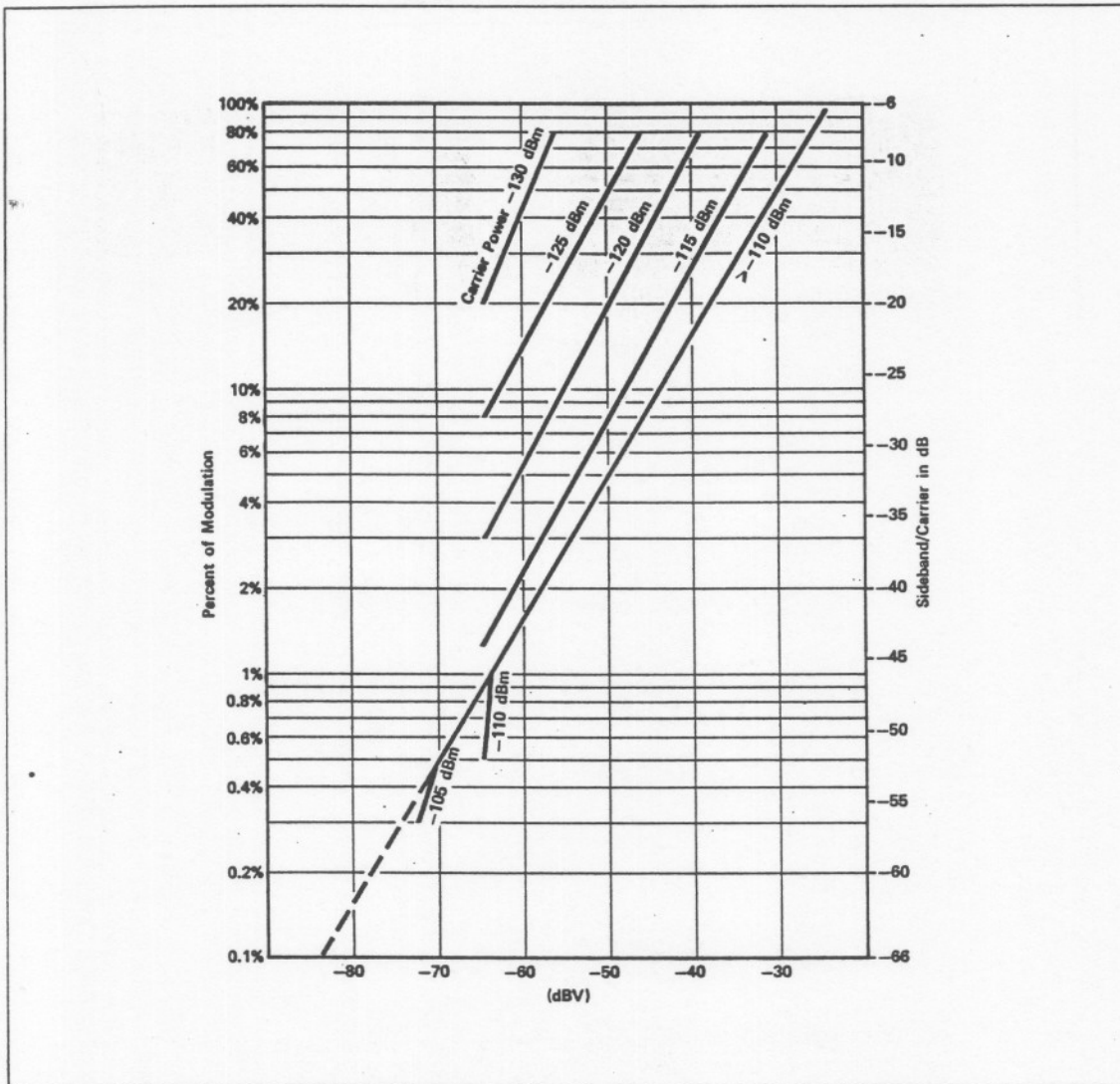
Figure 17. Percentage of modulation versus dBV for one system based on the instruments listed in Figure 16. The curves of conversion of dBV to percentage of modulation must be drawn for each system. The conversion depends on the carrier power. For example, for a signal at -125 dBm, a spectral line at -63 dBV on the display of the low frequency Spectrum Analyzer corresponds to 10% of modulation or the side bands are at -26 dB relative to the carrier or at -125 dBm -26 dB = -151 dBm.
