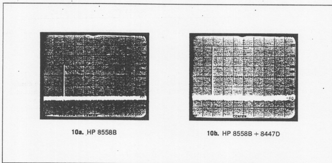
Figure 10. Measurement of Harmonics of a Weak Signal
