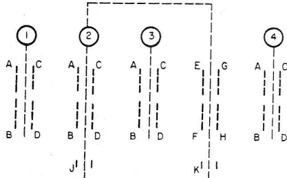
PUSH BUTTON SWITCH - CONTACT LAYOUT
