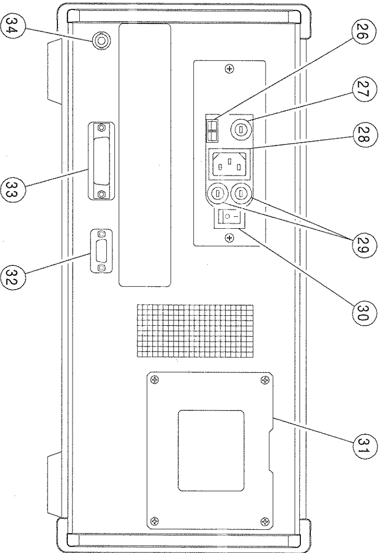
COM-120B Rear Panel
