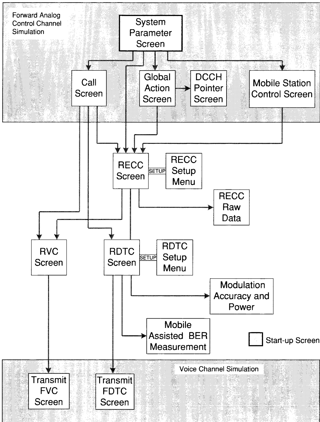
Analog Control Channel Cell Site Simulation Screen Hierarchy
