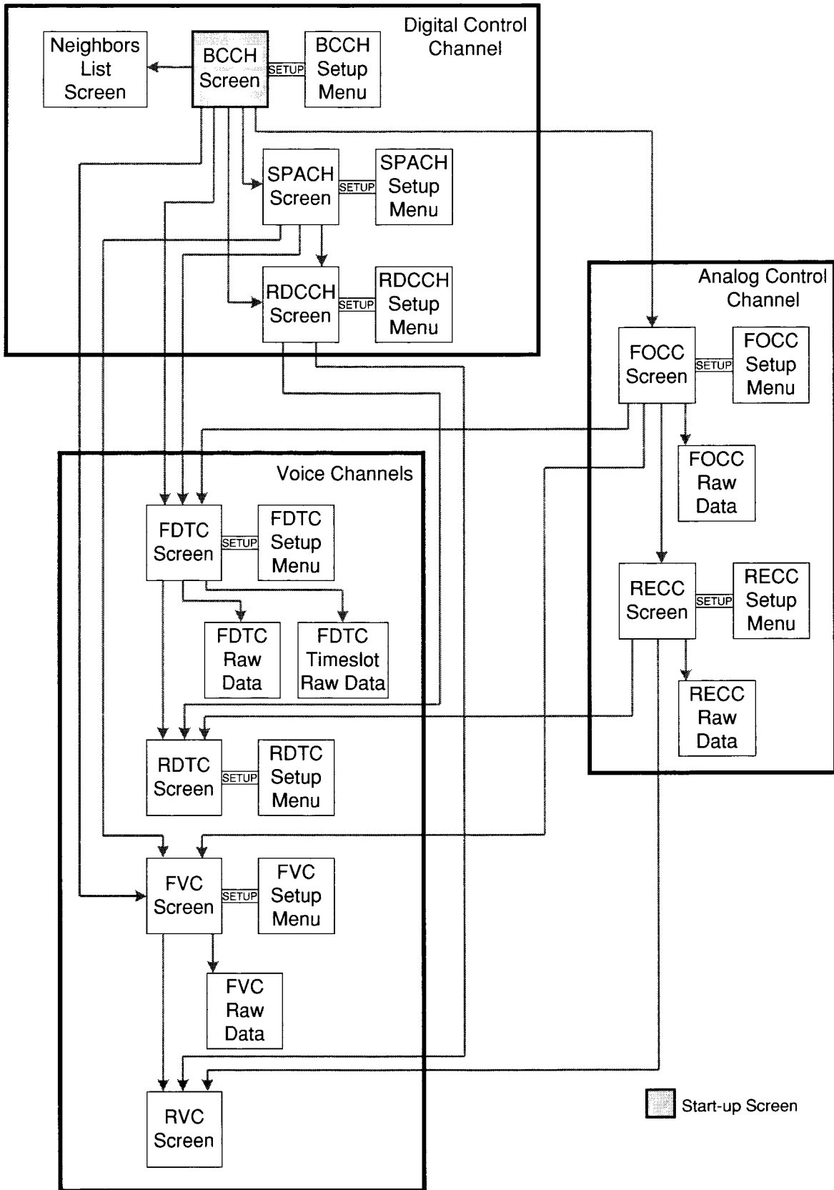
TIA/EIA-136 Cellular Data Monitor Screen Hierarchy
