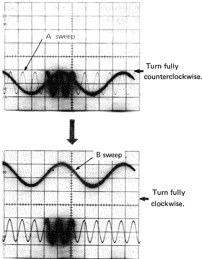
Figure 2-20. Where V Trigger Signal is Positive
