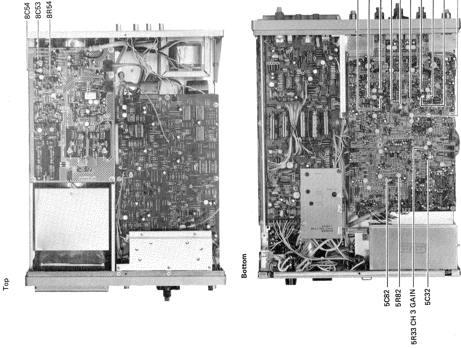
Figure 6-9-4. Adjustment locations (VERTICAL DEFLECTION SYSTEM II)
