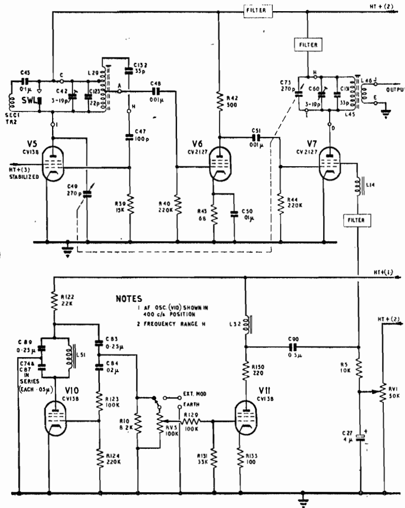
Fig. 3. Amplitude Modulation Circuit
