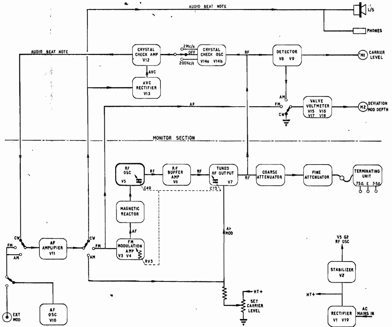
Fig. 3. Block Diagram
