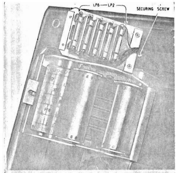
Fig. 2. Scale drive unit
