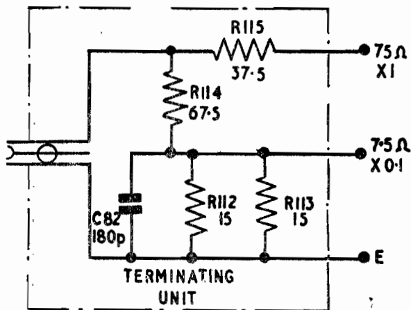
Fig. 3. Terminating Unit—Circuit
