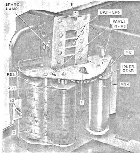
Fig. 2. Film scale sub-chassis
