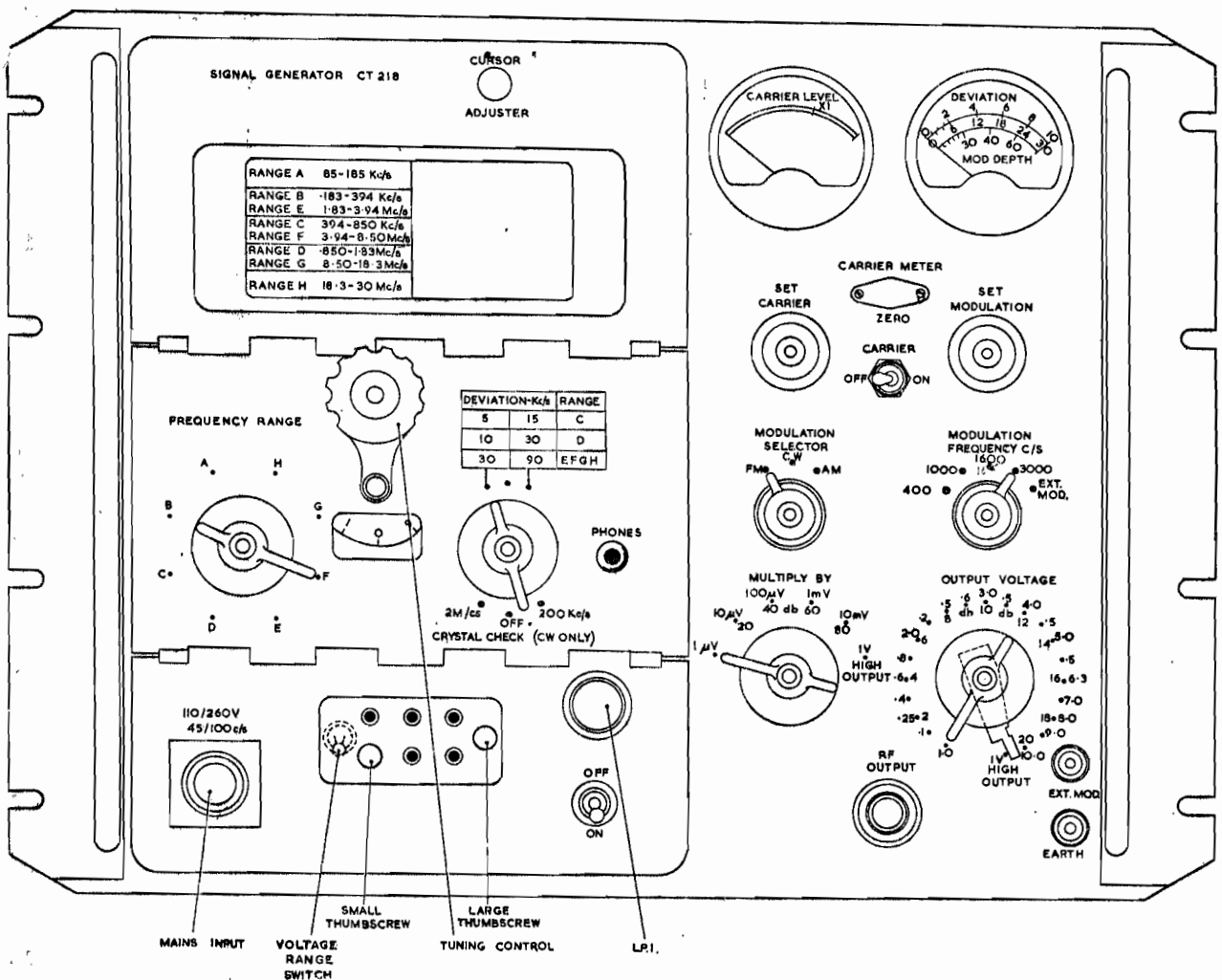
Fig. 1. Front Panel
