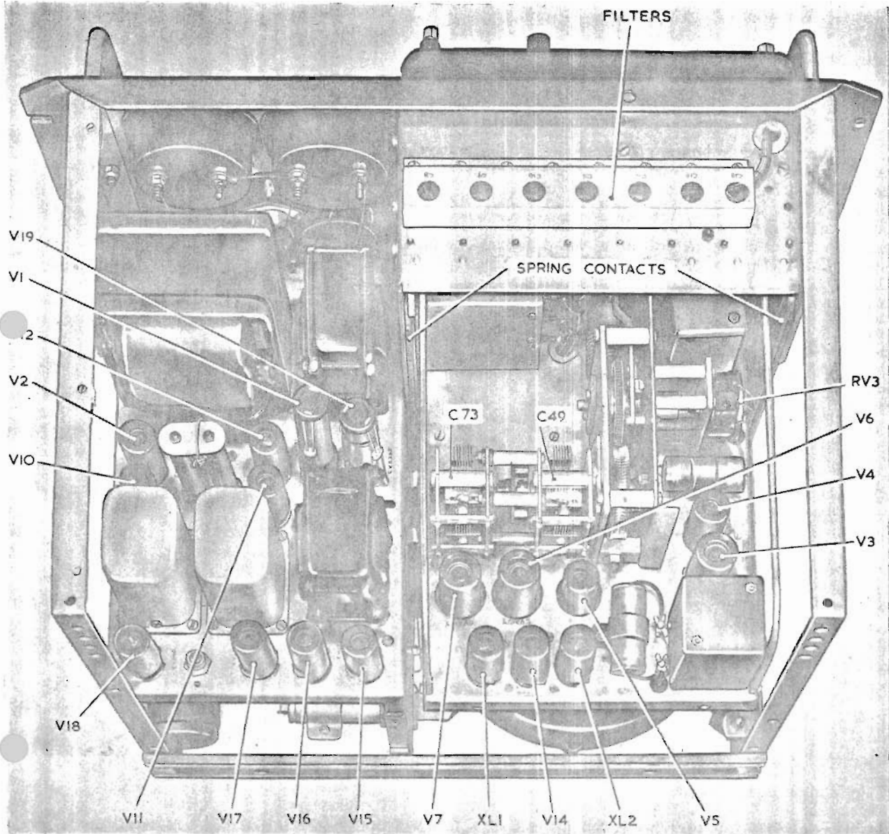
Fig. 4. Interior view of chassis
