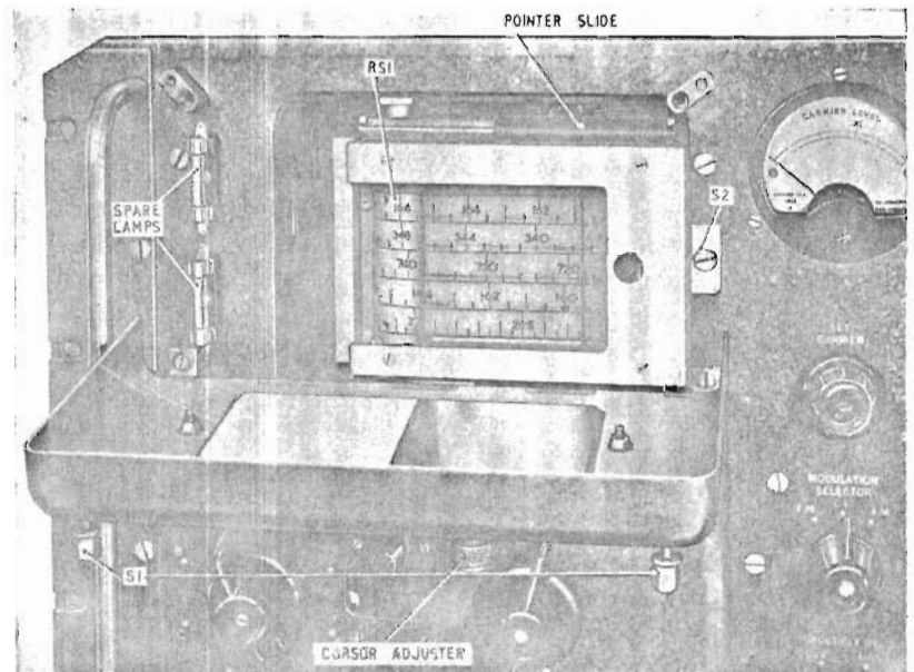
Fig. 3. Front panel with top cover open
