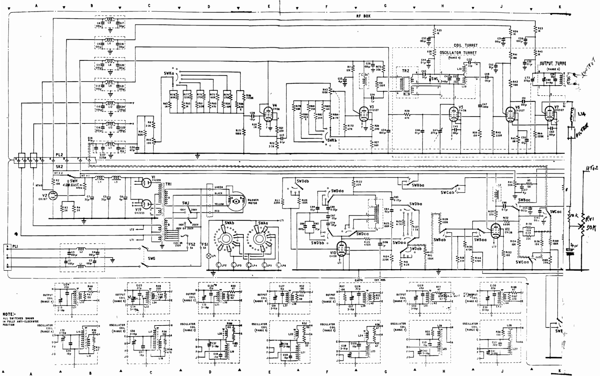
Signal generator CT218 - circuit
