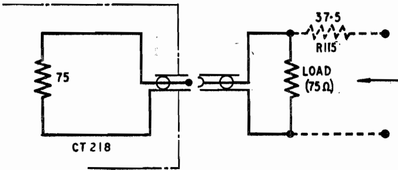
Fig. 2. Terminating unit
