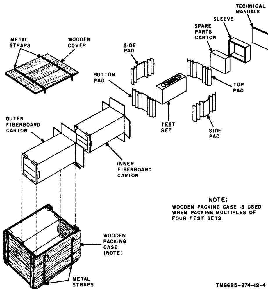
Figure 5. Typical packaging.
