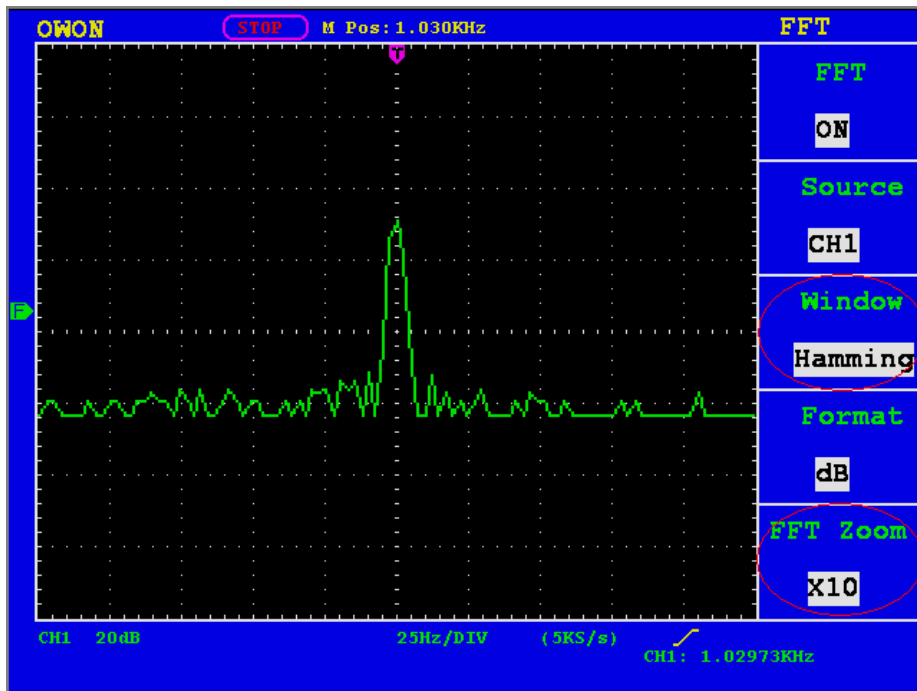
Fig.22 Hamming window
