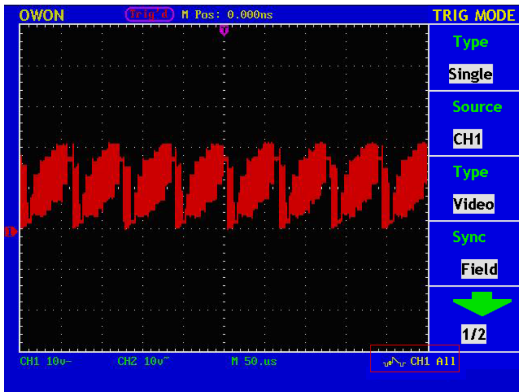
Fig.39 Wave Form Triggered in the Video Line
