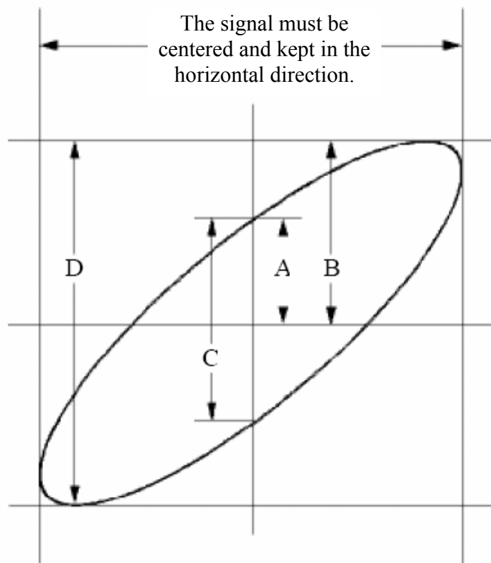
Fig.70 Lissajous Graph
