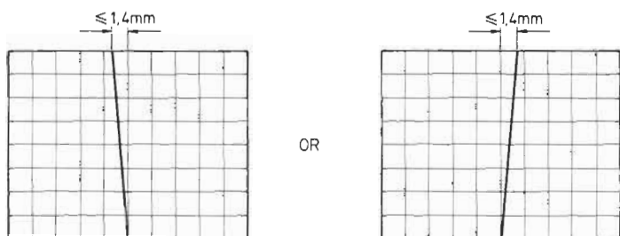
Figure 4.2. Orthogonality
