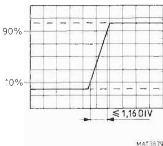
Figure 4.3 Rise-time.
