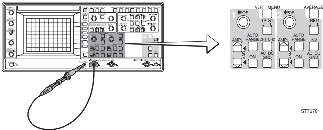
Figure 3.5 Vertical setup
