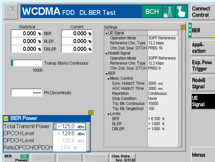
FIG 5 BER measurement.
