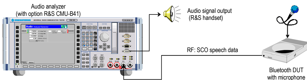
Fig. 4-79 Receive audio tests
