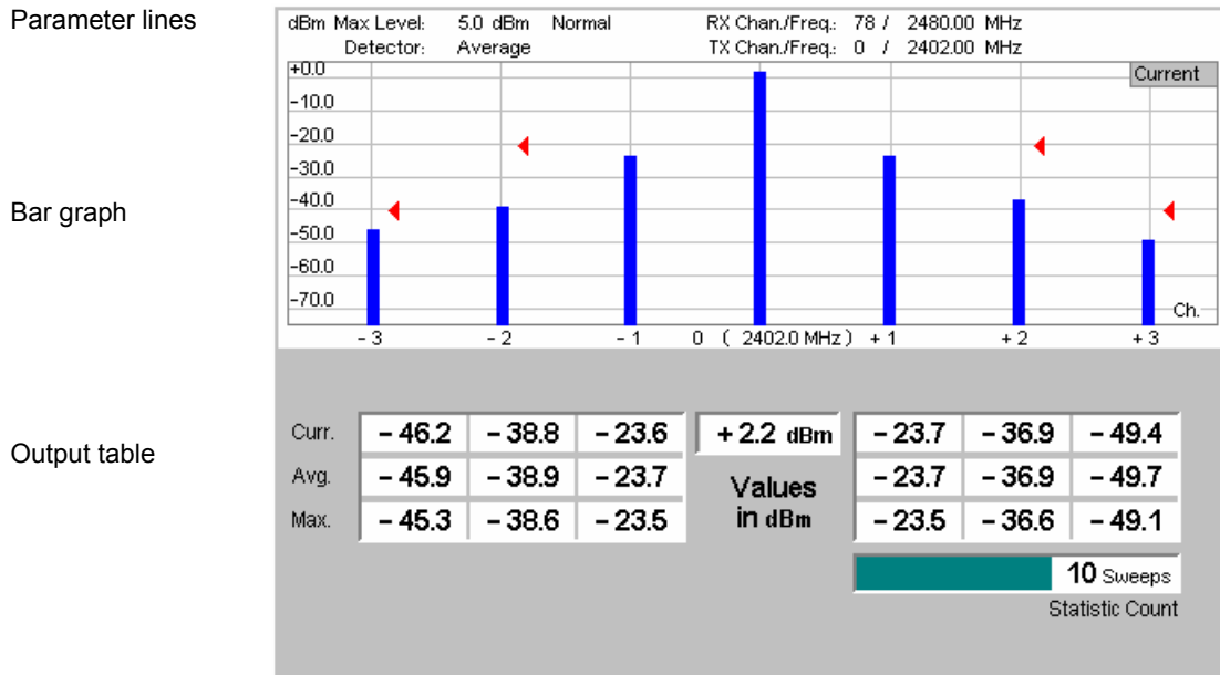
Fig. 4-67 Display of results (ACP)
