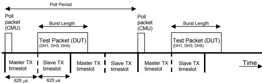
Fig. 4-93 Timing for transmitter tests
