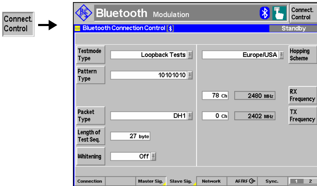
Fig. 4-91 Connection Control – Slave Sig. (panel)
