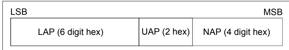
Fig. 4-84 Bluetooth address format
