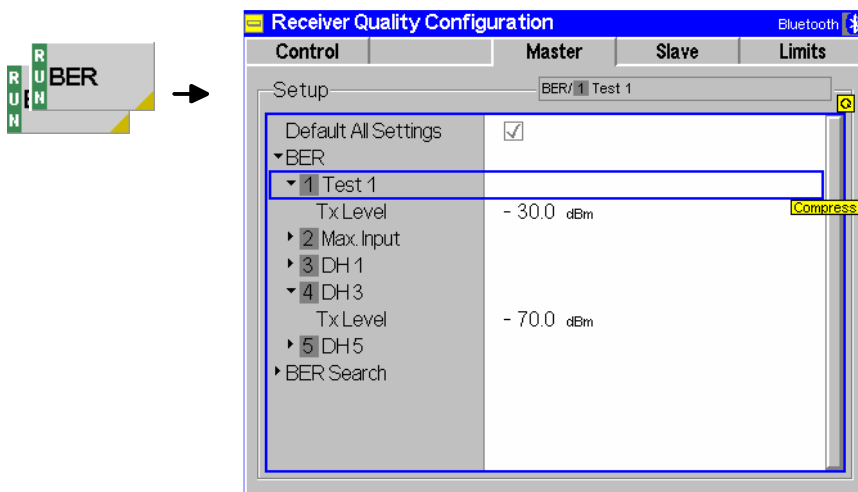
Fig. 4-76 Receiver Quality – Master
