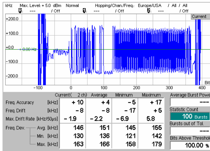
Fig. 4-57 Display of measurement results (Modulation menu)
