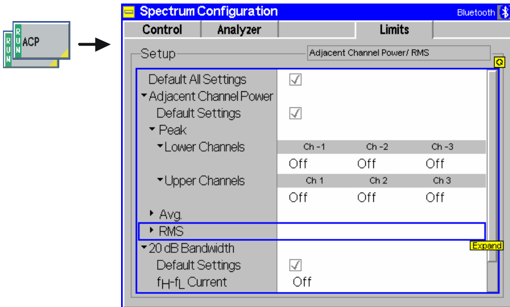
Fig. 4-72 Spectrum Configuration – Limits
