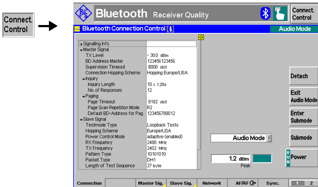
Fig. 4-88 Connection Control – Connection (Audio)
