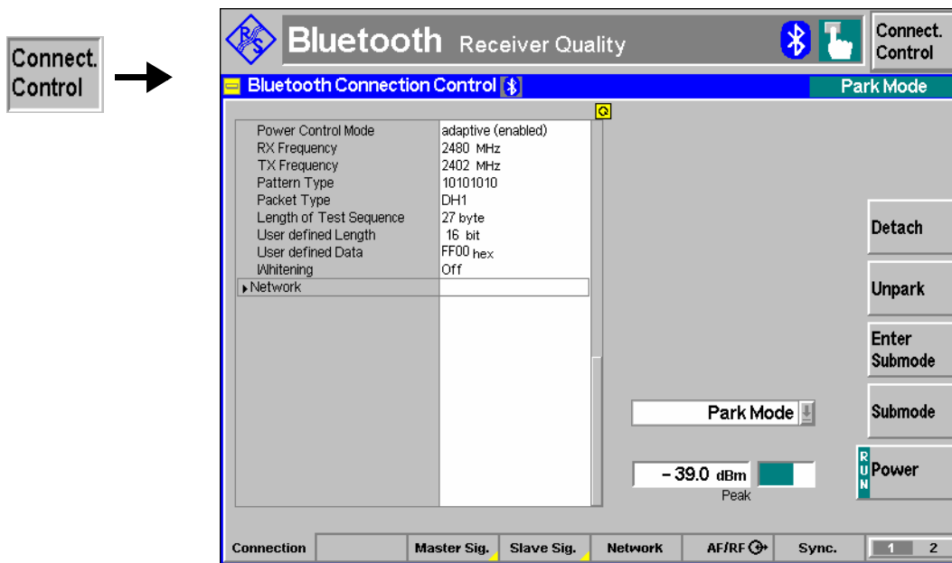
Fig. 4-87 Connection Control – Connection ( Park )
