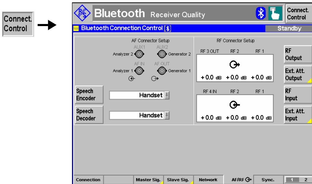
Fig. 4-97 Connection Control – AF/RF connectors
