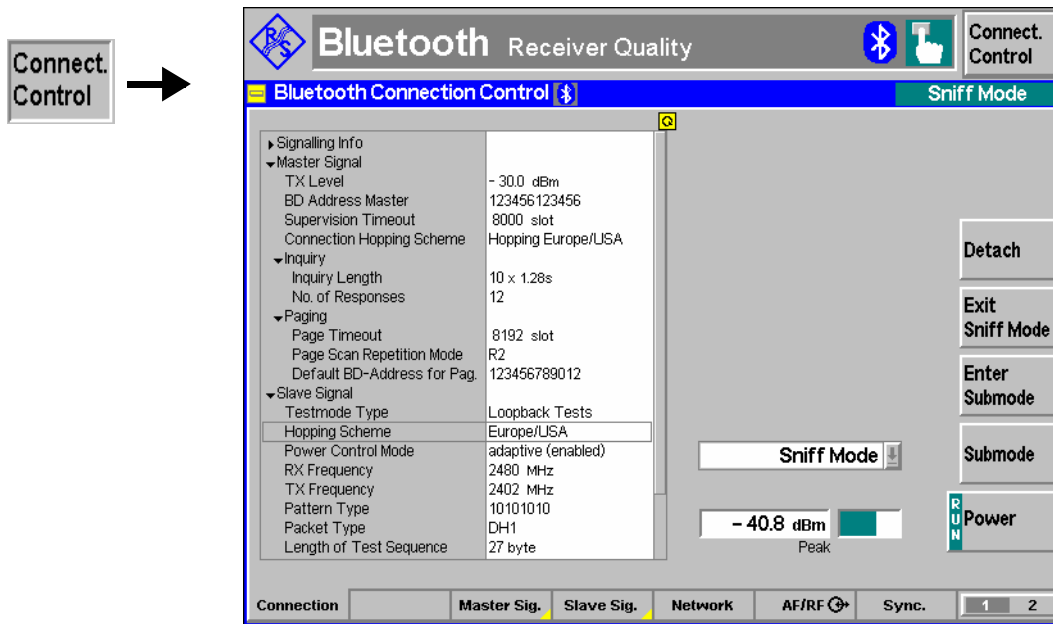
Fig. 4-85 Connection Control – Connection (Sniff)
