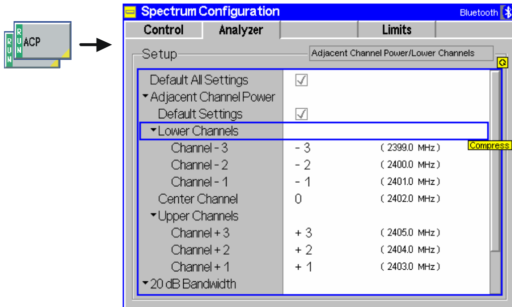
Fig. 4-71 Spectrum Configuration – Analyzer
