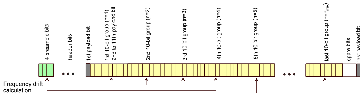
Fig. 4-59 Calculation of Frequency Drift
