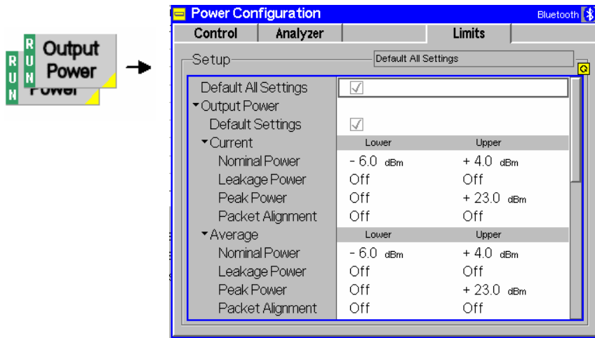
Fig. 4-54 Power Configuration – Limits
