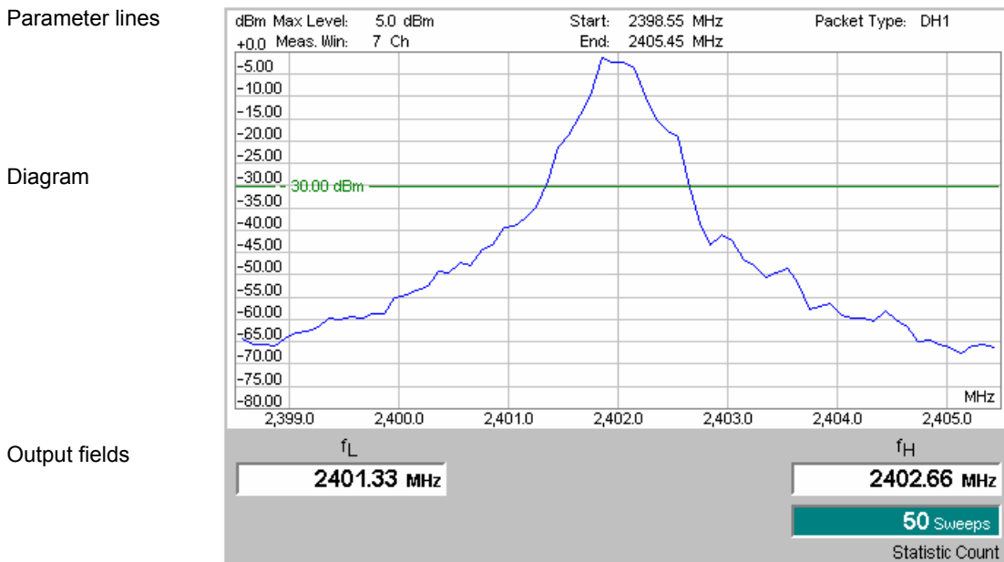
Fig. 4-69 Display of results (Frequency Range)
