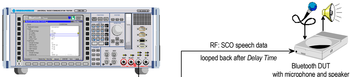
Fig. 4-81 Echo tests
