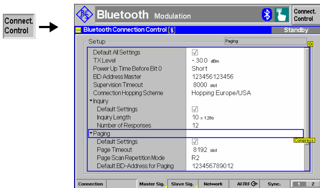
Fig. 4-90 Connection Control – Master Sig. (table)
