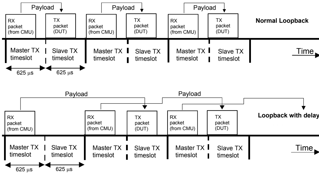
Fig. 4-94 Timing for loopback tests
