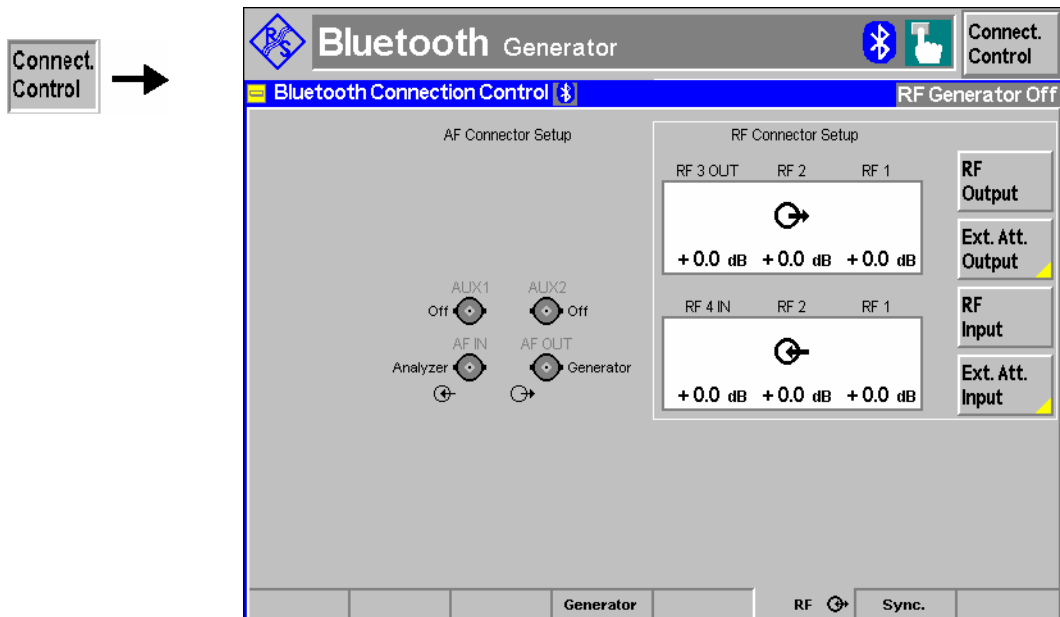
Fig. 4-38 Connection Control – RF connectors
