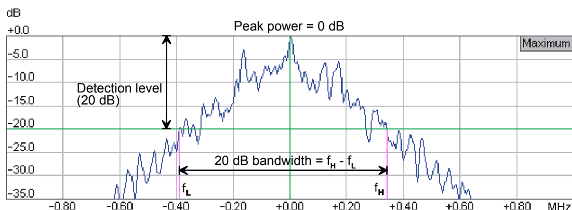
Fig. 4-65 20 dB bandwidth measurement
