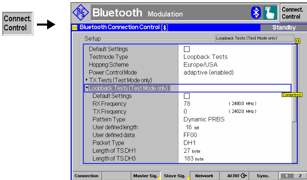
Fig. 4-92 Connection Control – Slave Sig. (table)
