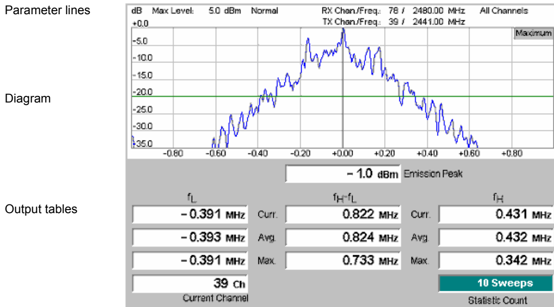
Fig. 4-68 Display of results (20 dB Bandwidth)
