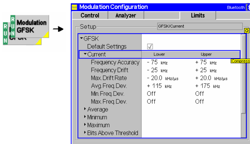
Fig. 4-63 Modulation Configuration – Limits
