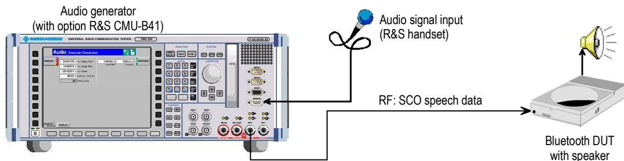
Fig. 4-80 Transmit audio tests
