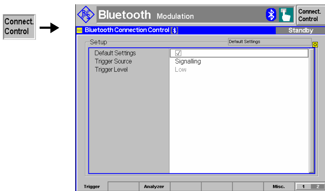
Fig. 4-98 Group Configuration – Trigger
