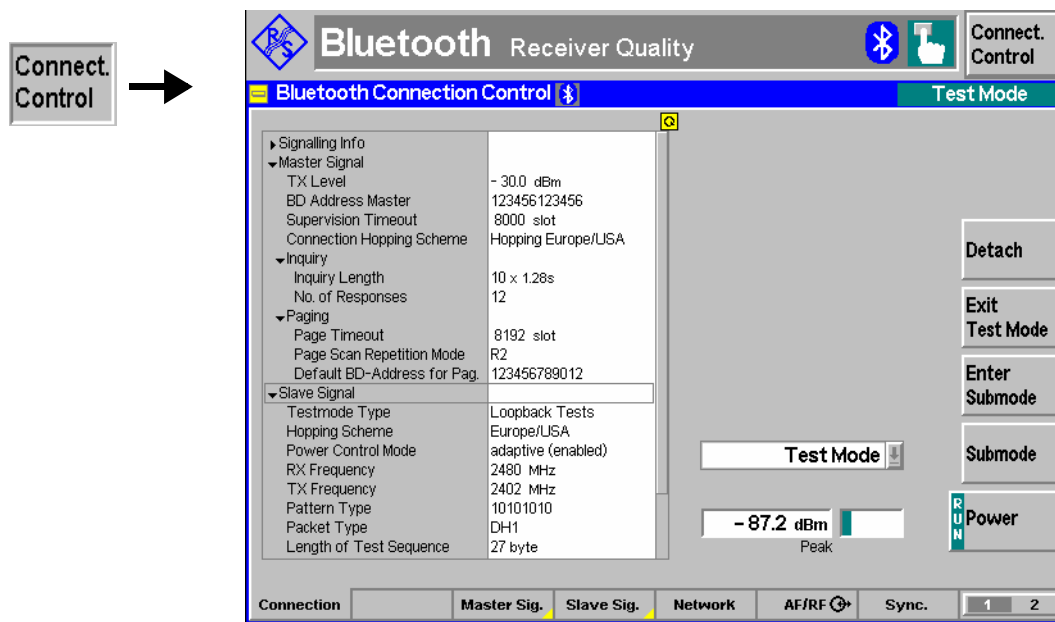
Fig. 4-83 Connection Control – Connection (Test Mode)
