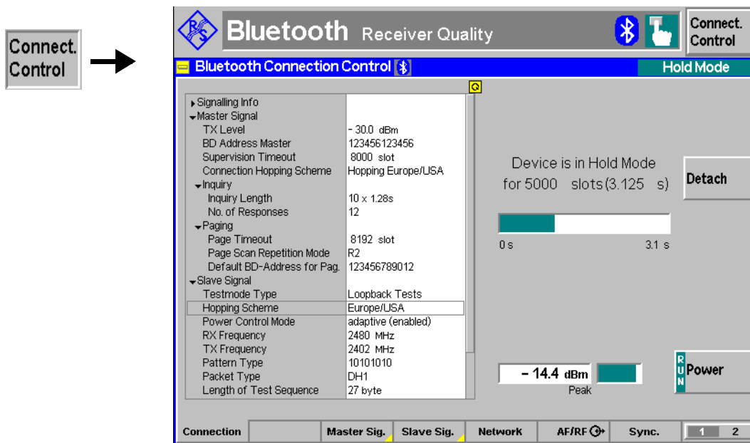
Fig. 4-86 Connection Control – Connection (Hold)
