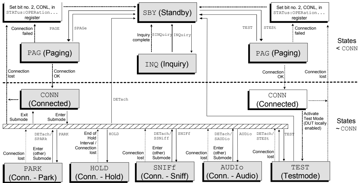
Fig. 6-1 Signalling states (shaded) of the R&S ® CMU and transitions
