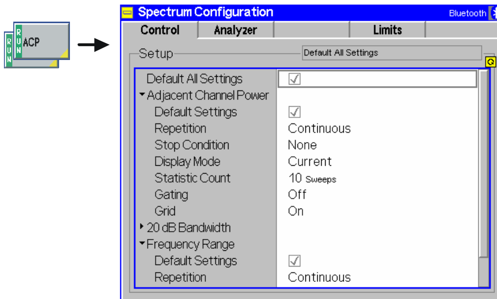
Fig. 4-70 Spectrum Configuration – Control
