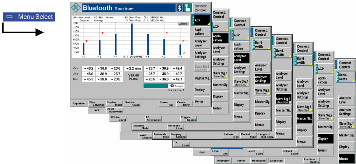
Fig. 4-66 Measurement menu Spectrum
