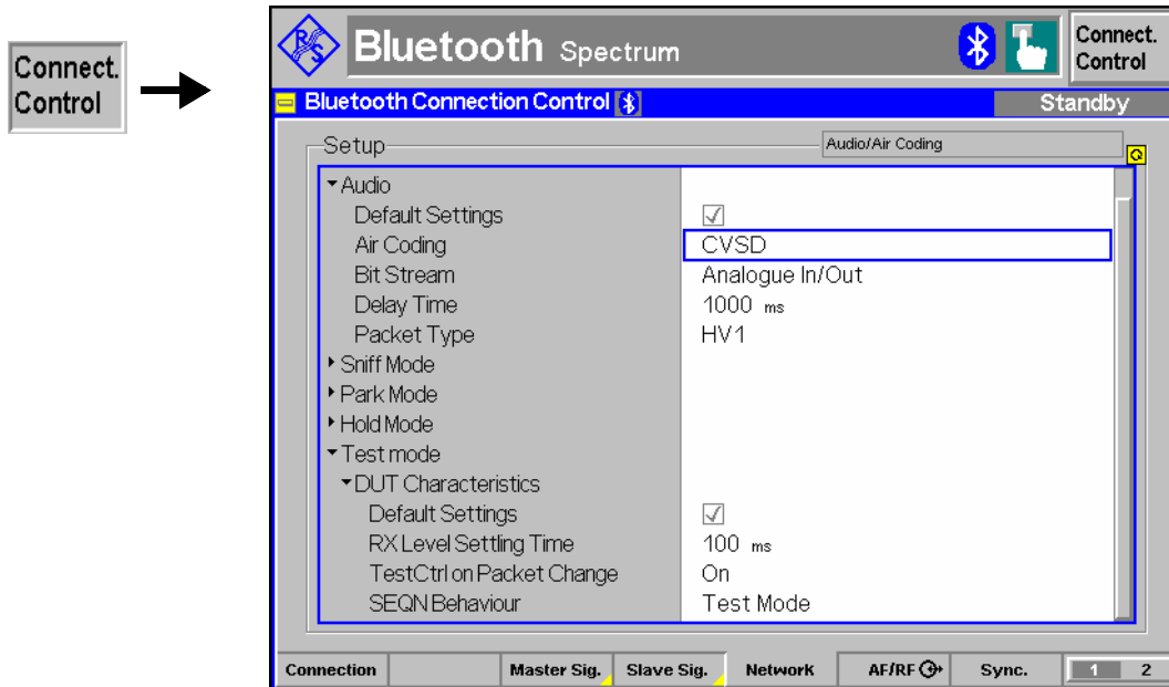
Fig. 4-95 Connection Control – Network (table)
