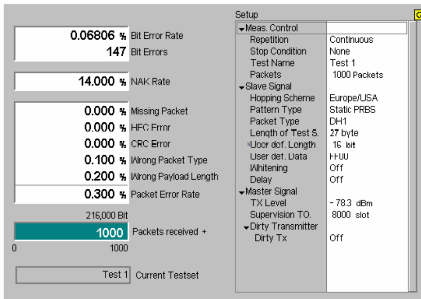
Fig. 4-74 Display of test settings and measurement results (BER)
