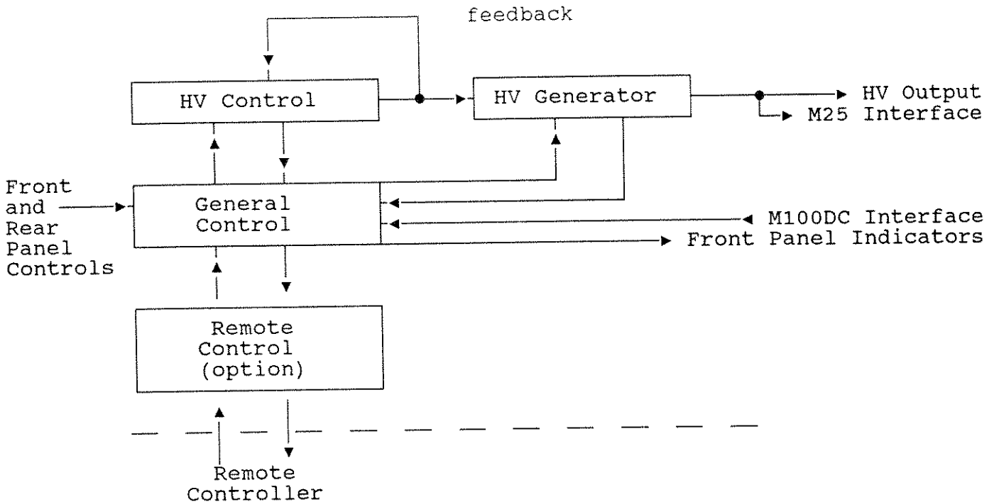
Figure 3-1: Functional Diagram
