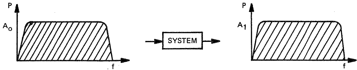
3A – Reference Power Measurement
