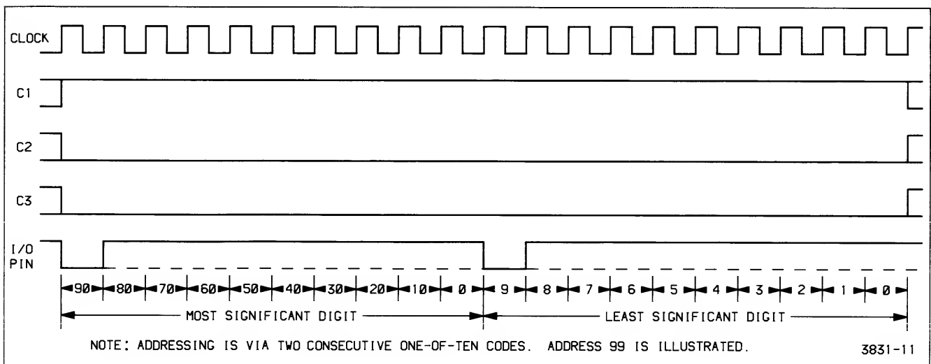
Figure 3-3. Accept address timing.
