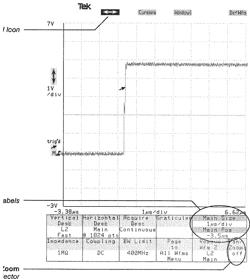
Horizontal Controls
