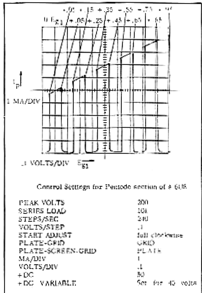
Fig. 2-11. Plate Current vs. Grid Voltage curves for the pentode section of a 6U8.
