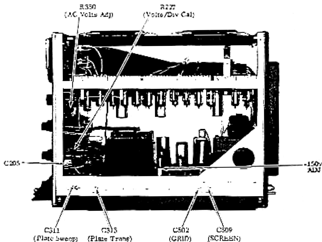
Fig. 3-7. Internal view of Type 570.
