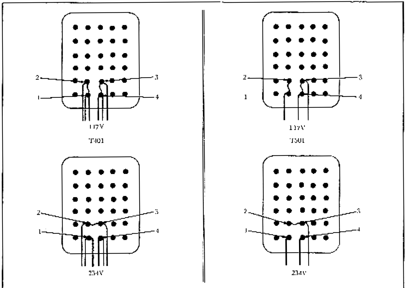
Fig. 2-1. Connections to be made when the Type 570 is connected for 254 (117) volt operation.
