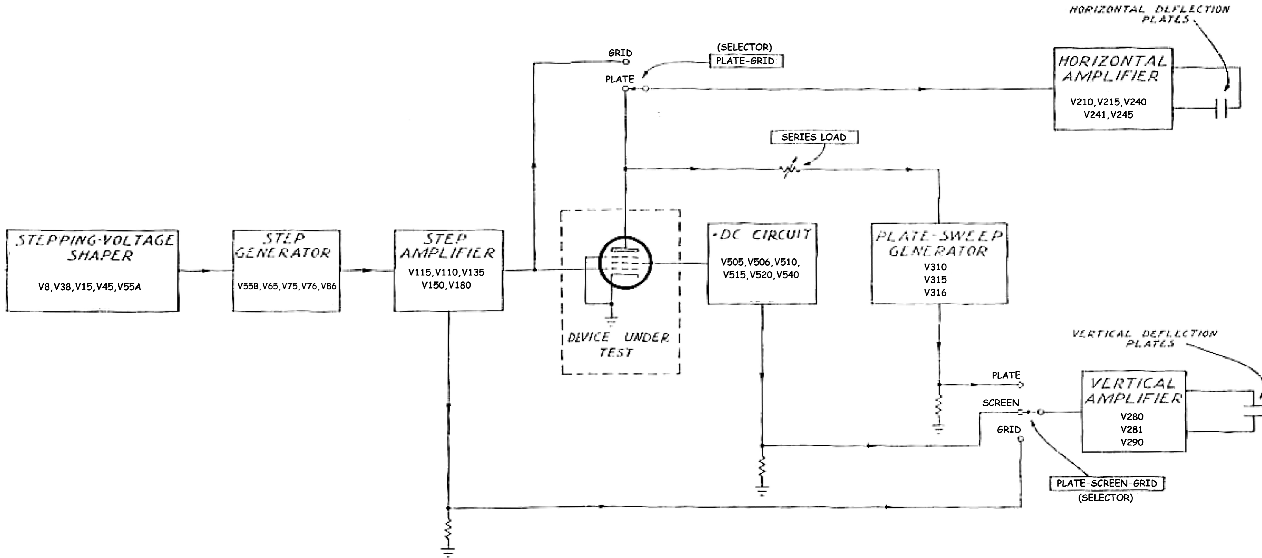
BLOCK DIAGRAM
