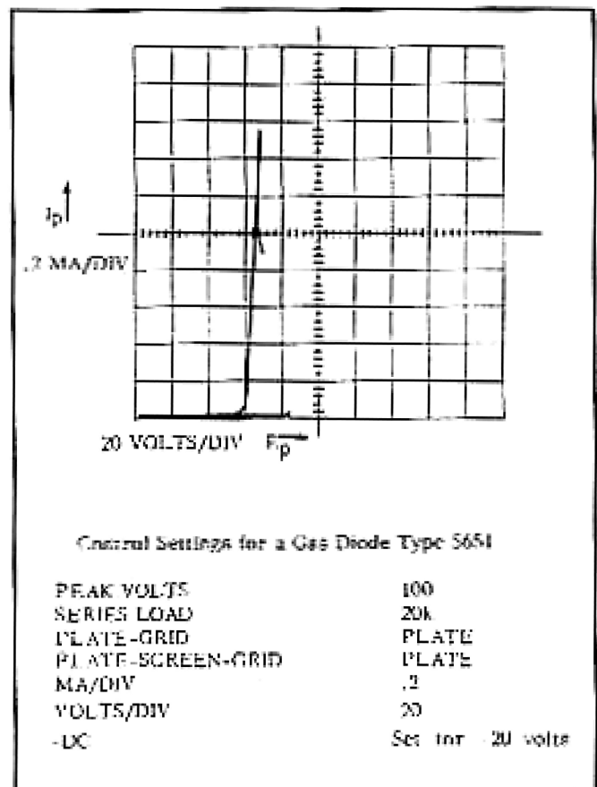
Fig. 2-16. Displaying the firing potential and voltage drop of a type 5651 gas diode. Note the cathode is connected to the -1X' electrode.
