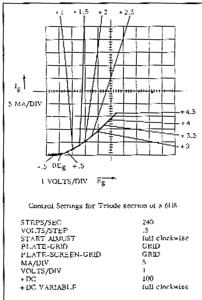
Fig. 2-8. Grid Current vs. Grid Voltage curves for the triode section of a 6U8. Now +DC connector supplied the plate voltage.
