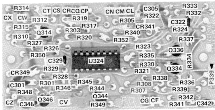
Fig. 8-4. A3. Trigger Selector circuit board.
