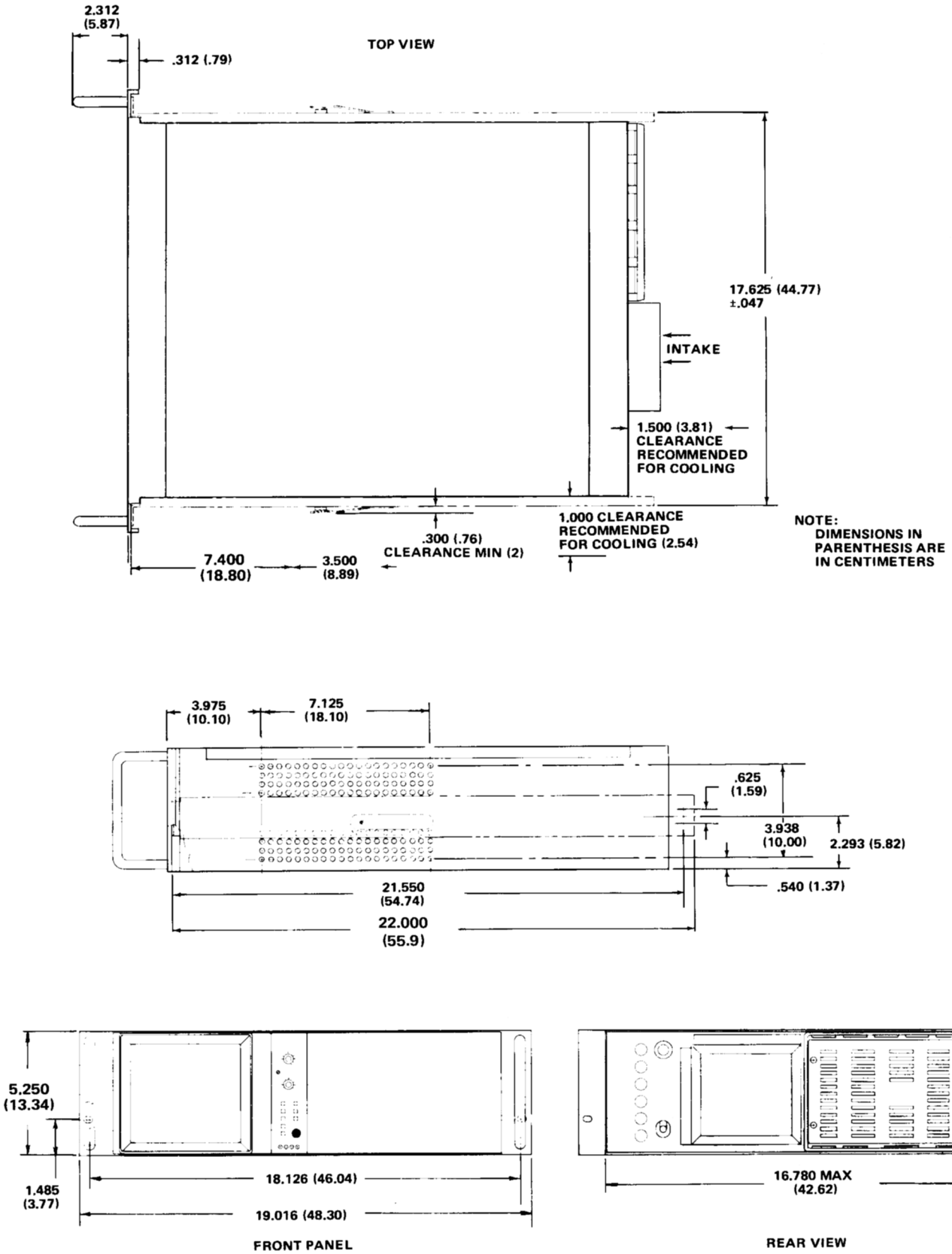
Fig. 6-6. Dimensional drawing.
