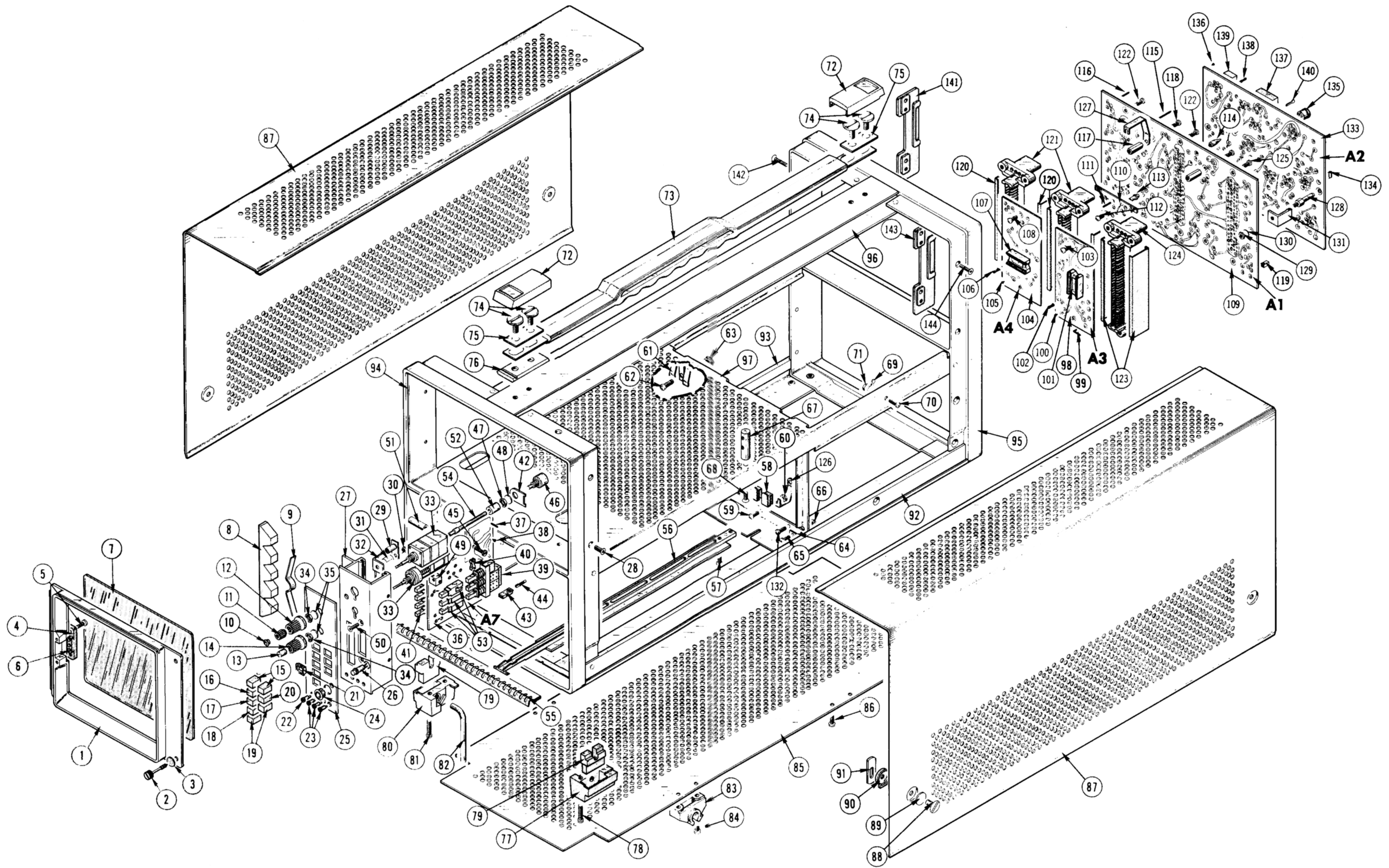
7603/R7603 OSCILLOSCOPE
