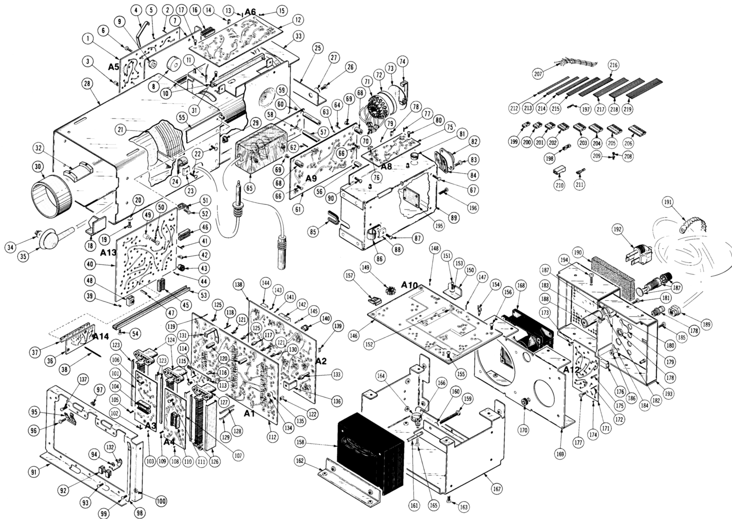
7603/R7603 OSCILLOSCOPE
