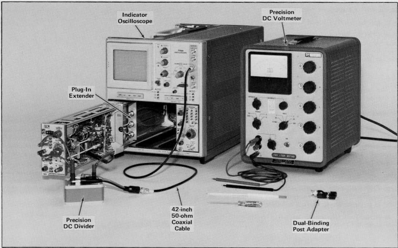
Fig. 5-7. Initial setup showing equipment required for performing calibration steps 12 through 16. To continue the Performance Check procedure, go to step 16A.
