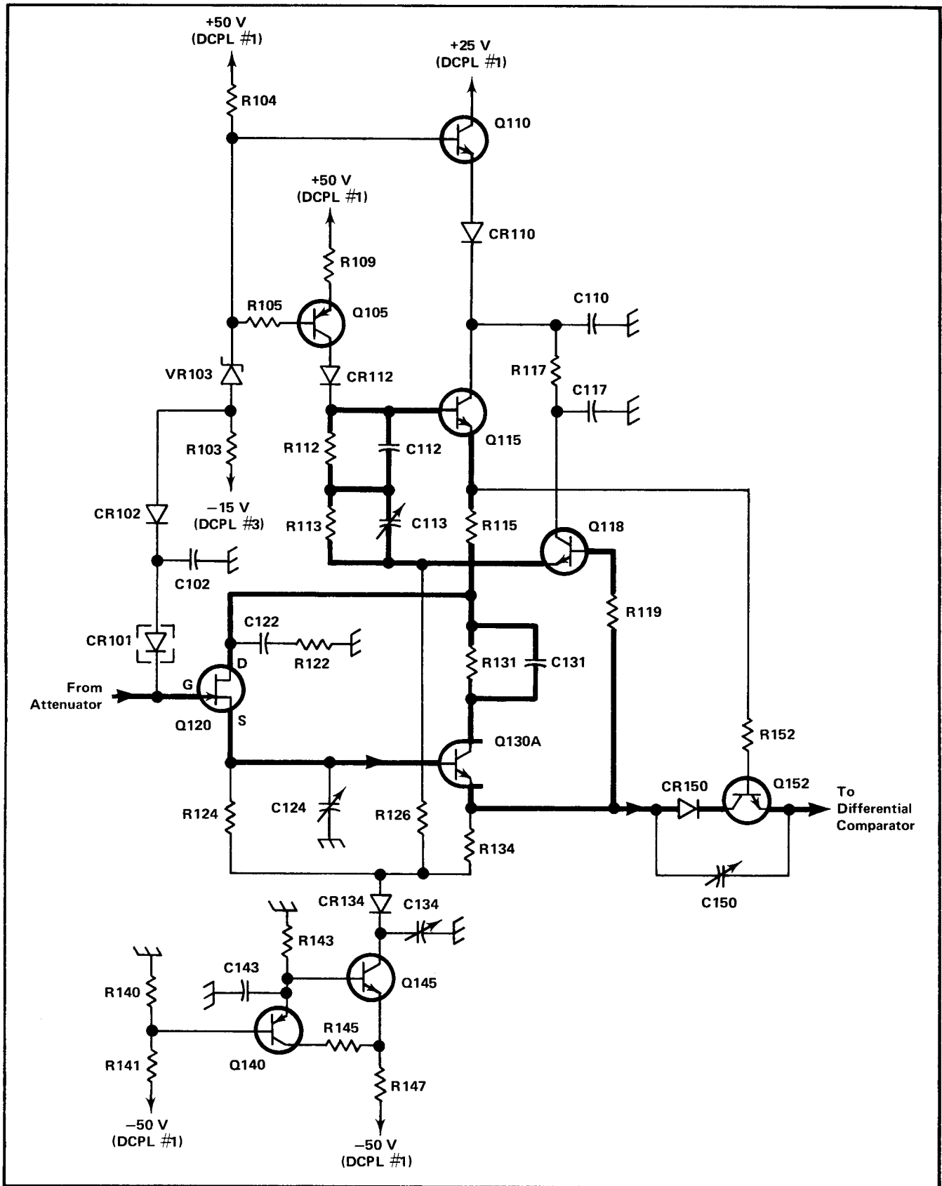
Fig. 3-1. Input Source and Emitter Follower, simplified schematic diagram.
