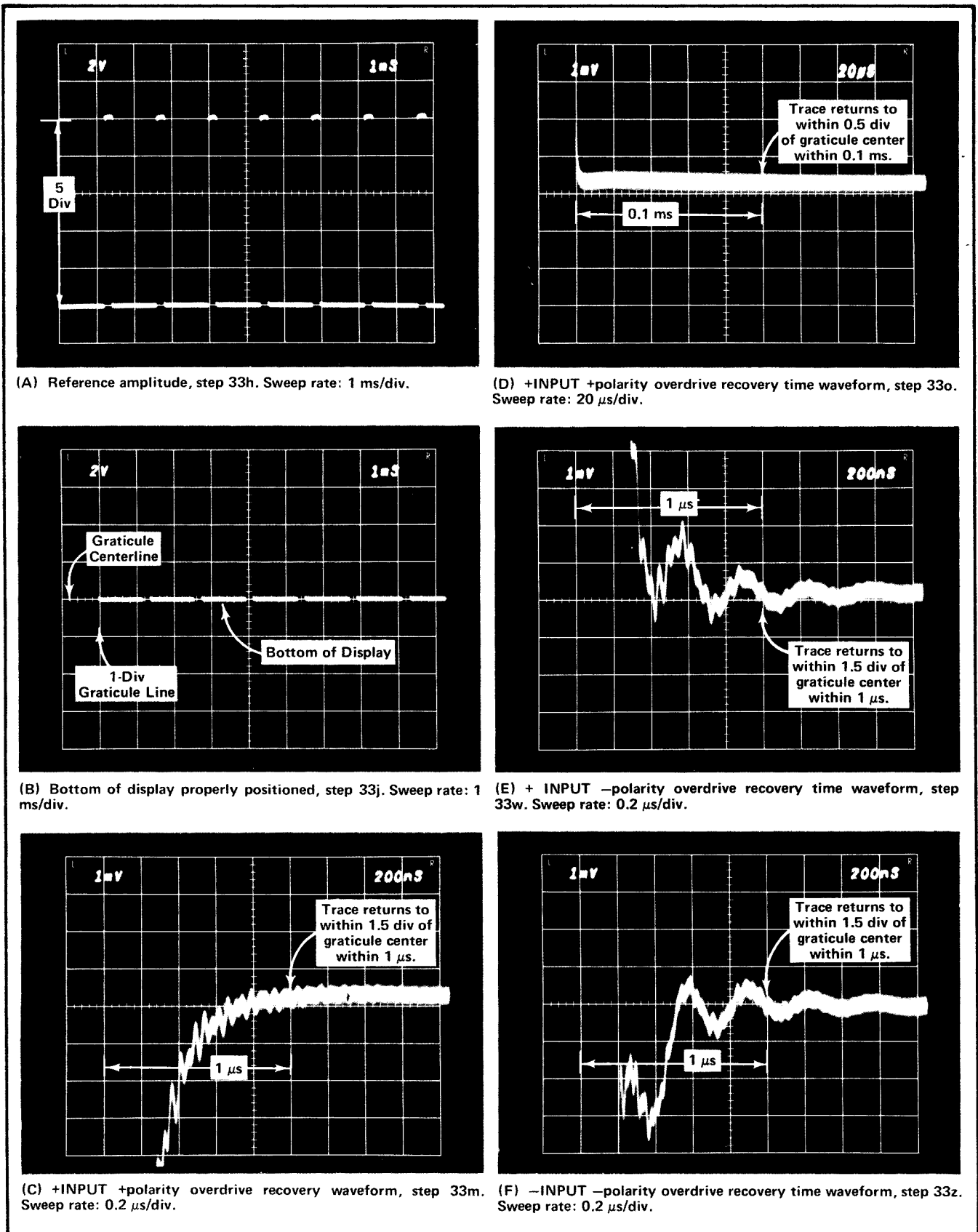
Fig. 5-31. Examples of waveforms obtained when checking override recovery time. Vertical deflection factor for waveforms (A) and (B) is 2 V/div; remaining waveforms are 1 mV/div.
