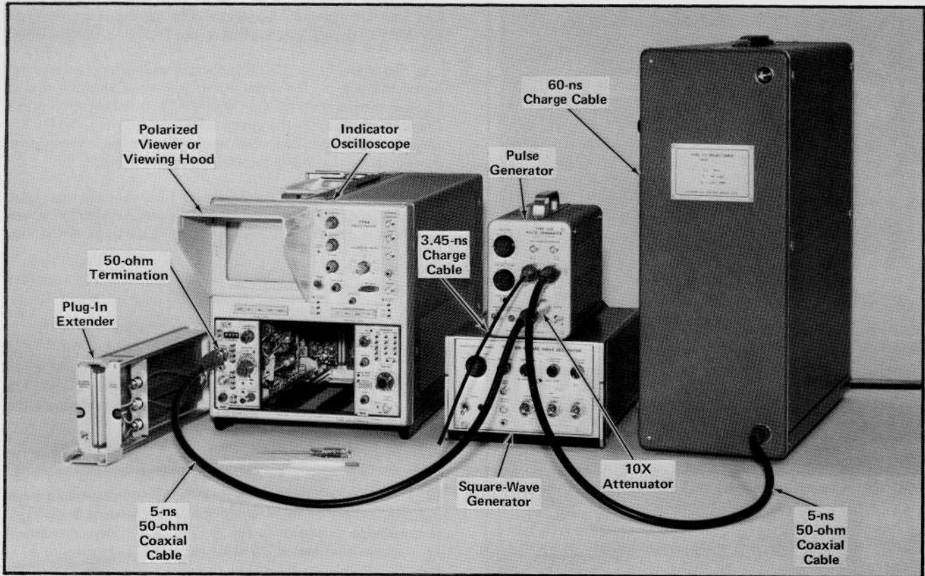
Fig. 5-11. Initial setup showing equipment required for performing the high-frequency compensation calibration checks and adjustments. The plug-in extender is not needed for a performance check.
