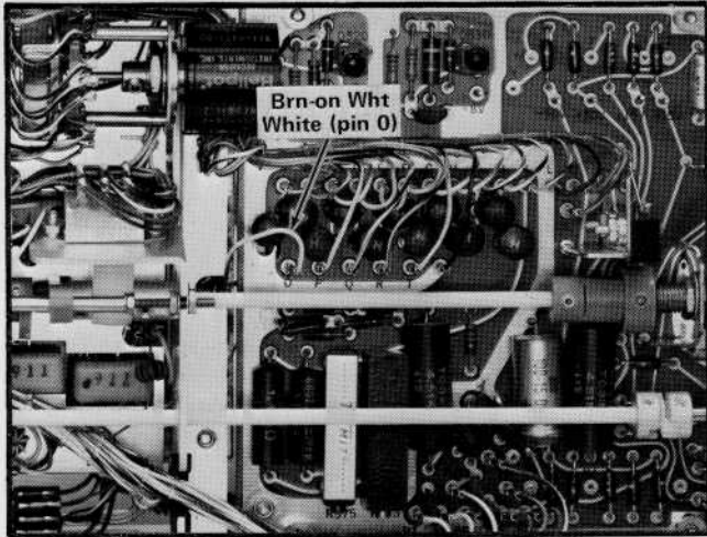
Fig. 5-9. Partial view of Output board showing the Vc input wire and the Vc output pin connector location.
