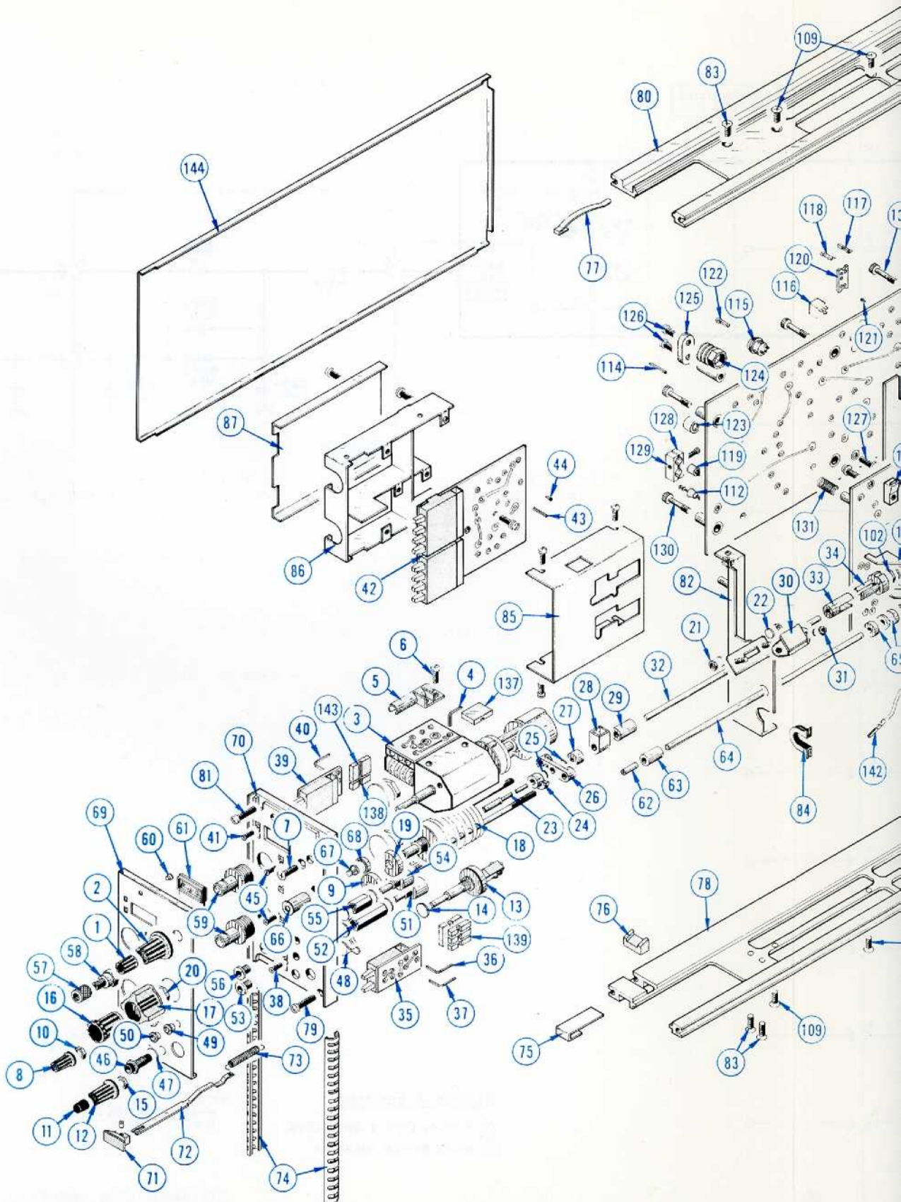
TYPE 7A13 DIFFERENTIAL COMPARATOR
