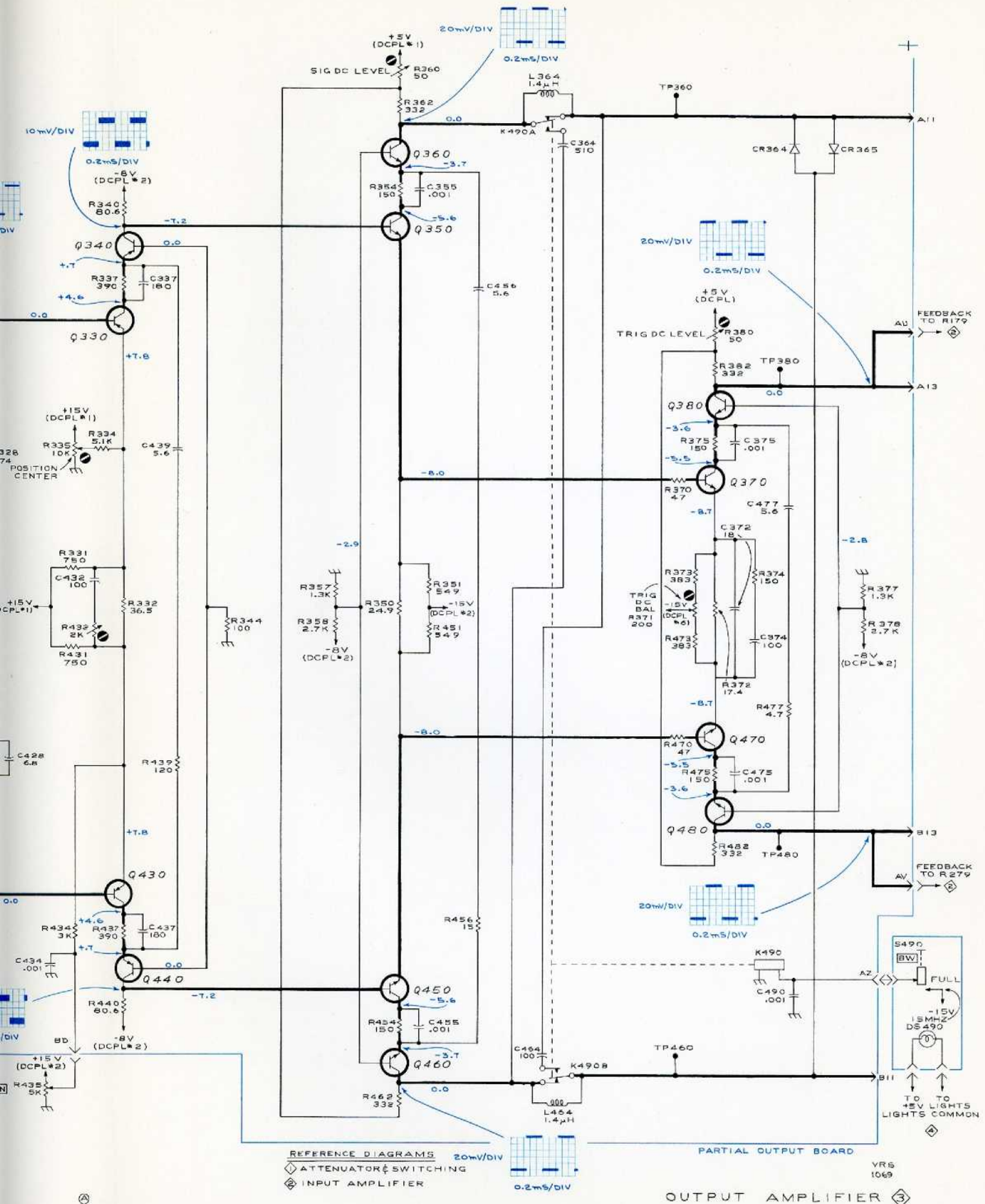
OUTPUT AMPLIFIER 3
