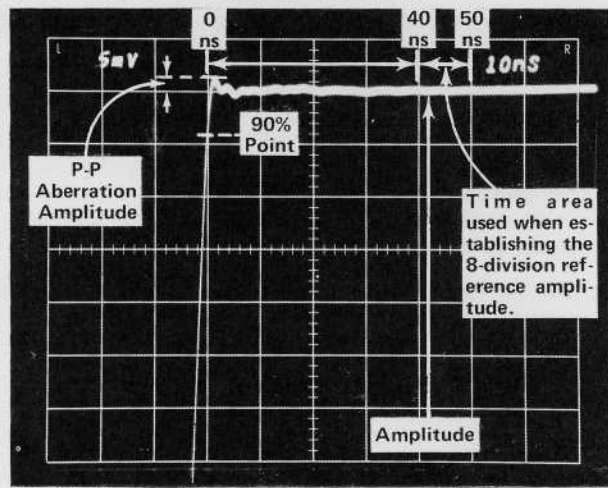
(C) Checking peak-to-peak aberration amplitude. Sweep rate is 10 ns/div. The 8-division reference amplitude was established when the top of the waveform was positioned to the top of the graticule. Then the waveform was positioned downward one division as a vertical position reference location for checking aberrations.
