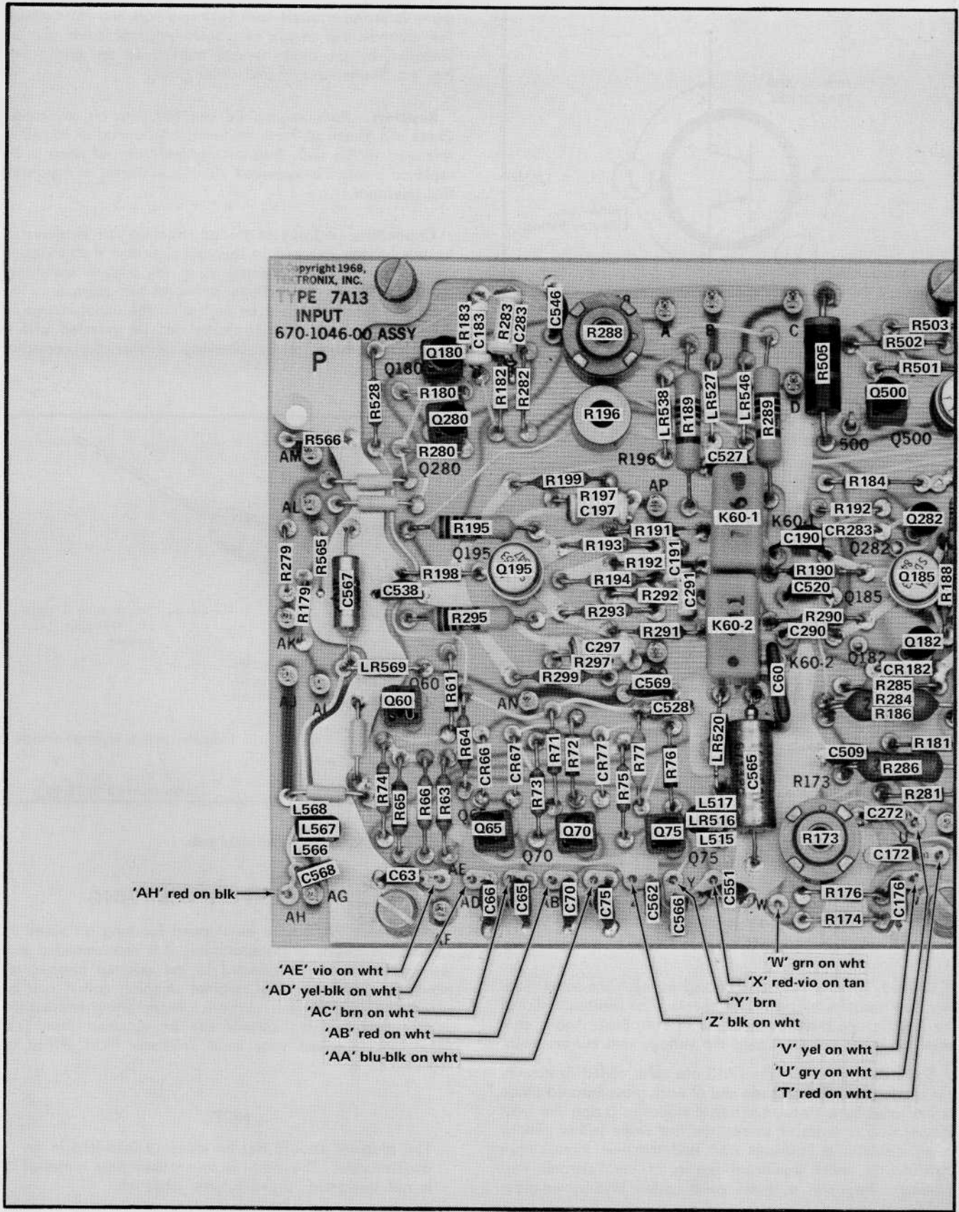
Fig. 4-6. Partial Input Amplifier board showing component locations and wire color code.
