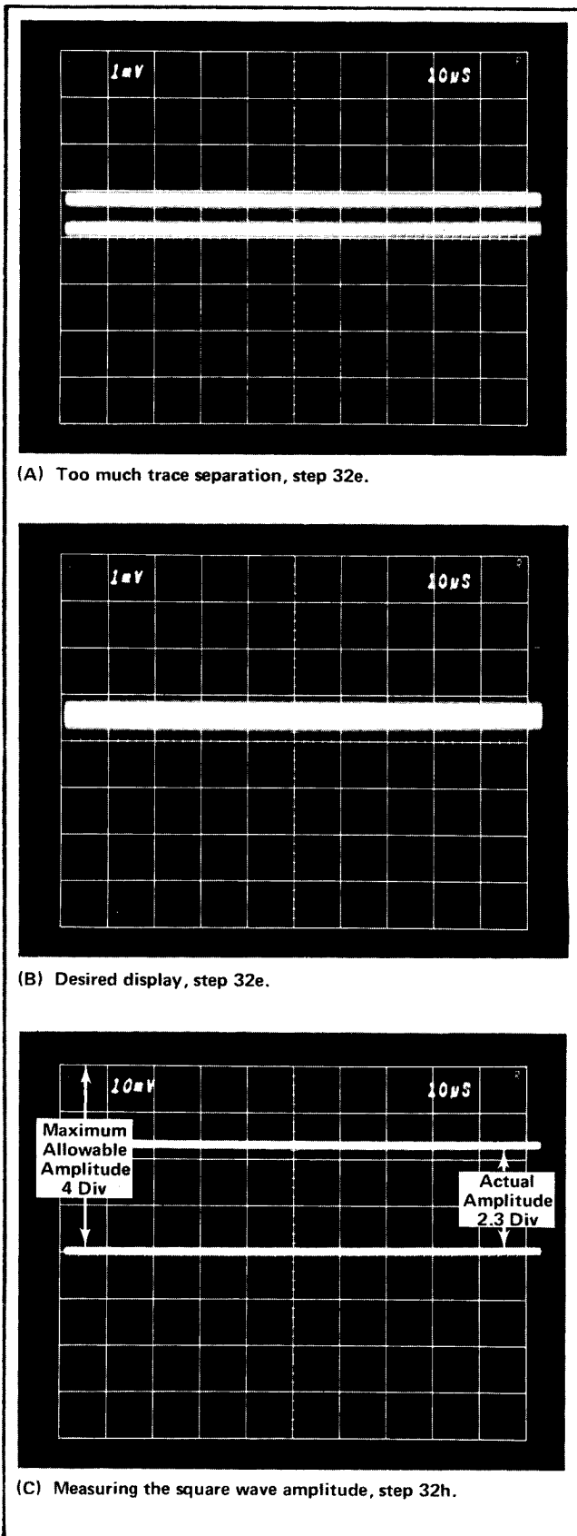
Fig. 5-29. Noise measurement displays. Sweep rate: 10 μs/div, free running.
