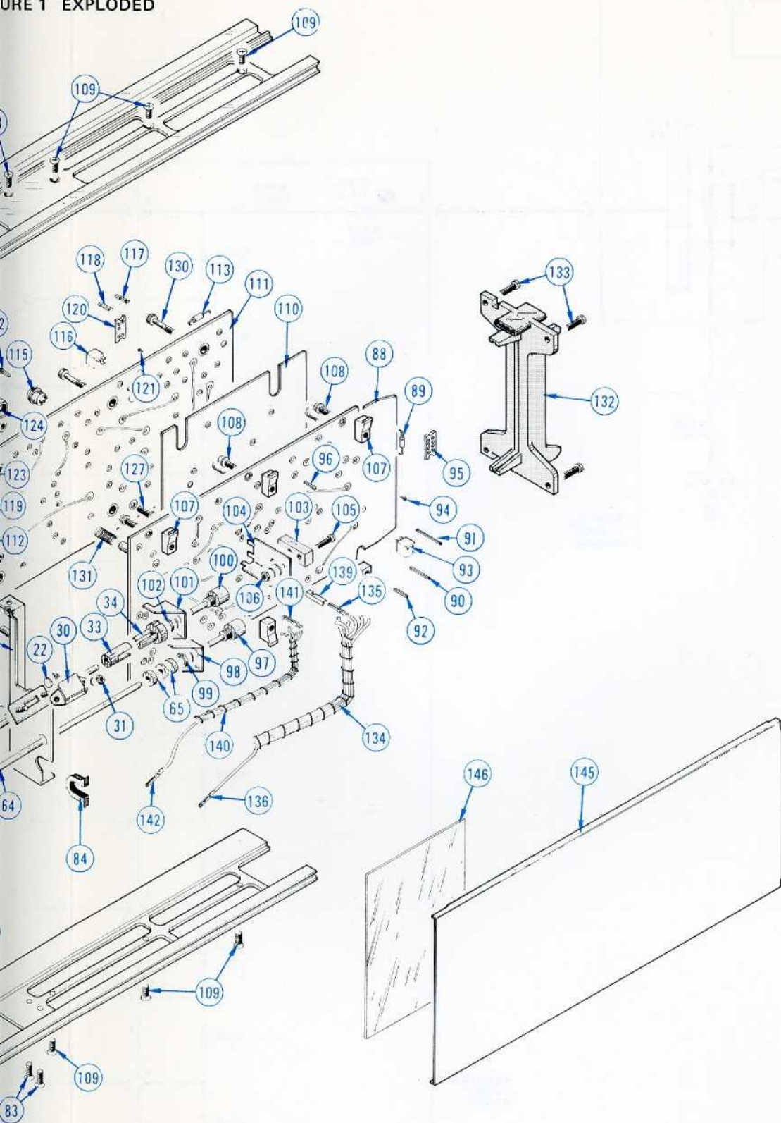
FIGURE 1 EXPLODED
