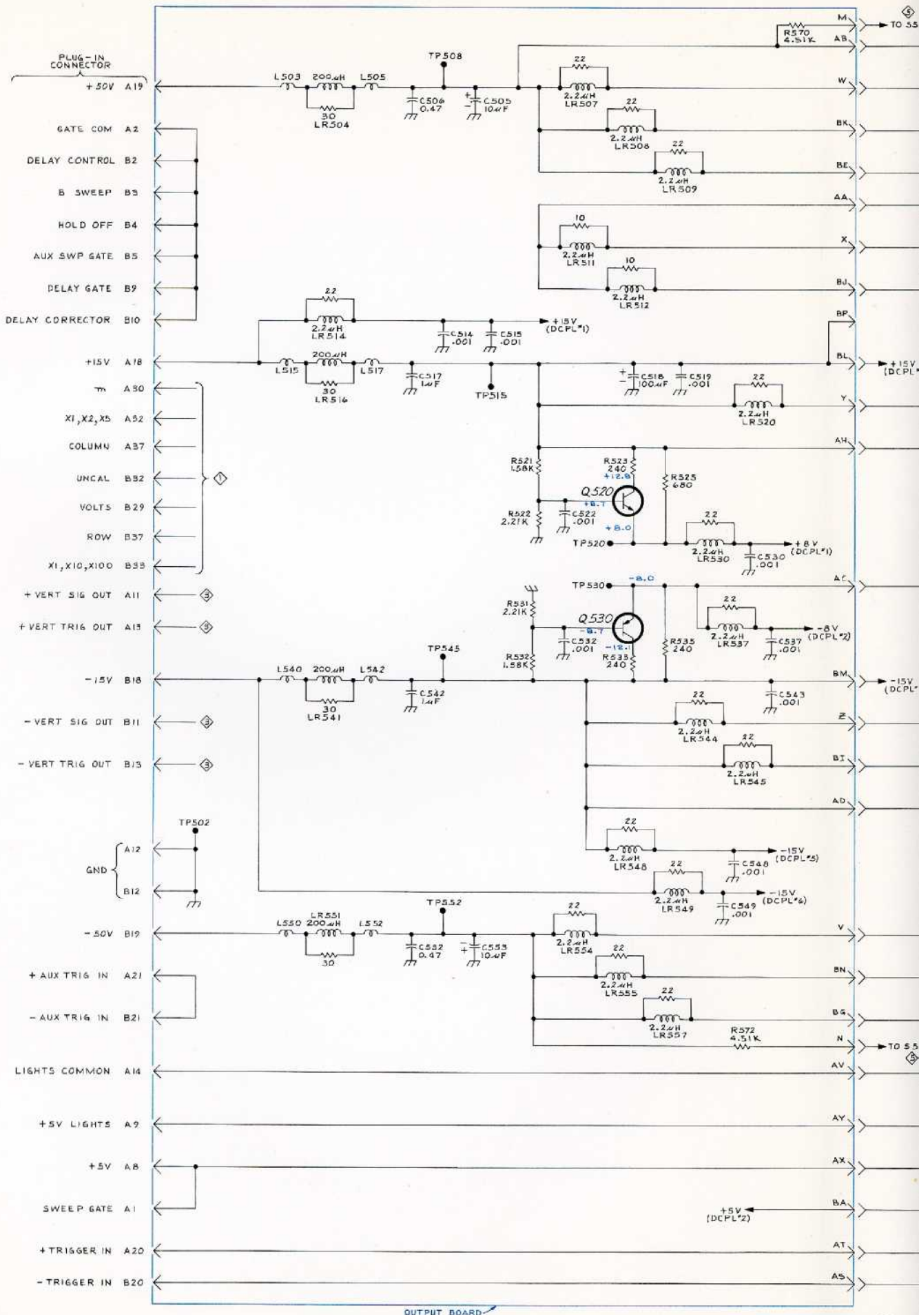
TYPE 7A13
