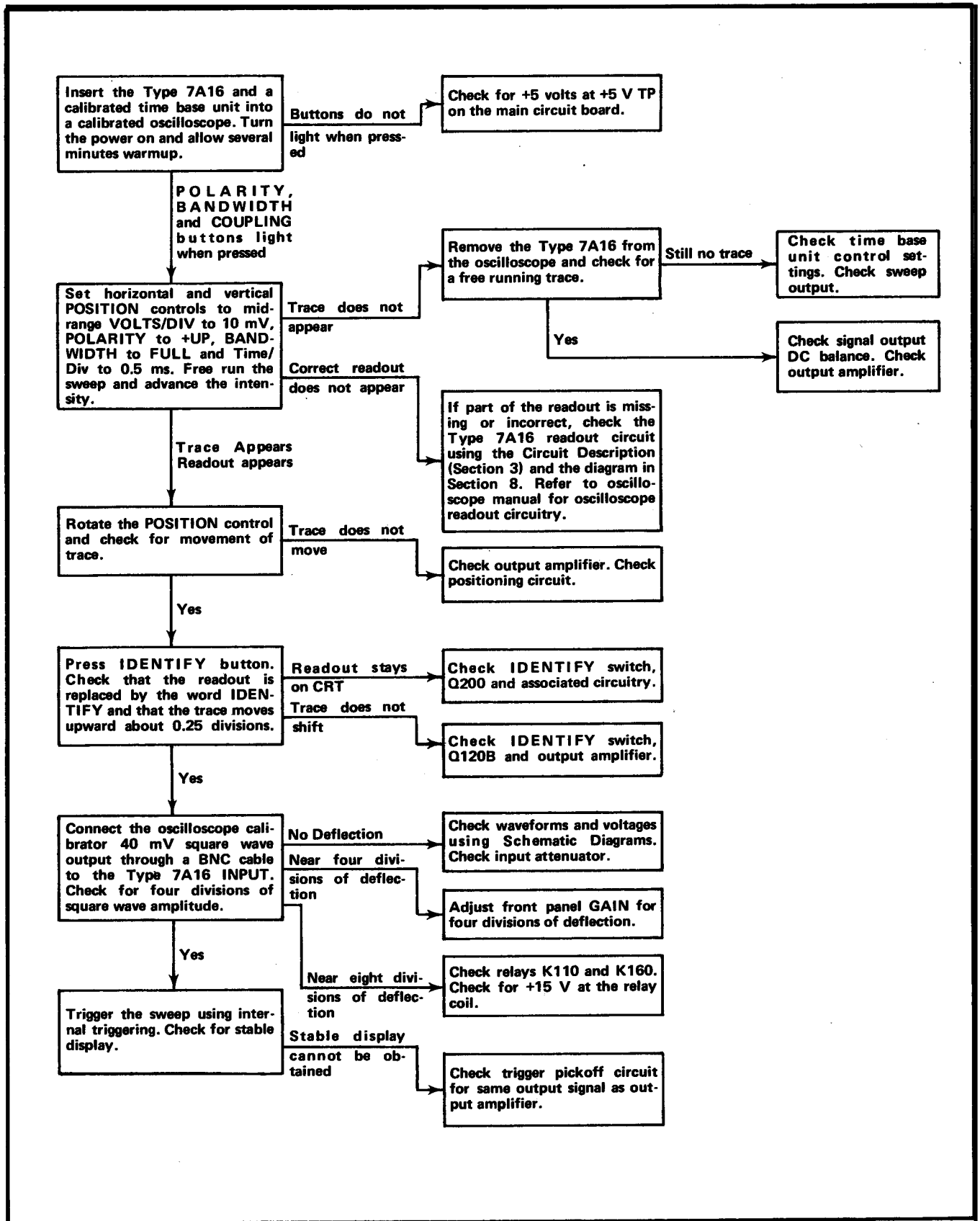
Fig. 4-2. Troubleshooting chart for Type 7A16.
