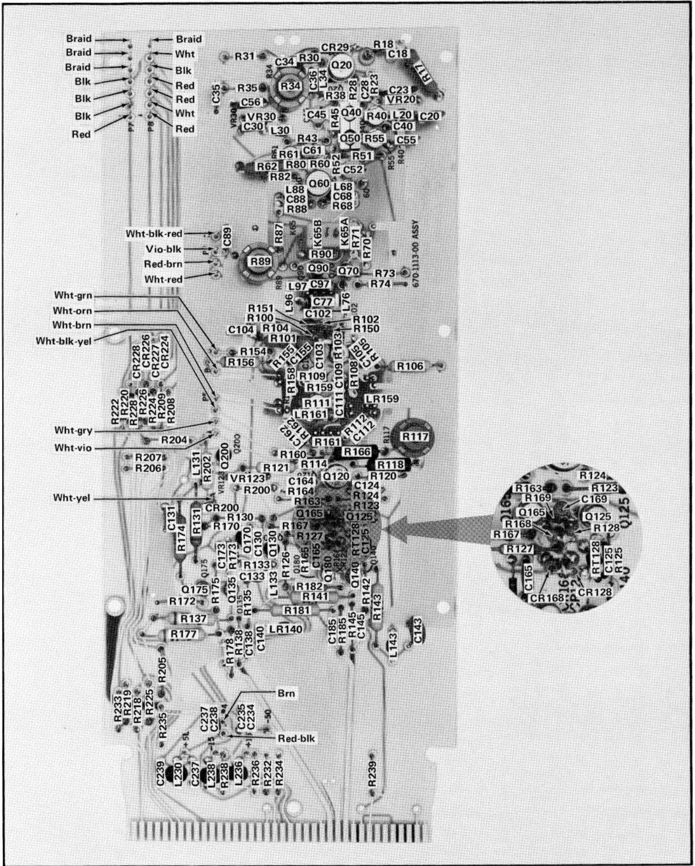
Fig. 4-5. Main amplifier circuit board (front).
