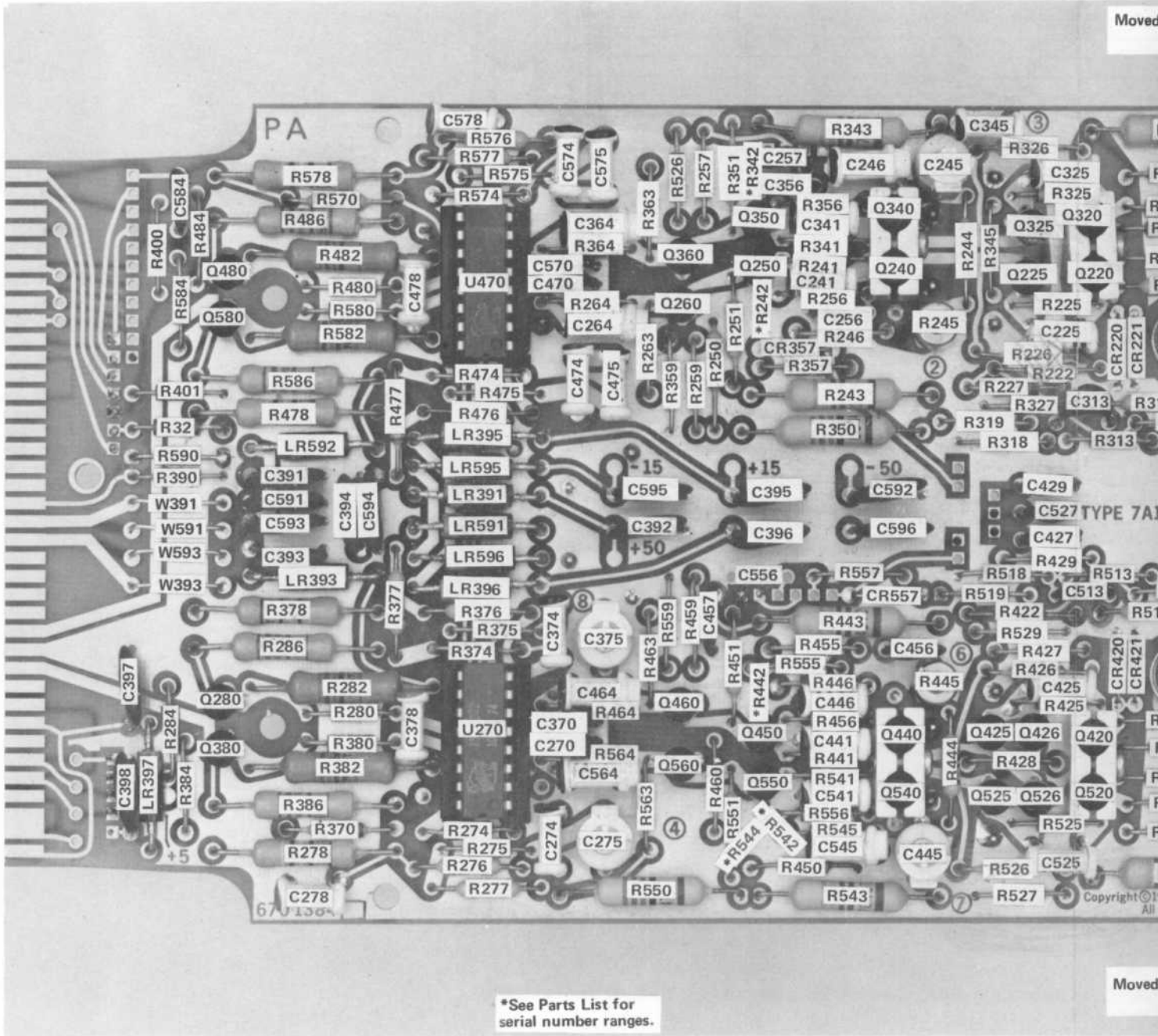
Fig. 7-1. A2 Amplifier Circuit Board Assembly (front view).
