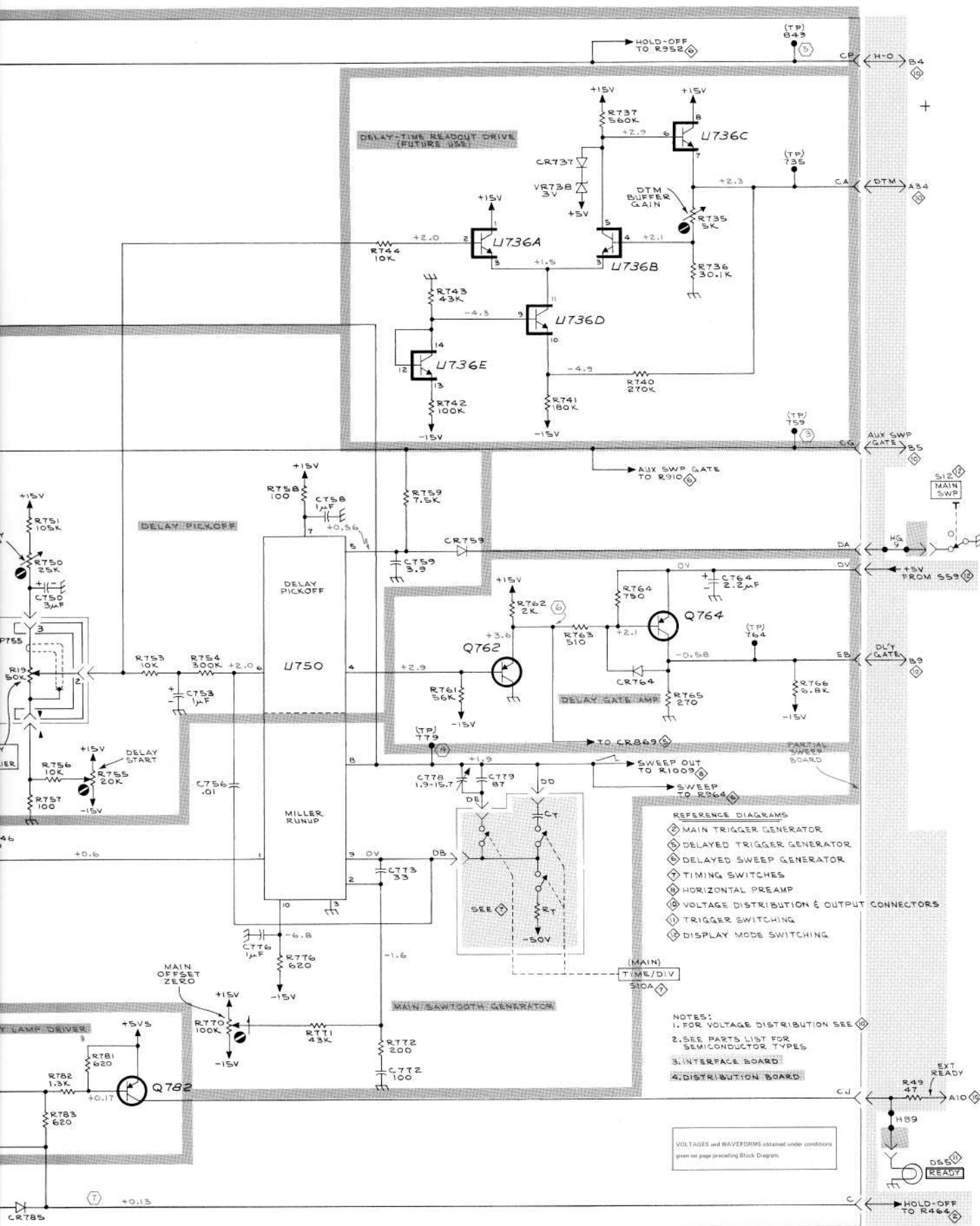
MAIN SWEEP GENERATOR
