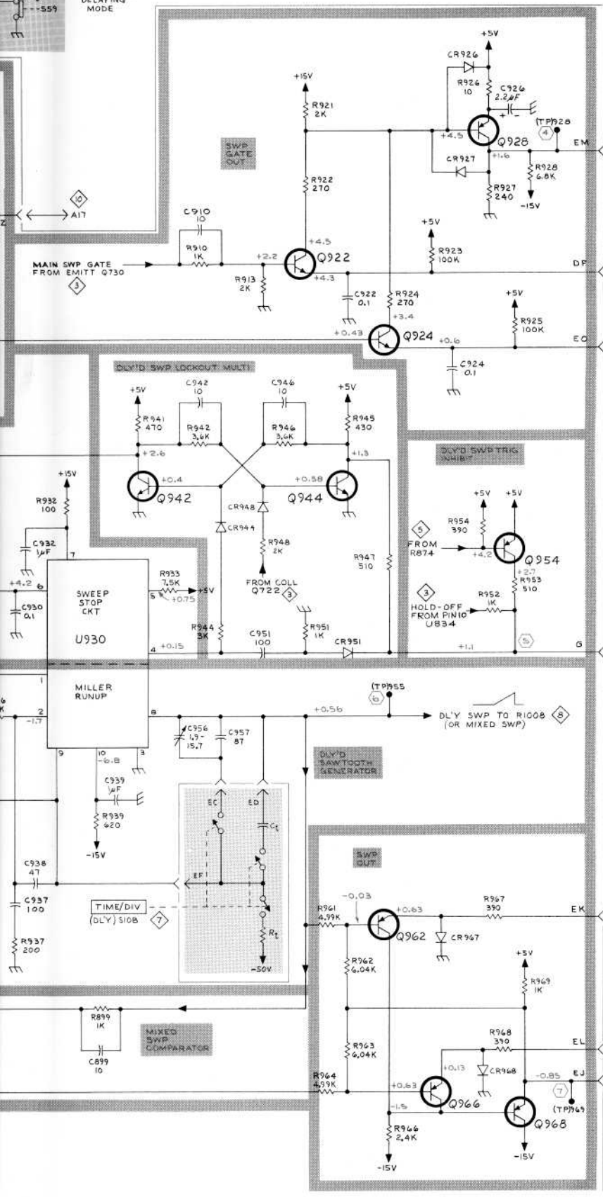
DELAYED SWEEP GENERATOR MGF 0670
