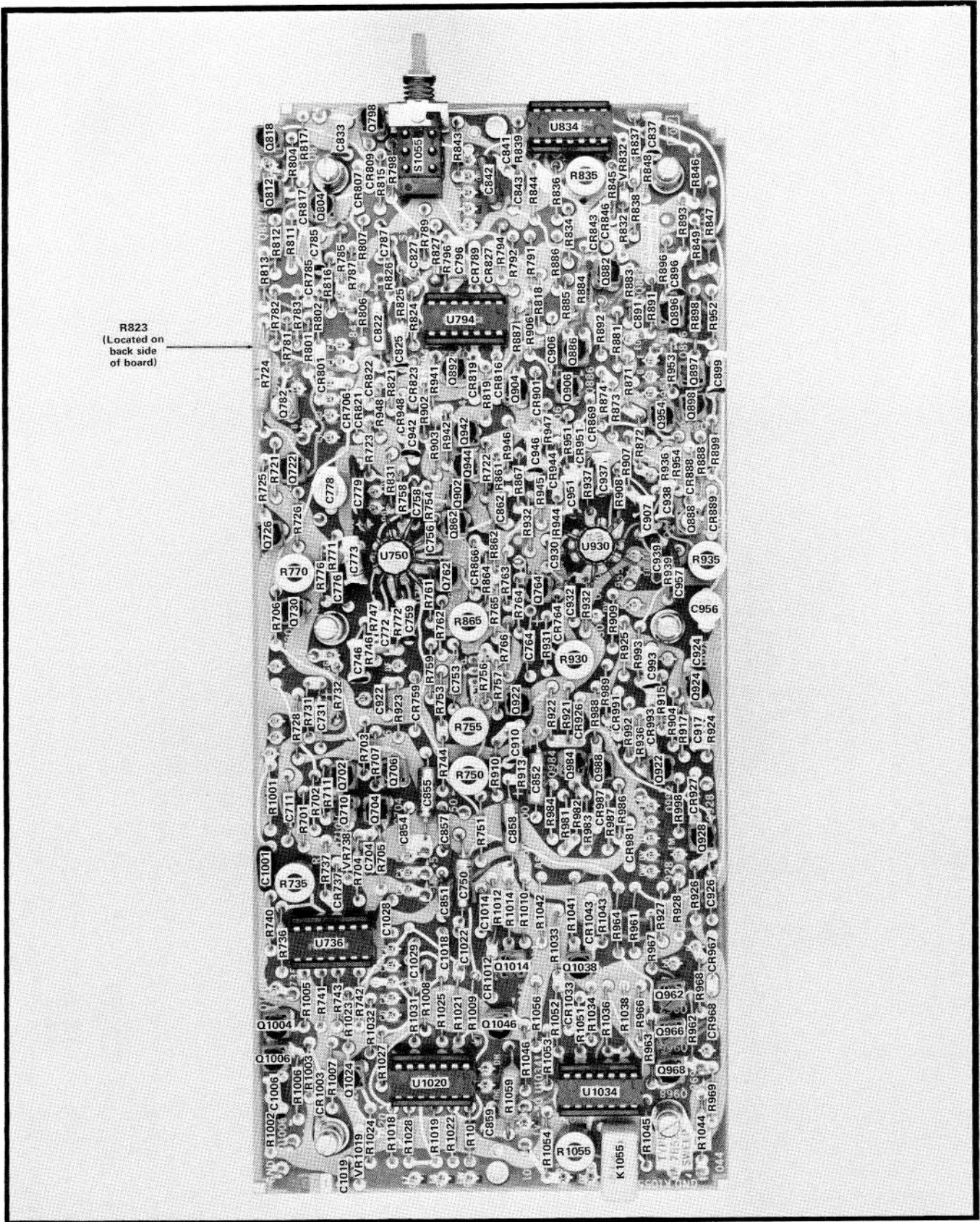
Fig. 4-4. 7B52 SWEEP BOARD showing component locations.
