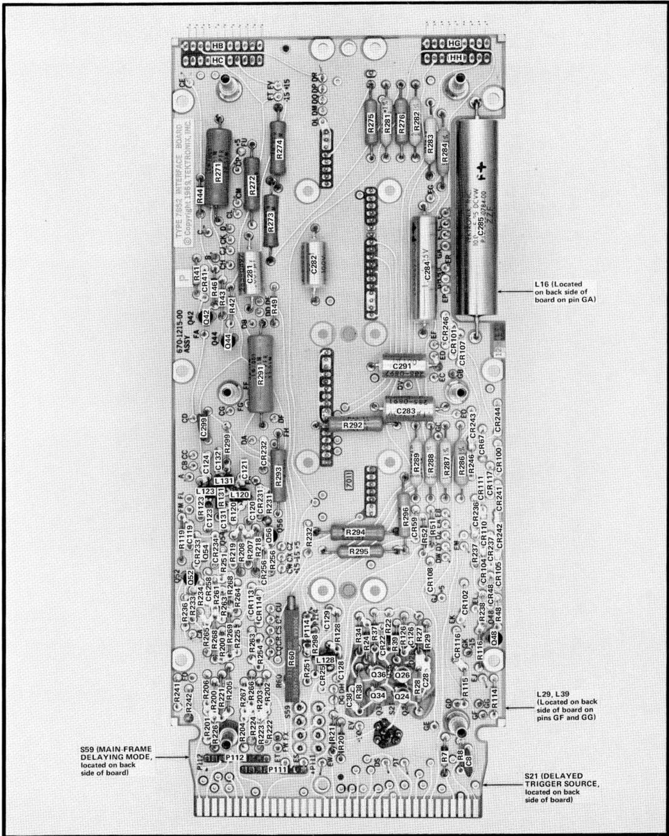
Fig. 4-3. 7B52 INTERFACE BOARD showing component locations.
