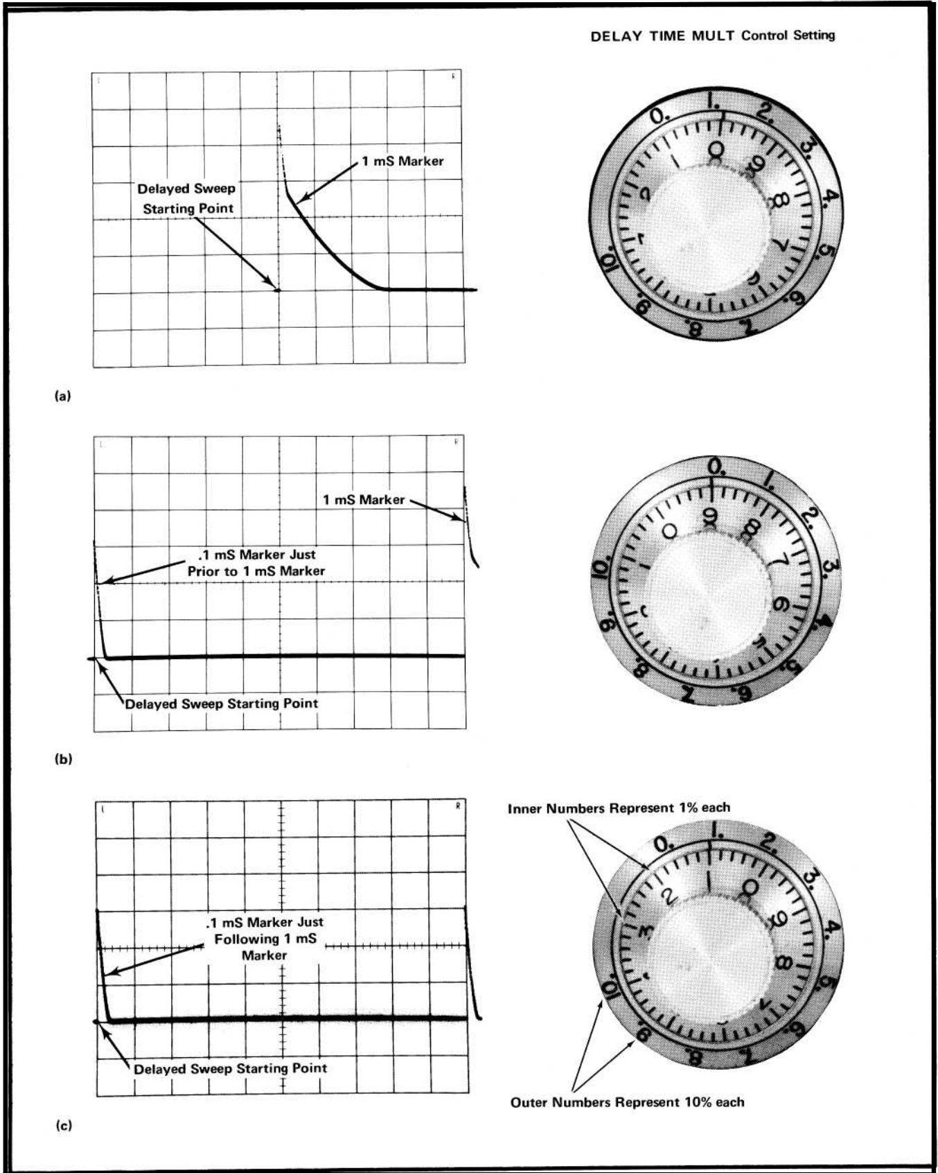
Fig. 5-5. Typical CRT display obtained in DLY'D SWP (a) delayed sweep adjusted (b) delayed sweep 1% slow and (c) delayed sweep 1% fast.
