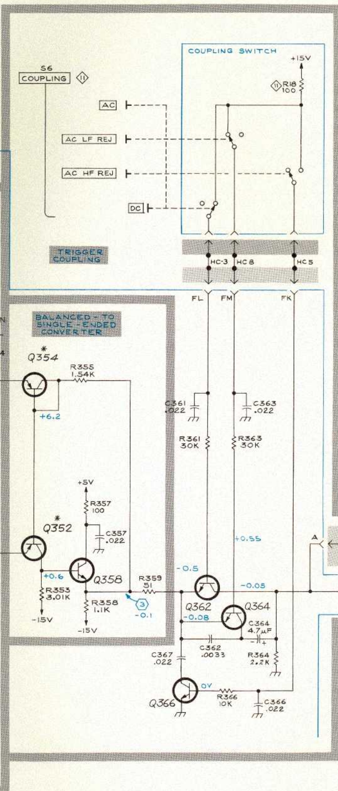
BC 0670 MAIN TRIGGER PREAMP 1
