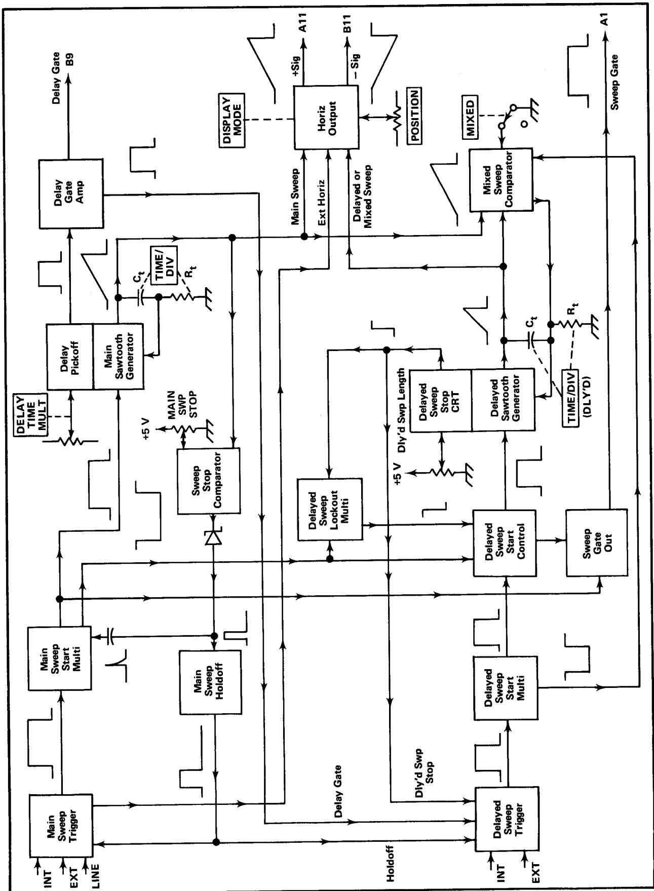
Fig. 3-1. 7B52 Simplified Block Diagram.
