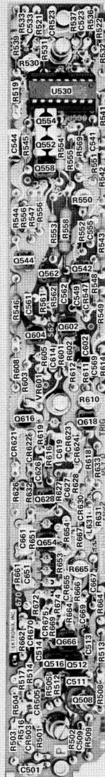
DLY'D TRIG BOARD
