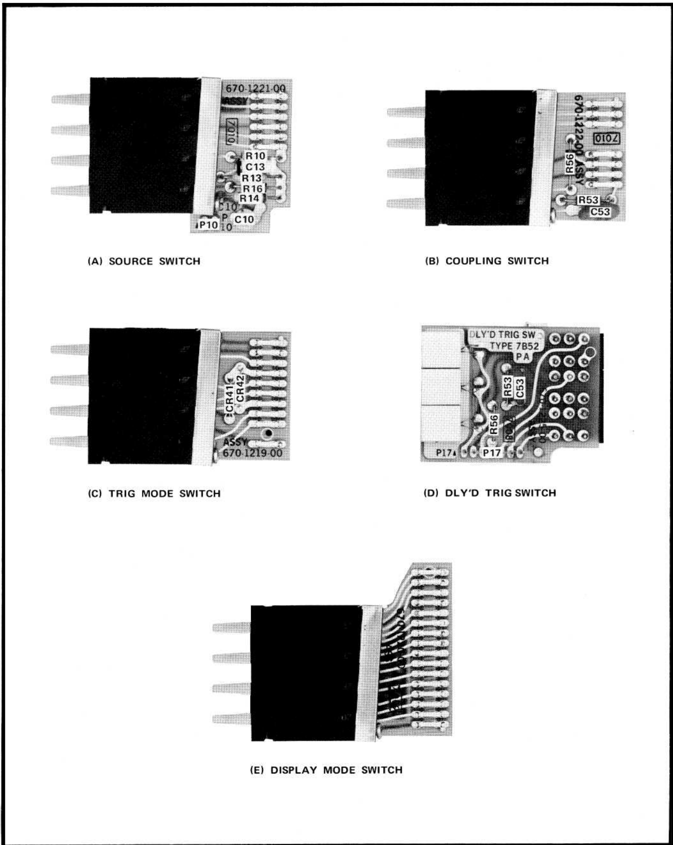
Fig. 4-7. 7B52 SOURCE SWITCH (a), COUPLING SWITCH (b), TRIG MODE SWITCH (c), DLY'D TRIG SWITCH (d), and DISPLAY MODE SWITCH (e) showing component locations. (There are no components on the DISPLAY MODE SWITCH, see (e).
