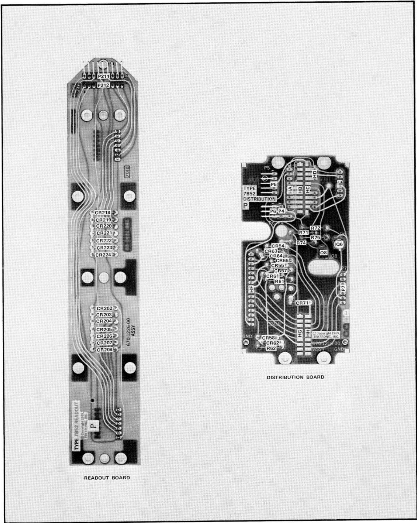
Fig. 4-6. 7B52 READOUT BOARD (left) and DISTRIBUTION BOARD (right) showing component locations.
