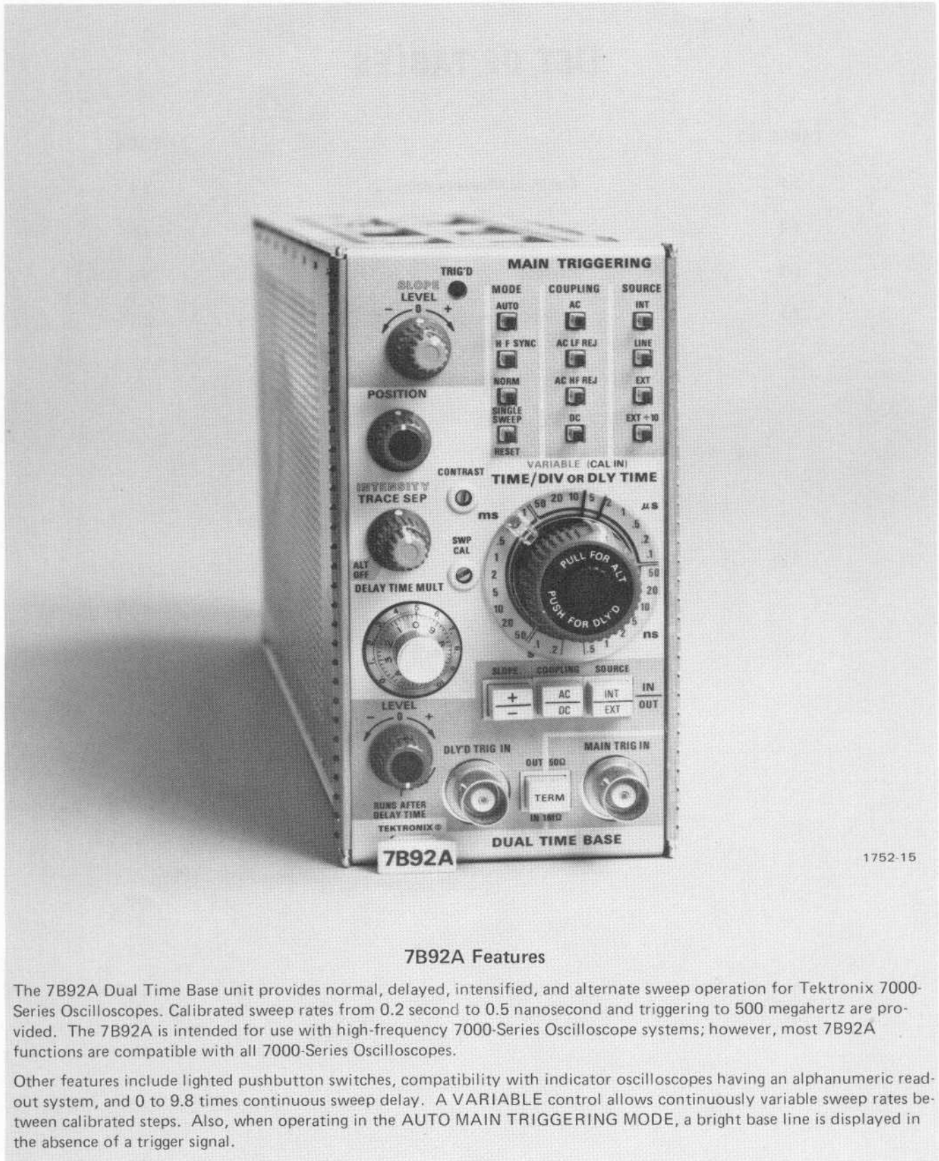
Fig. 1-1. 7B92A Dual Time Base.
