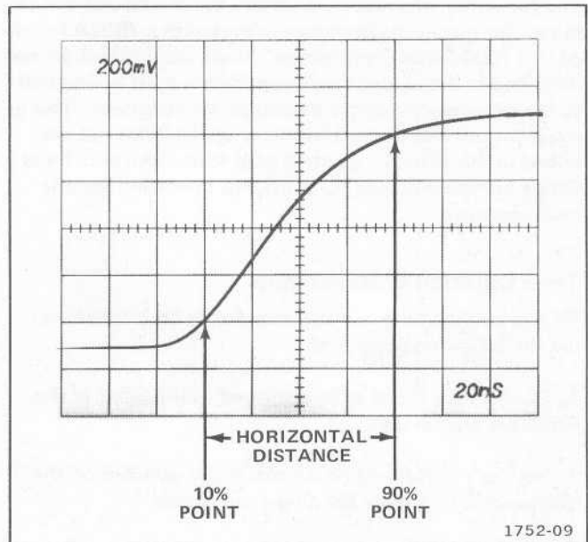
Fig. 2-8. Measuring risetime.
