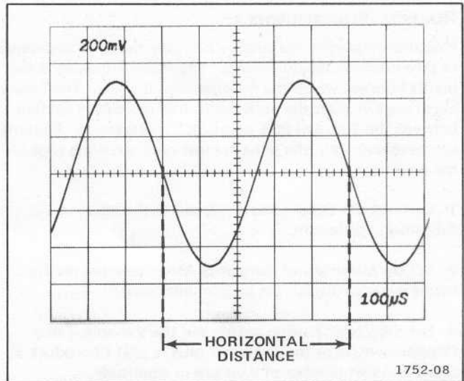
Fig. 2-7. Measuring the time duration between points on a waveform.
