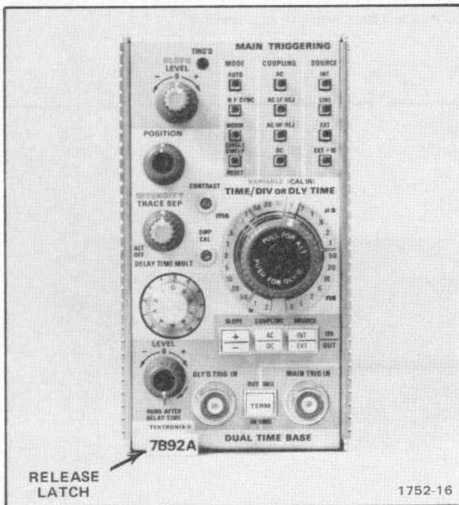
Fig. 2-2. Location of release latch.
