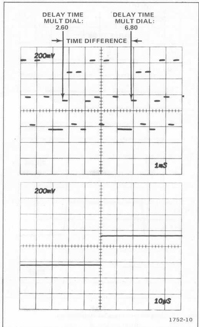
Fig. 2-9. Measuring time difference using delayed sweep.
