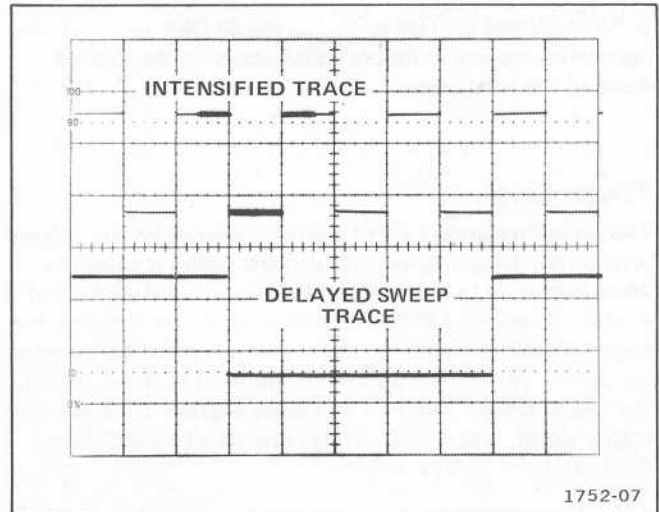
Fig. 2-6. Typical alternate sweep display.
