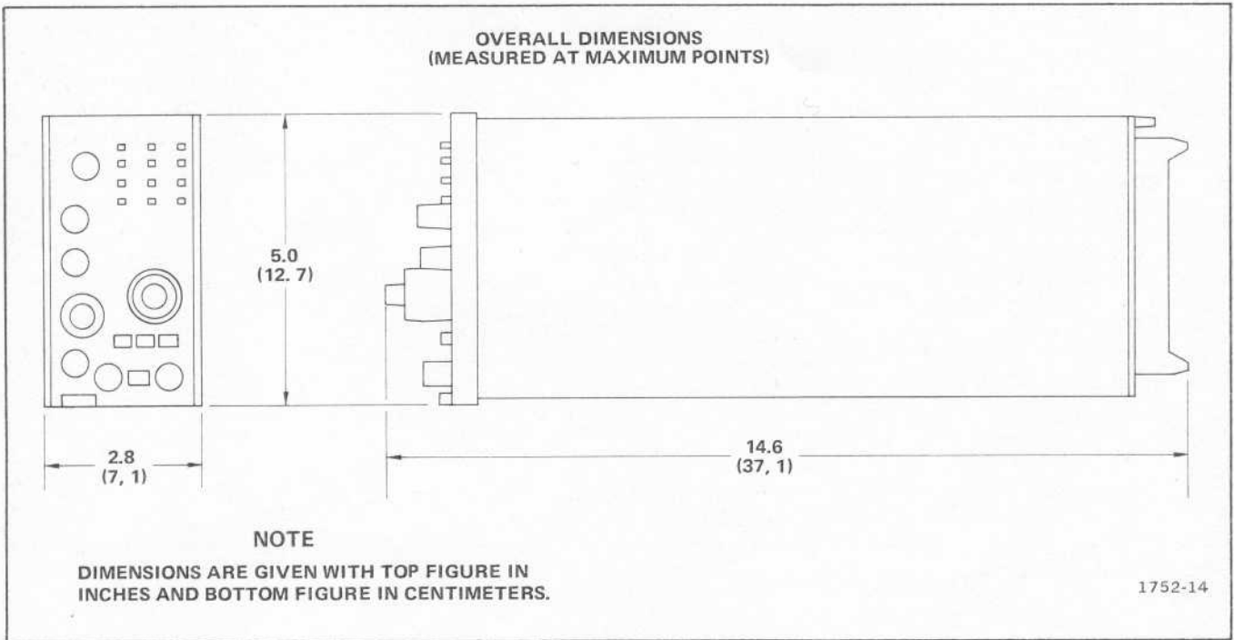
Fig. 1-2. Dimensional drawing.
