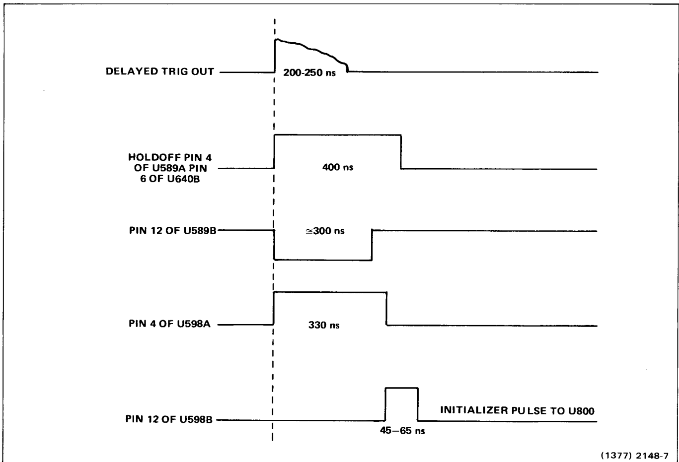
Figure 3-6. 7D10 Reset function timing diagram.
