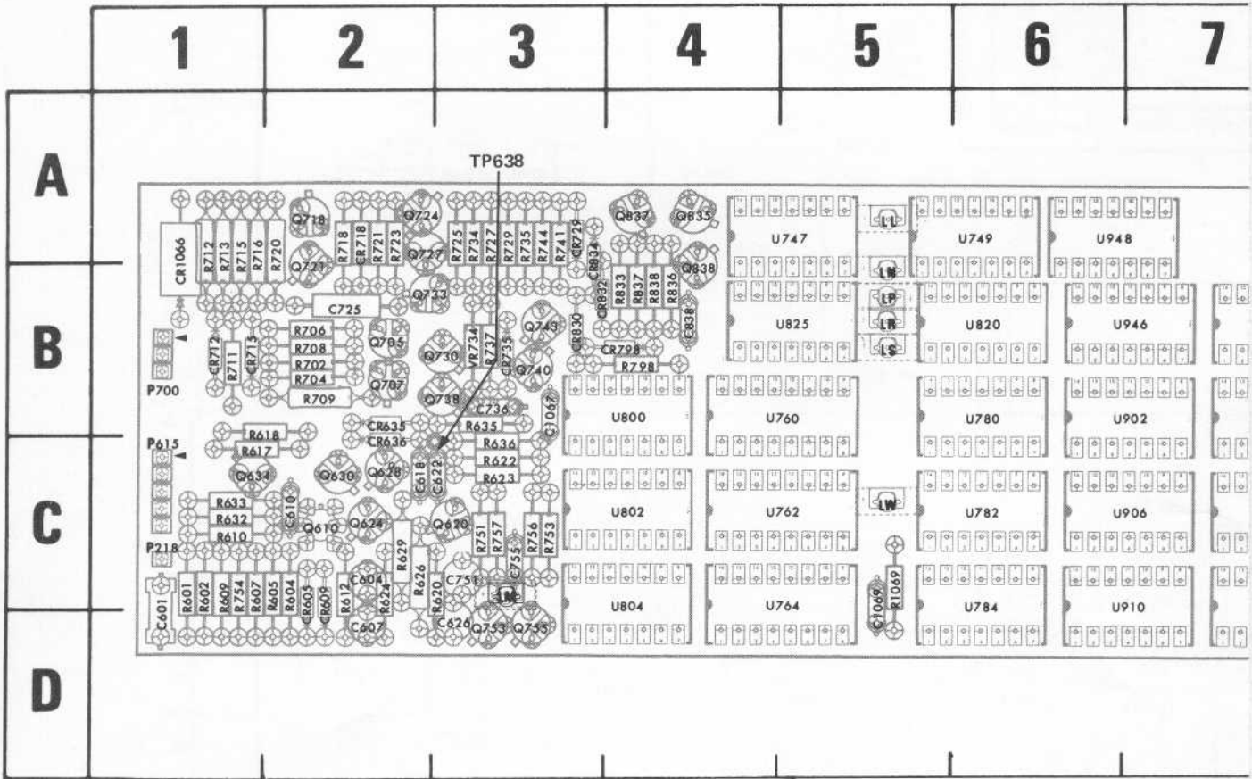
Figure 8-6. A7—Logic circuit board.
