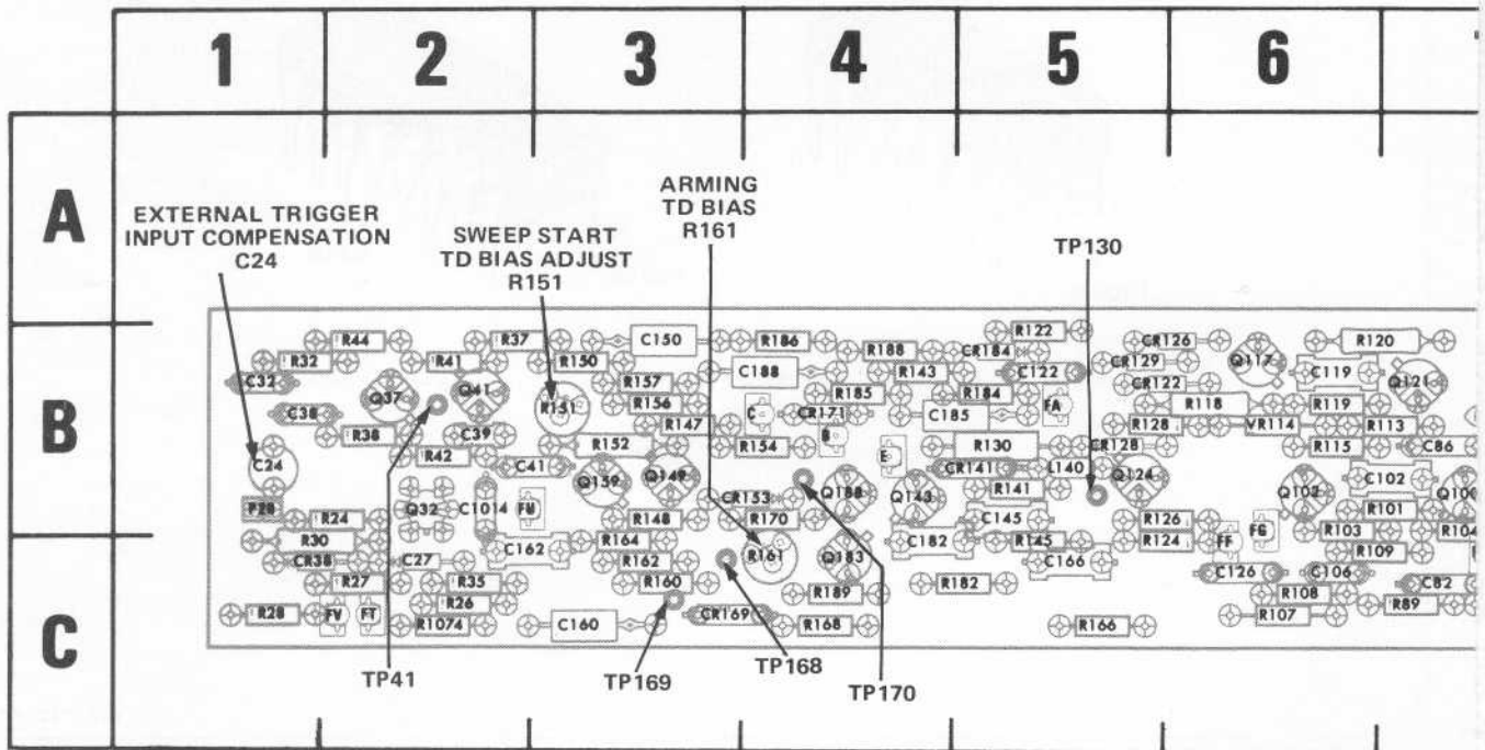
Figure 8-4. A3—Trigger circuit board
