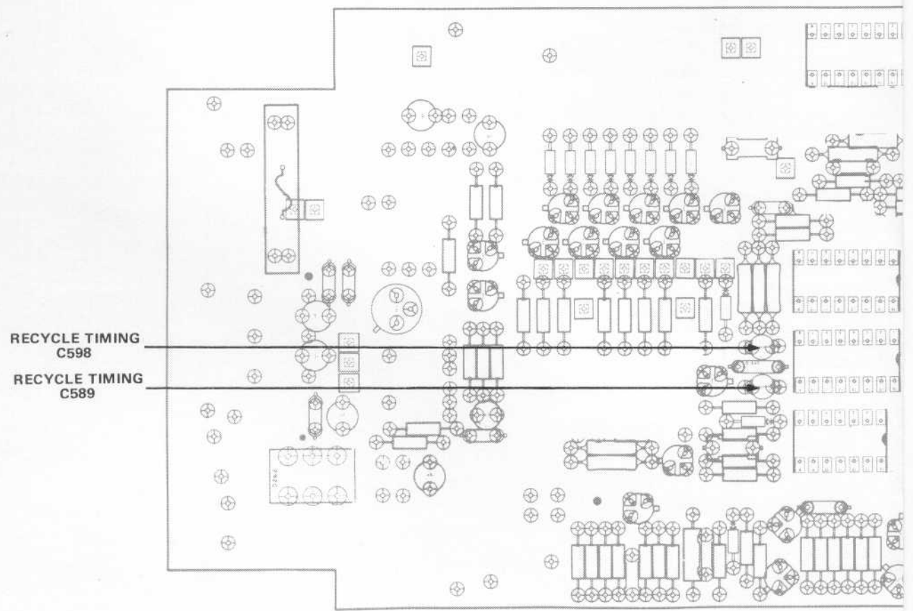
Figure 8-11. Interface circuit
