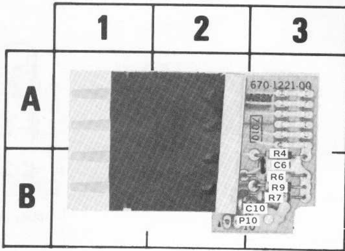
Figure 8-2. A1—Source switch.
