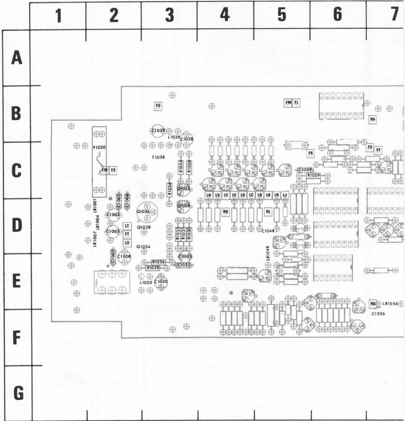
Figure 8-7. A4—Partial Interface circuit
