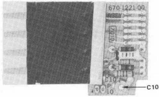
Figure 8-10. Source switch adjustment locations.
