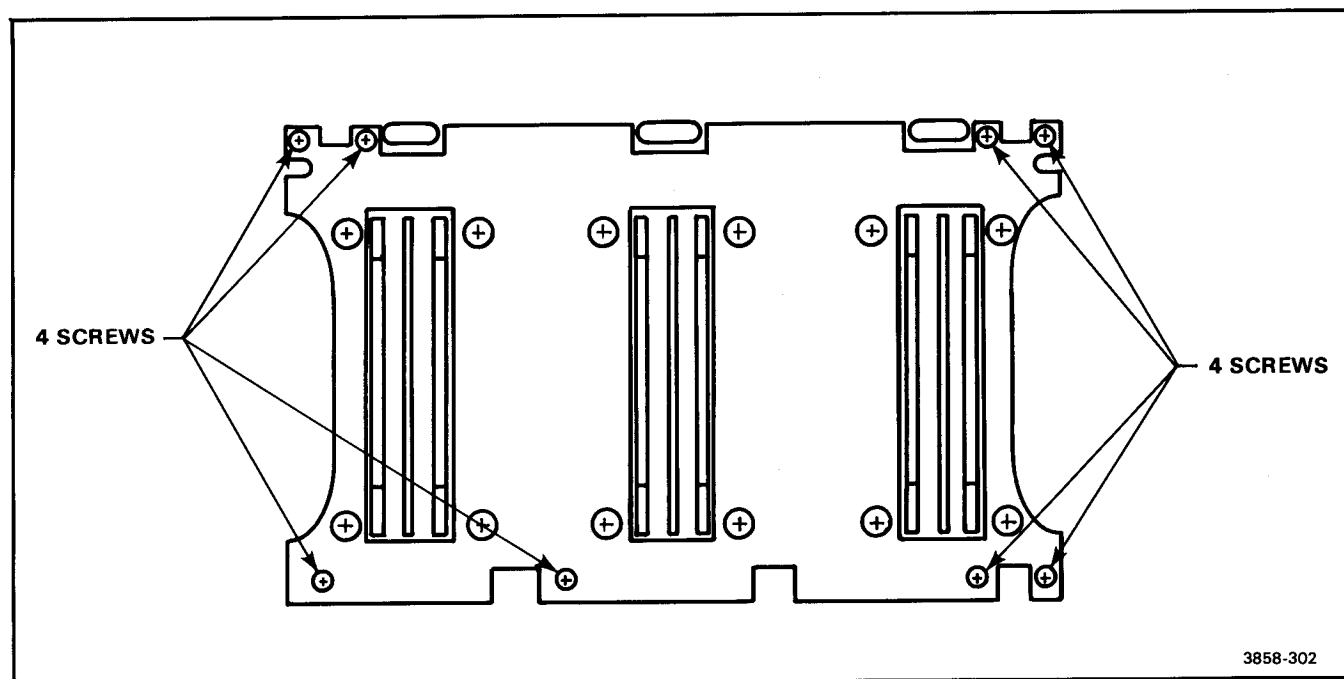
Figure 3-6. Back-panel removal.
