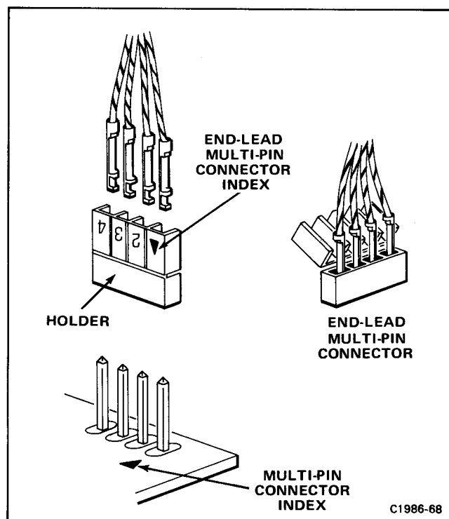
Figure 3-3. Orientation of multi-pin connectors.
