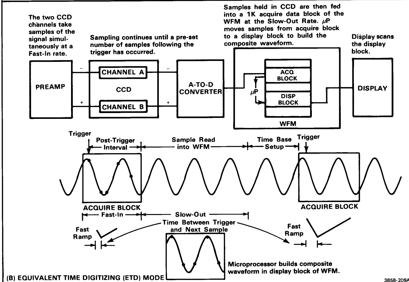
Figure 2-4. Fast-In, Slow-Out Time Base Modes: (A) Extended Real-Time Digitizing (ERD) Mode; (B) Equivalent Time Digitizing (ETD) Mode.
