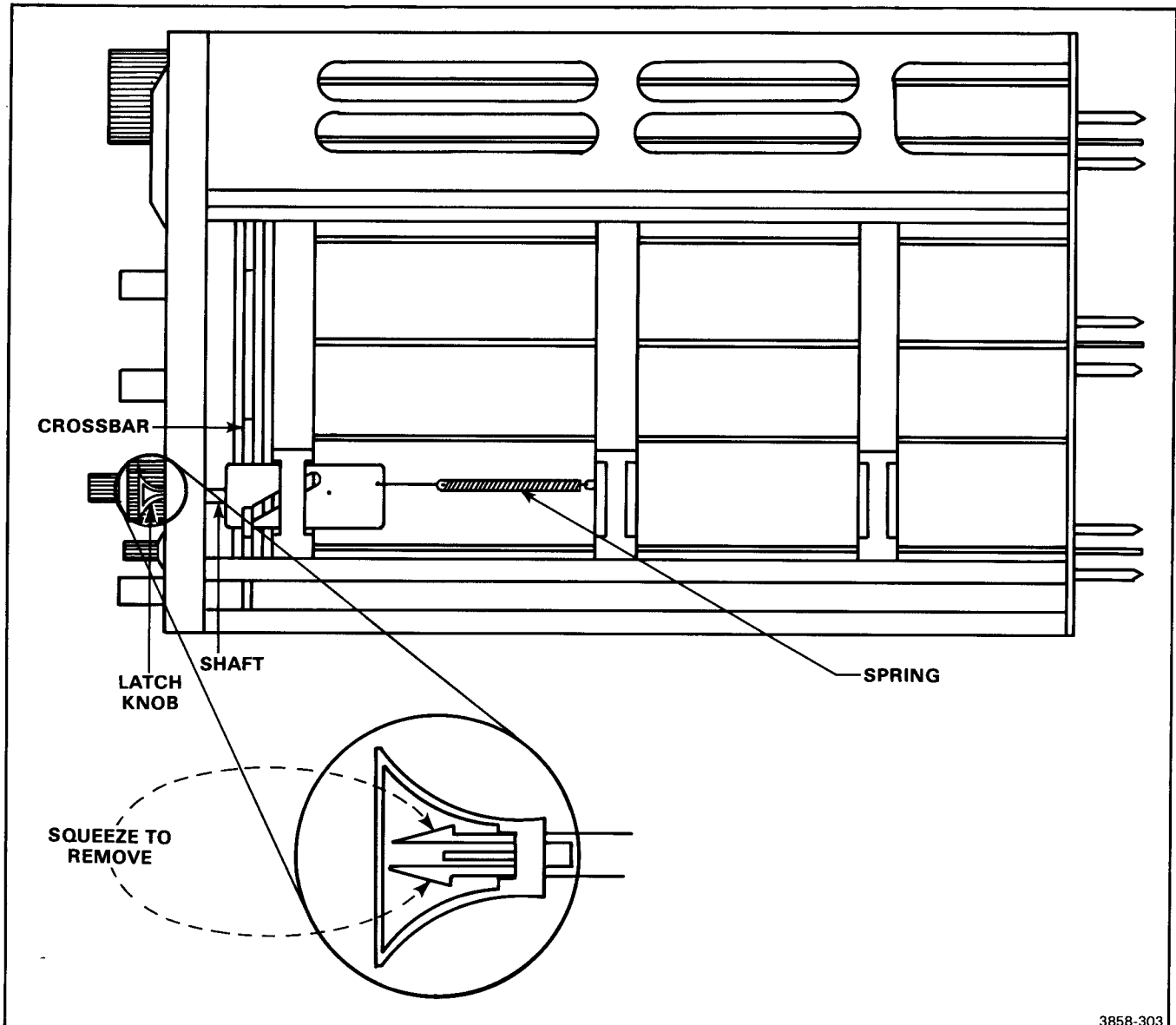
Figure 3-7. Latch assembly.
