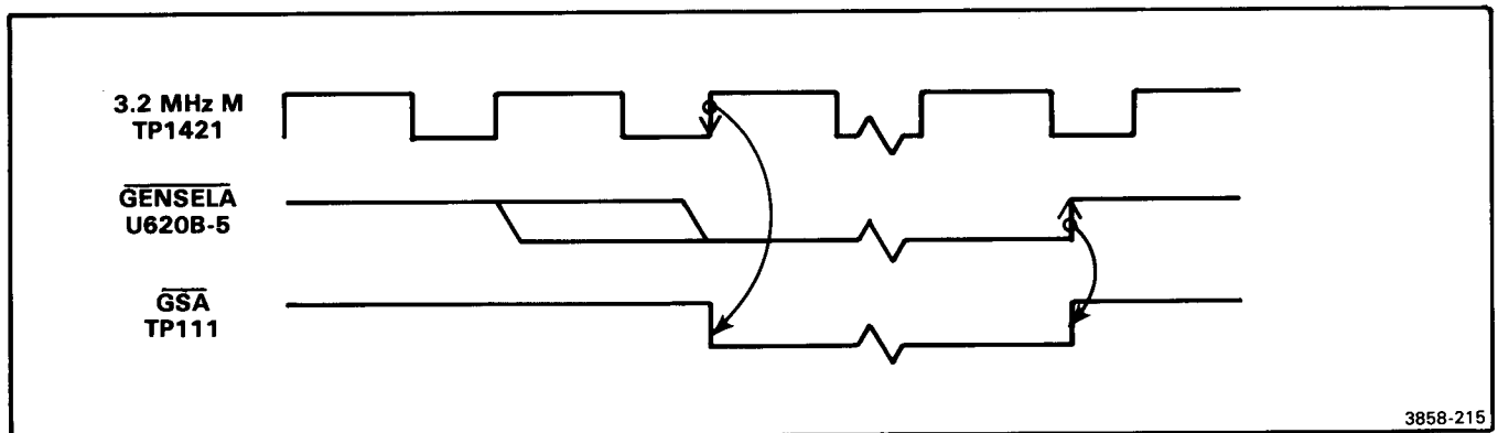
Figure 2-17. \overline{\text{GENSELA}} and \overline{\text{GSA}} signal synchronization.
