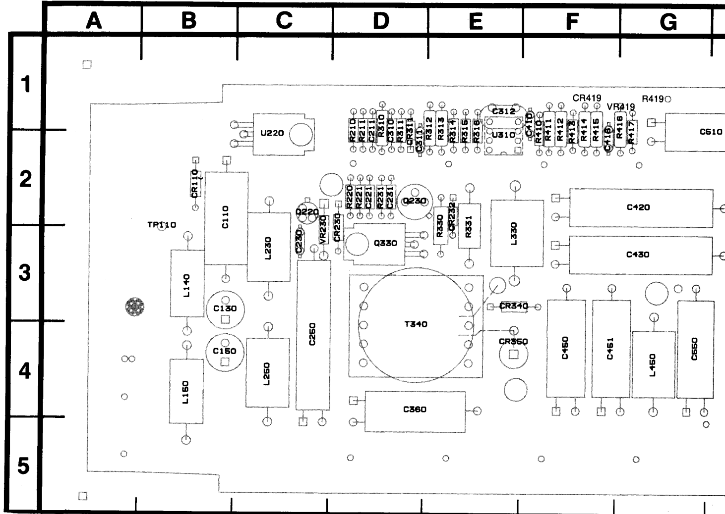
Figure 7-9. A7—Power Supply circuit board assembly
