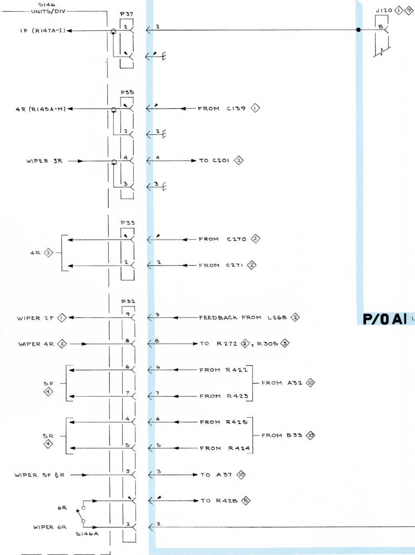
+ 7512 SAMPLING UNIT
