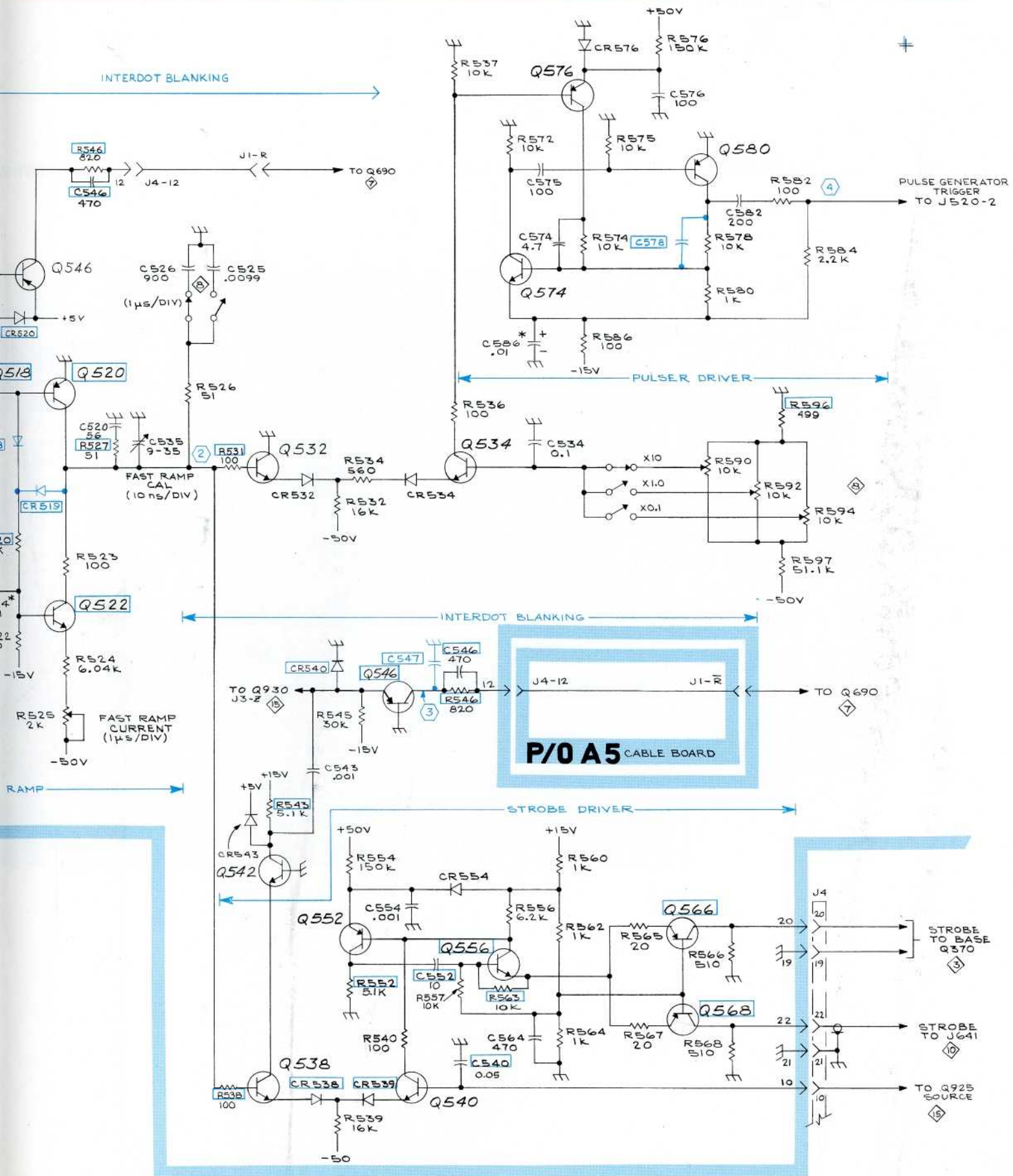
TRIGGER, FAST RAMP, PULSER, STROBE DRIVERS & COMPARATORS
