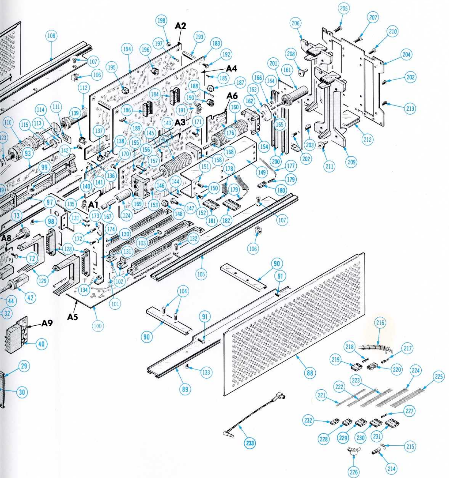
7S12 TDR SAMPLING UNIT (SN B020000-up)
