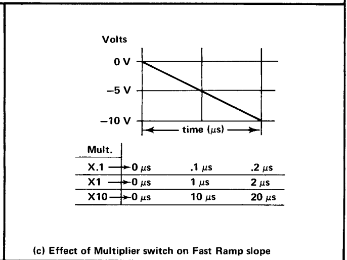
Fig. 3-4. Partial Horizontal circuit block diagram and Fast Ramp voltage versus time waveforms.
