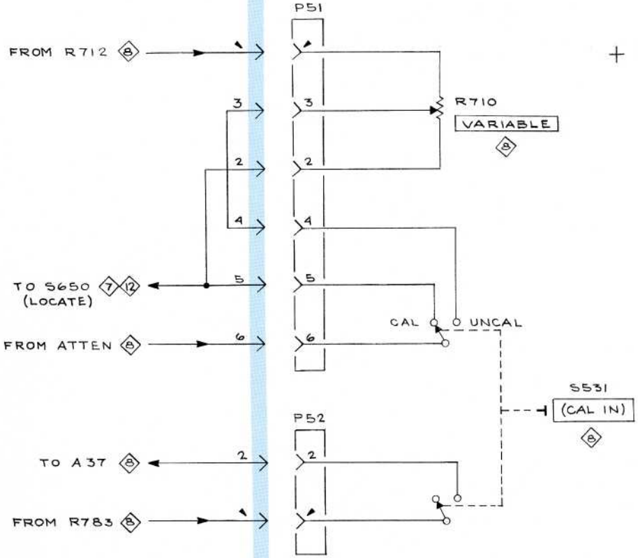
P/O A3 RIGHT INTERFACE BOARD
