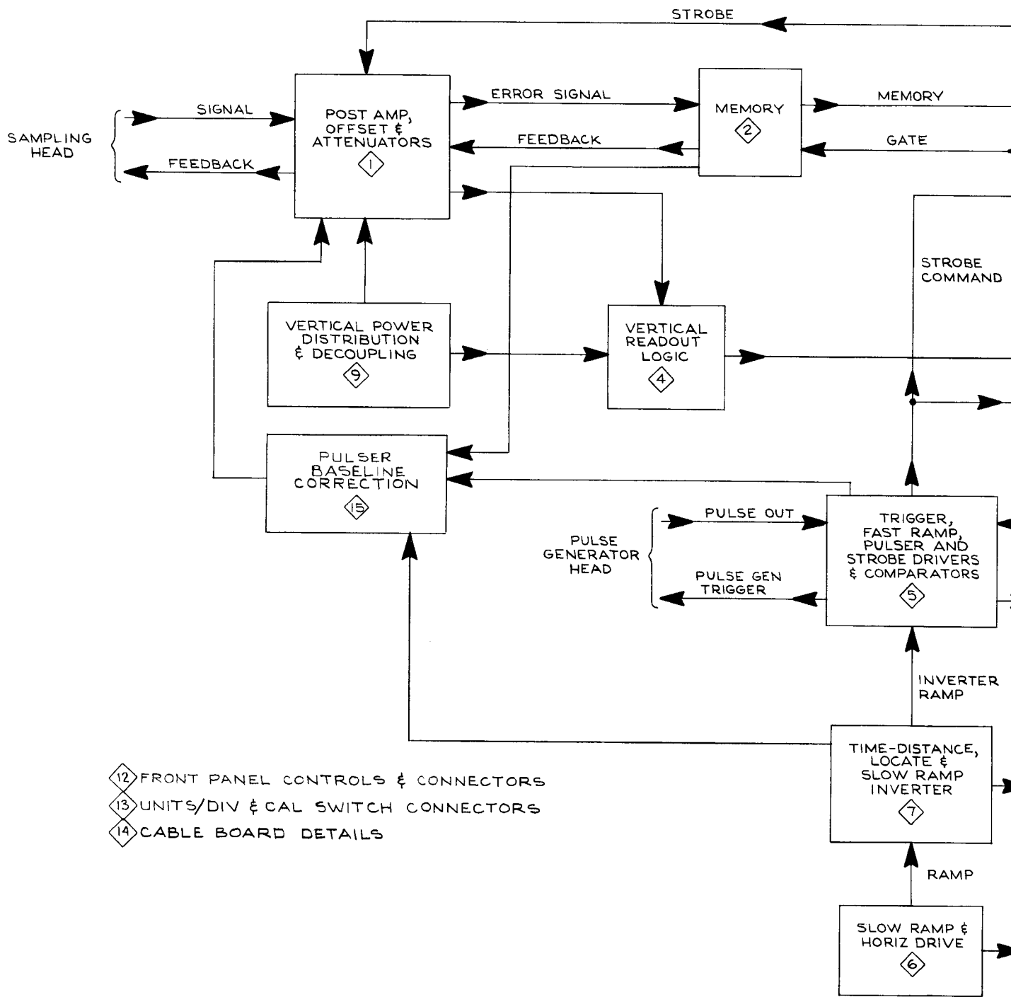
7S12 SAMPLING PLUG-IN
