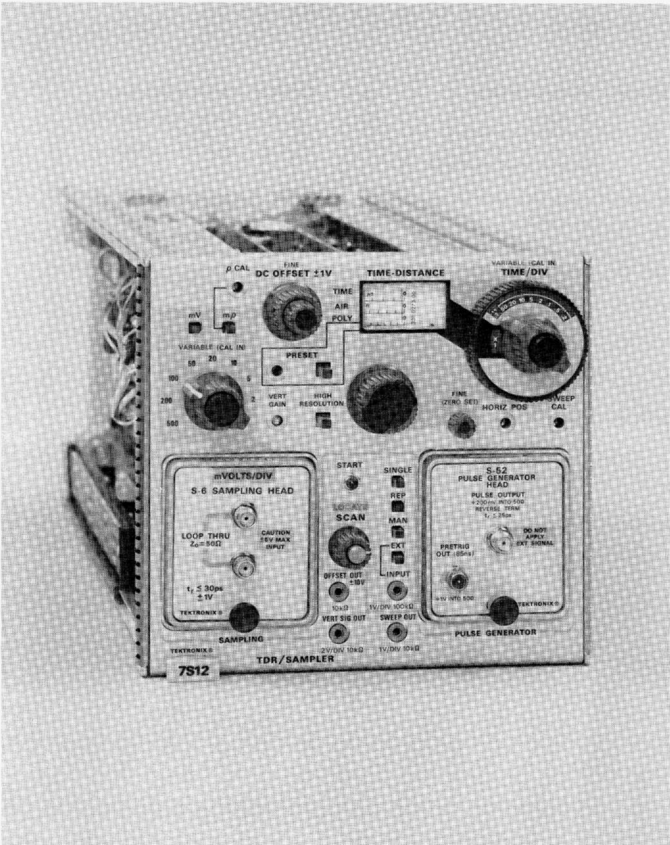
Fig. 1-1. 7S12 TDR/Sampler unit.
