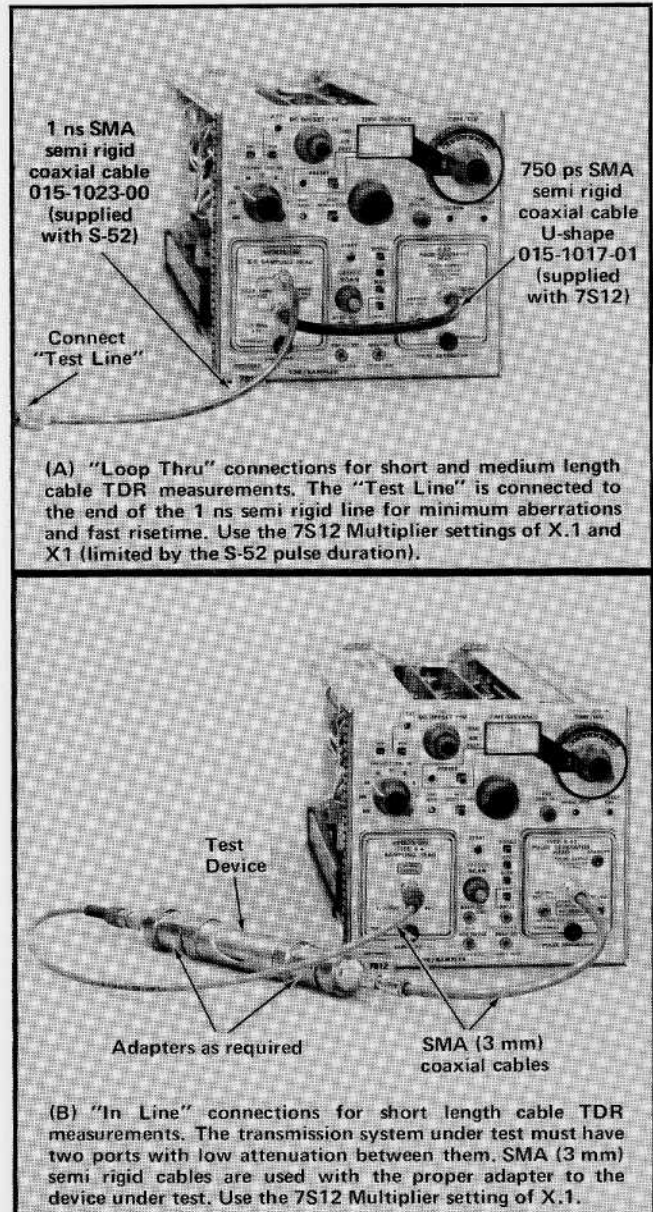
Fig. 2-10. Application connections for "Loop Thru", and "In Line" TDR.
