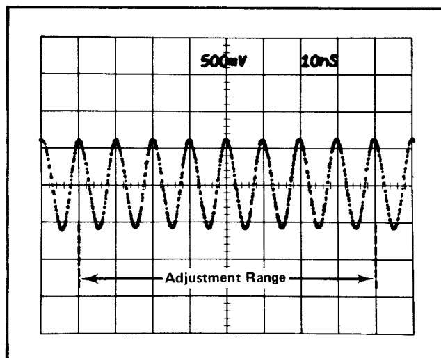
Fig. 5-16. Correct 10 ns/div adjustment waveform.
