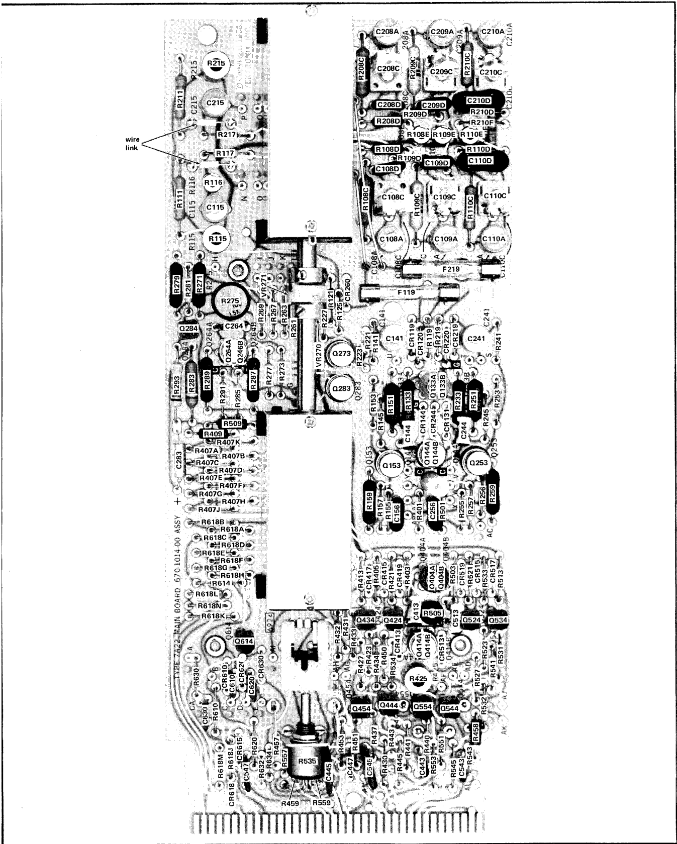
Fig. 4-6. Main circuit board (components)
