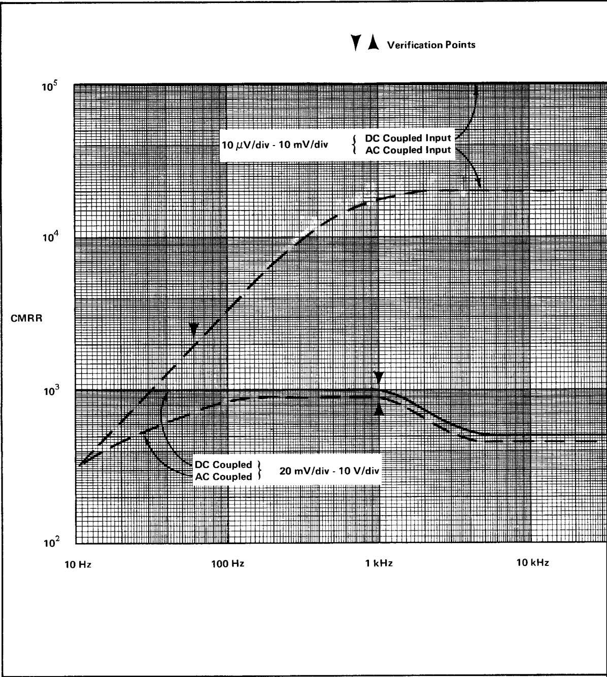
Fig. 1-2. CMRR vs. Frequency for signals not exceeding Common Mode Signal Range.
