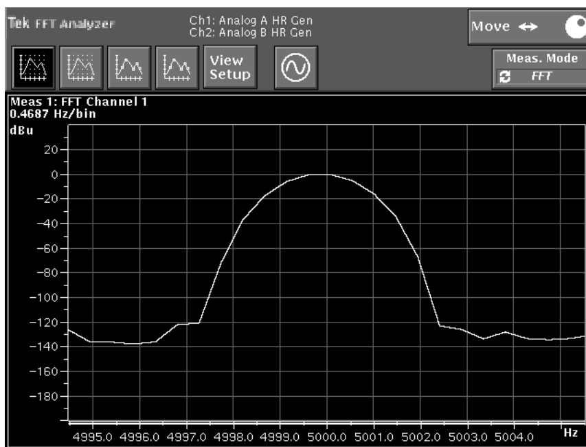
Figure 4-41: Zoomed FFT display showing maximum expansion of the trace
