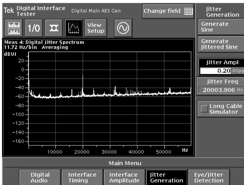
Figure 4-68: Digital Interface Tester Main Menu with Jitter Spectrum submenus
