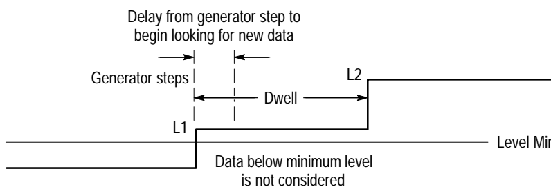
Figure 4-29: Regulation mode delay time setting
