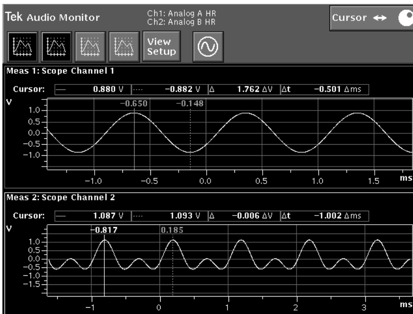
Figure 4-49: Dual channel display showing different signals on Channel 1 and Channel 2
