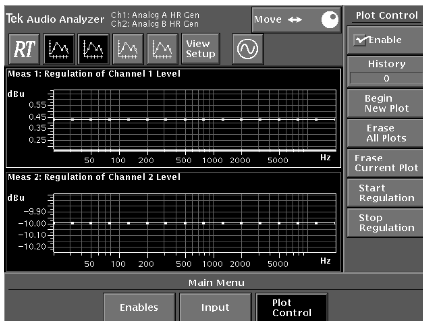
Figure 4-17: Regulation mode with Plot Control menu
