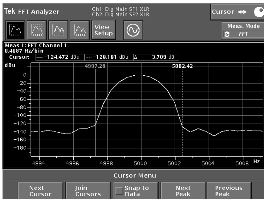
Figure 2-8: Cursor menu showing frequency and level readouts
