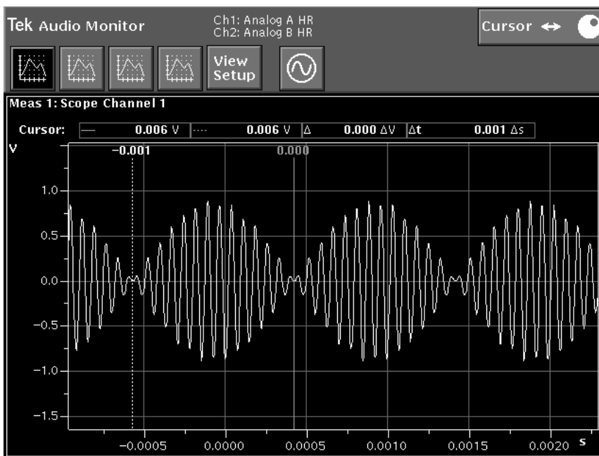
Figure 4-52: Use of Cursors to measure pulse time
