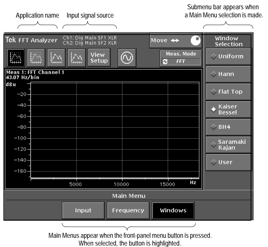
Figure 2-2: Touch screen interface with main menus and submenus displayed
