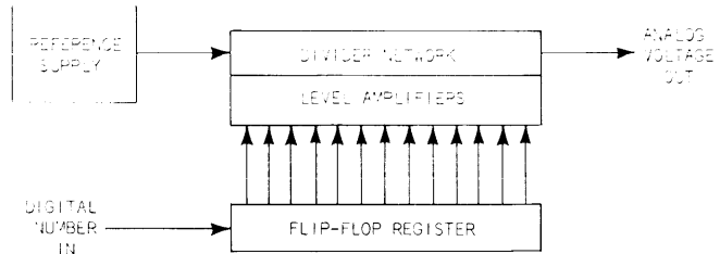
Fig. 8-1. Digital-to-analog converter.
