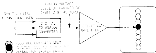
Fig. 9-3. Driving system addressibility.
