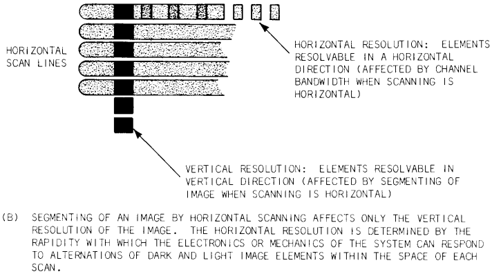
Fig. 9-8. TV resolution.
