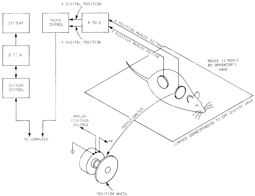
Fig. 7-3. X-Y mouse.
