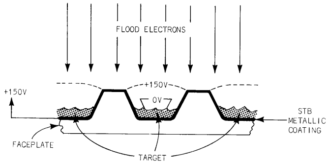
Fig. 9-7. Raised collector target.
