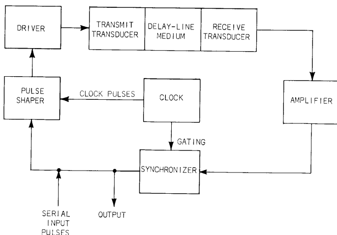
Fig. 6-5. Delay-line memory.
