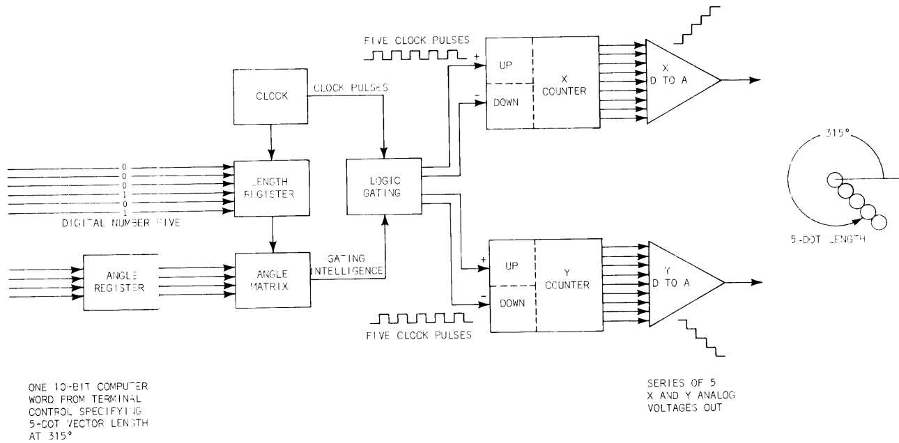
Fig. 8-5. Vector generator.
