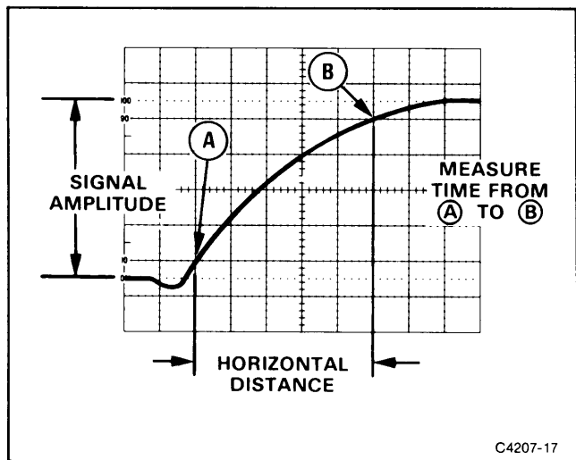
Figure 4-7. Rise time.
