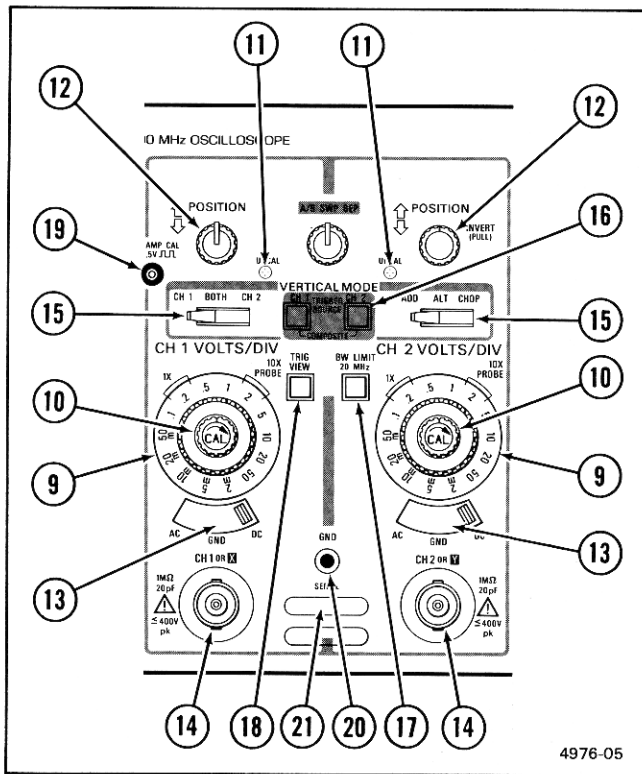
Figure 2-4. Vertical controls, connectors, and indicators.
