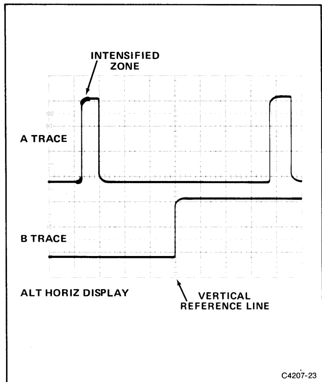
Figure 4-13. Time difference on single waveform.
