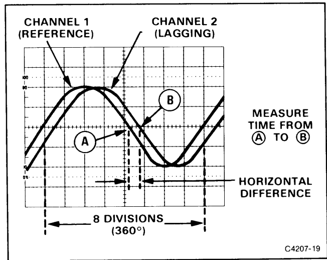
Figure 4-9. Phase difference.
