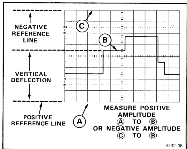
Figure 4-3. Instantaneous voltage measurement.
