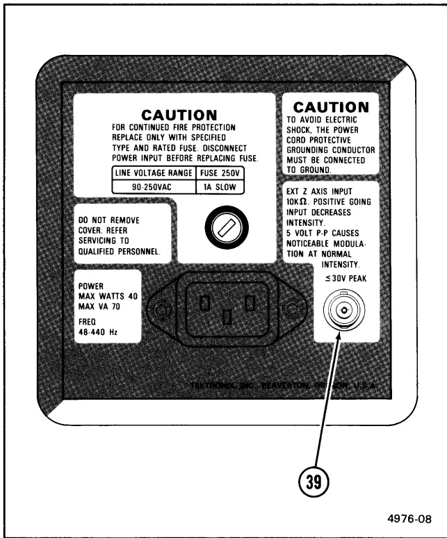
Figure 2-7. Rear-panel connector.
