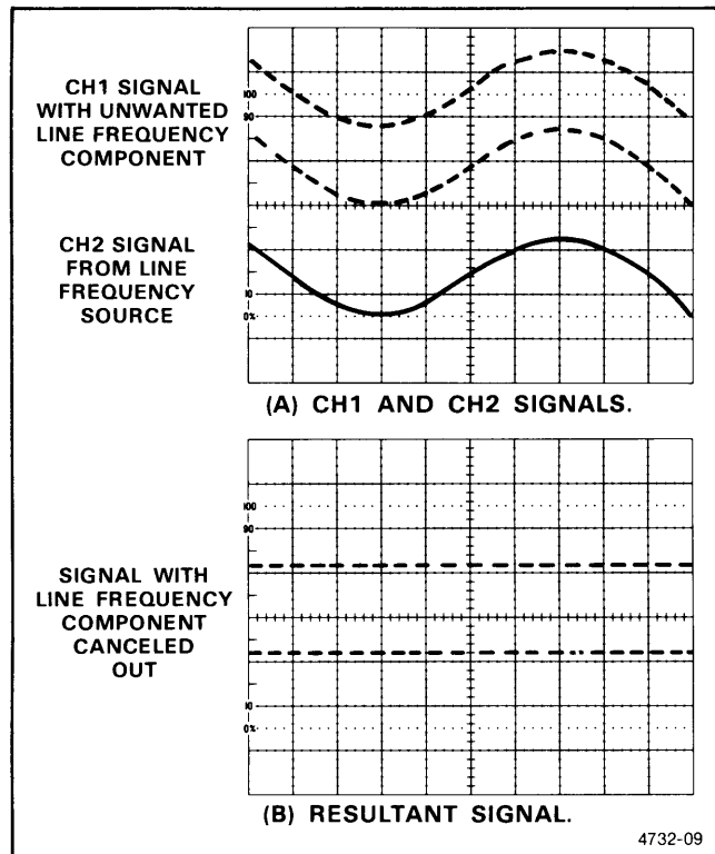
Figure 4-4. Common-mode rejection.
