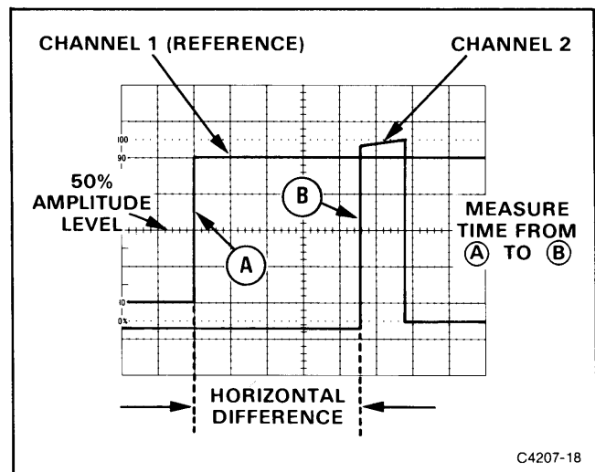
Figure 4-8. Time difference between pulses on time-related signals.
