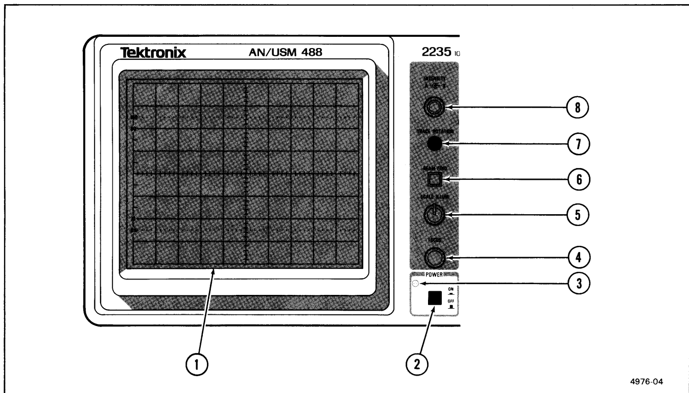
Figure 2-3. Power and display controls and indicator.
