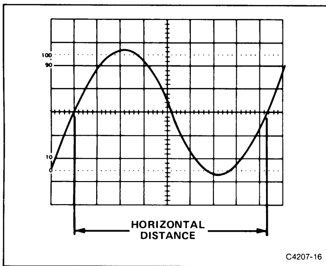
Figure 4-6. Time duration.
