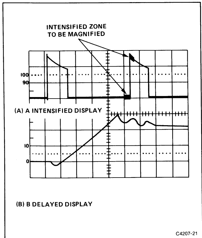
Figure 4-11. Delayed-sweep magnification.
