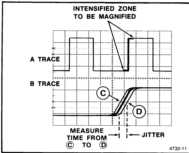
Figure 4-12. Pulse jitter.
