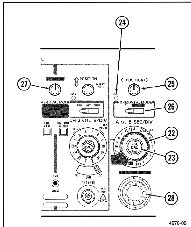
Figure 2-5. Horizontal controls and indicator.
