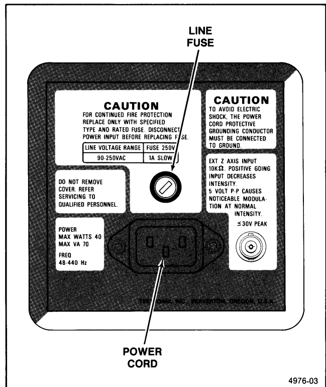
Figure 2-2. Fuse holder and power cord connector.
