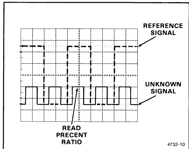
Figure 4-5. Voltage ratios.
