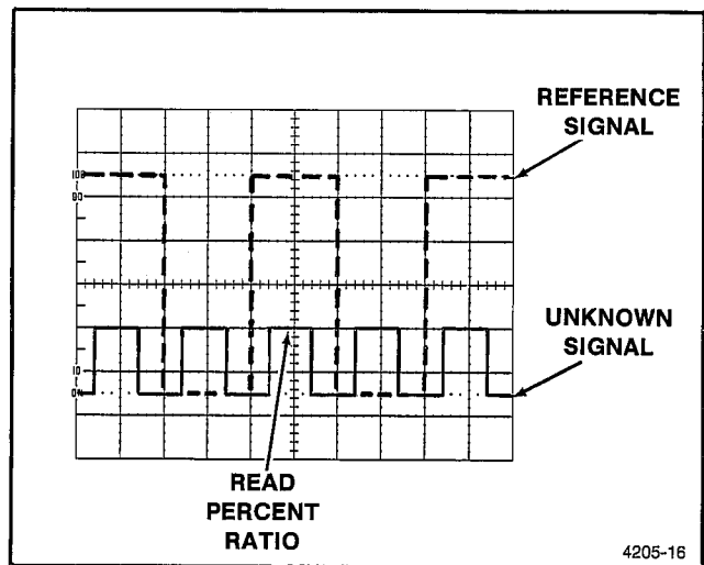
Fig. 4-4. Voltage ratios.
