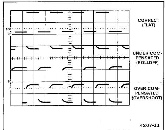
Fig. 3-2. Probe compensation.
