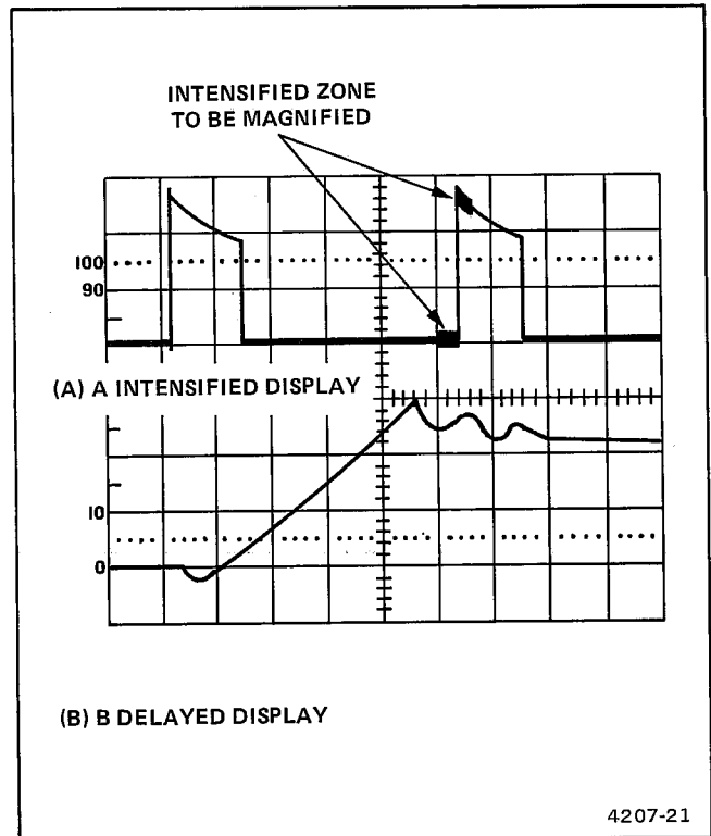
Fig. 4-5. Delayed-sweep magnification.
