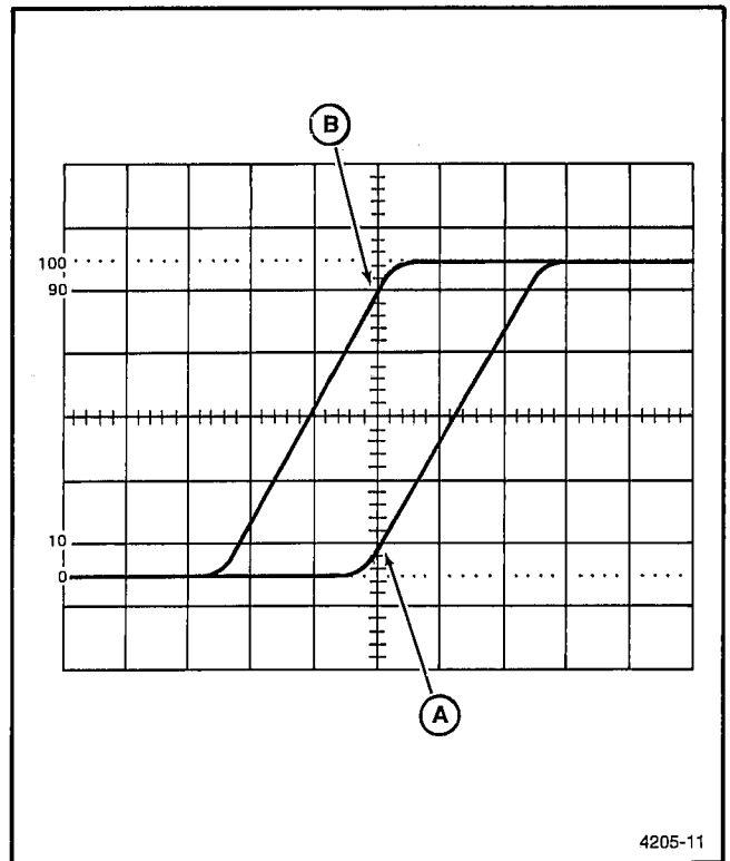
Fig. 4-7. Rise time.
