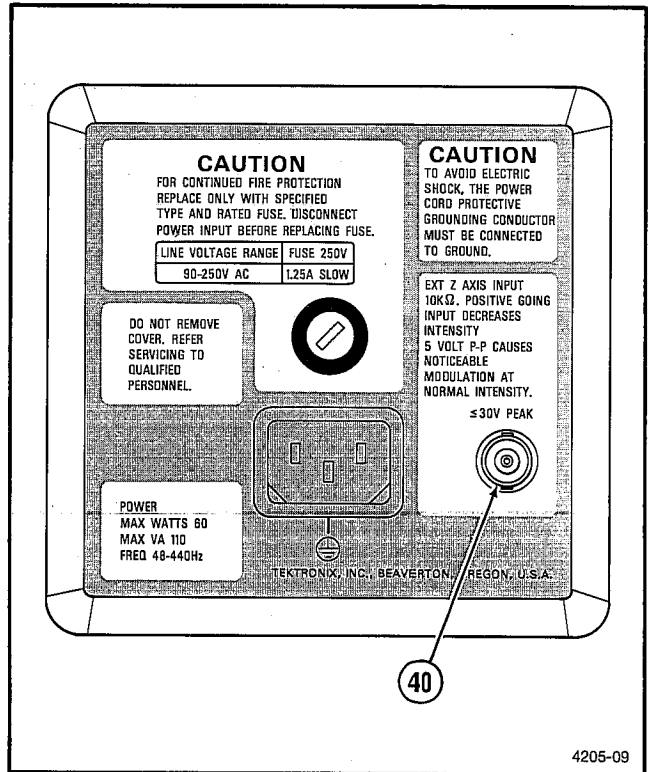
Fig. 2-9. Rear-panel connector.
