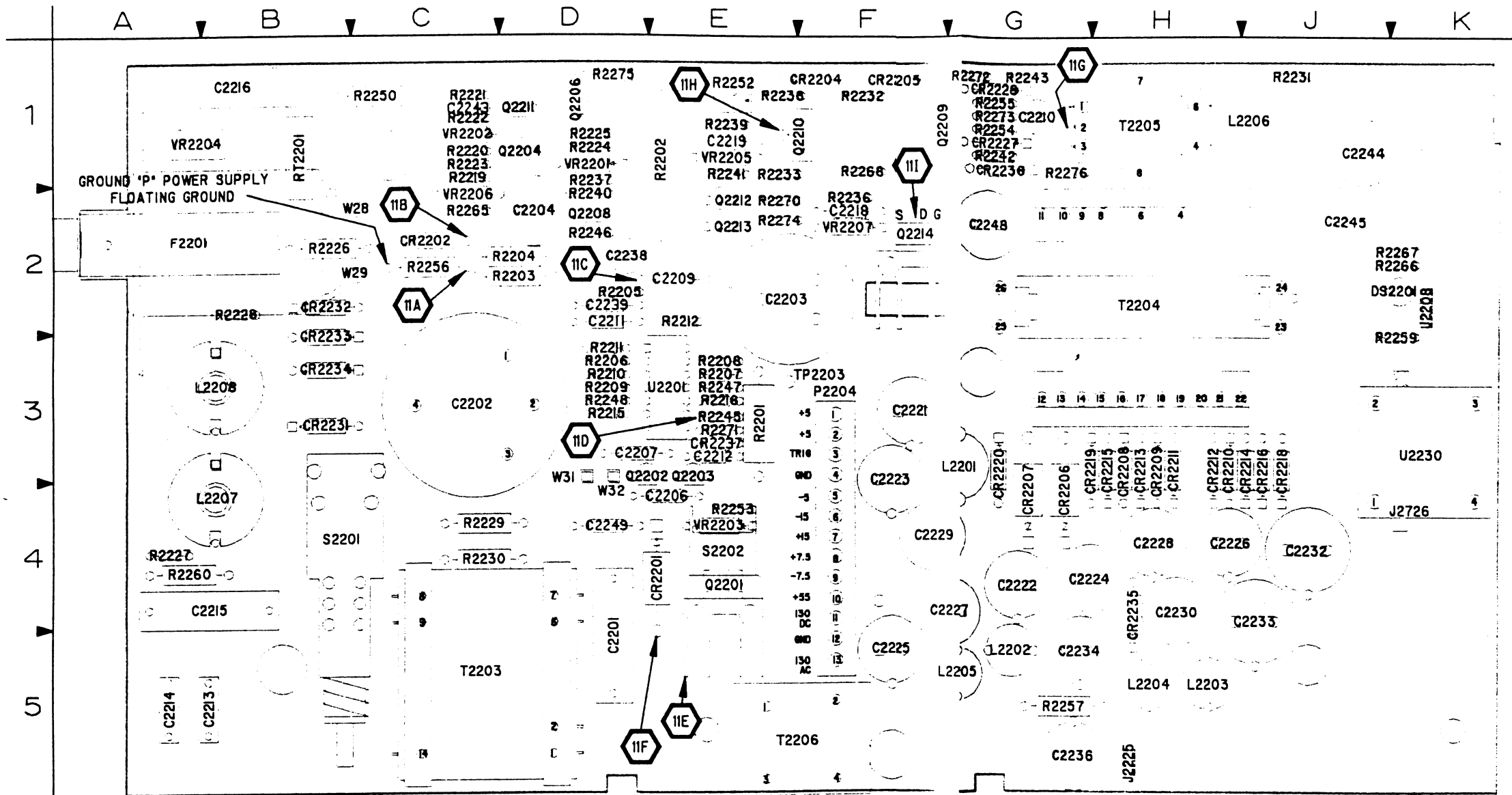
Figure 9-10. A18—Power Supply board.
