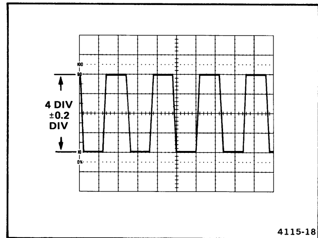
Figure 12. Vertical display accuracy.
