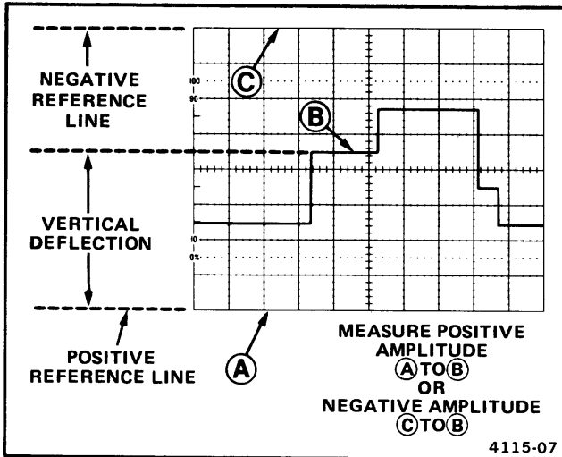
Figure 14. Instantaneous voltage measurement.
