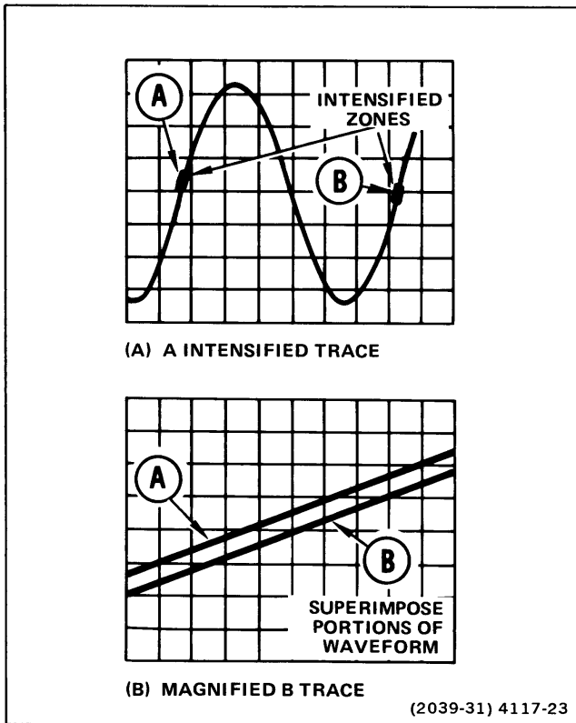
Figure 24. Time duration using delayed sweep.
