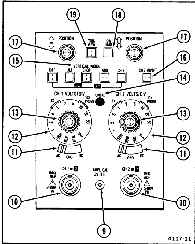
Figure 4. Vertical controls, connectors, and indicators and calibrator output.
