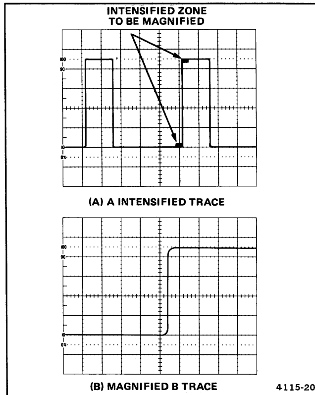
Figure 22. Delayed-sweep magnification.
