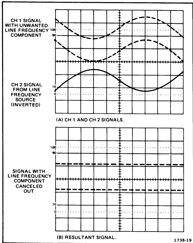
Figure 16. Common-mode rejection.
