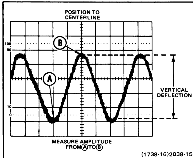
Figure 13. Peak-to-peak waveform voltage.
