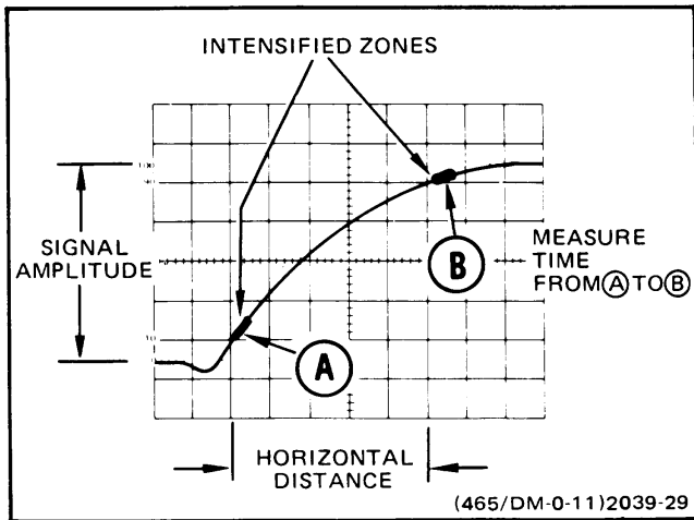
Figure 25. Rise time, differential time method.
