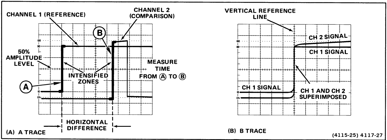
Figure 27. Time difference between two time-related pulses.
