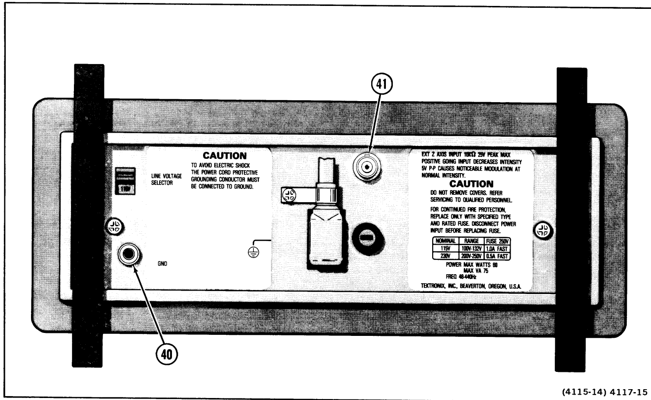
Figure 8. Rear-panel connectors.
