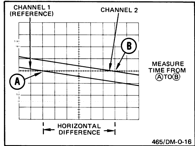
Figure 21. High-resolution phase difference.
