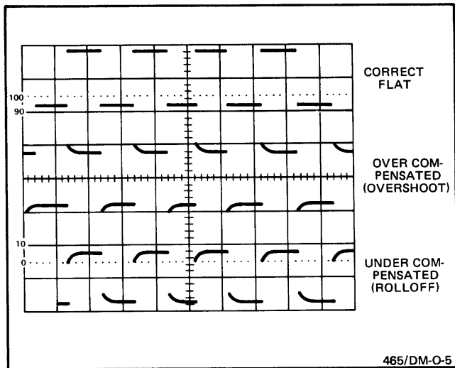
Figure 11. Probe compensation.
