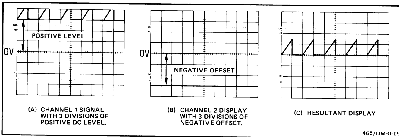
Figure 15. Algebraic addition.
