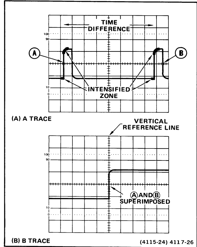
Figure 26. Time difference between repetitive pulses.
