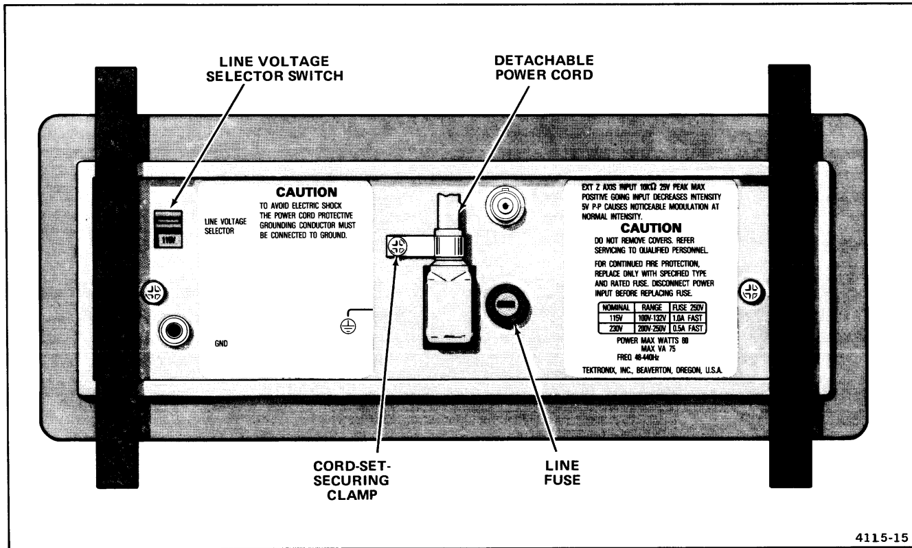
Figure 1. LINE VOLTAGE SELECTOR switch, line fuse, and power cord.
