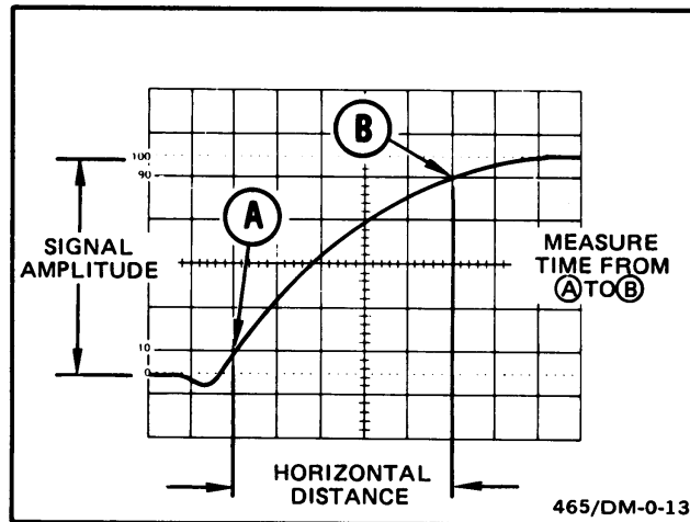
Figure 18. Rise time.
