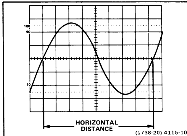
Figure 17. Time duration.
