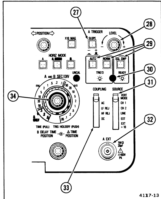
Figure 6. A TRIGGER controls, connector, and indicator.
