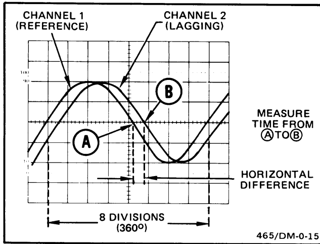
Figure 20. Phase difference.
