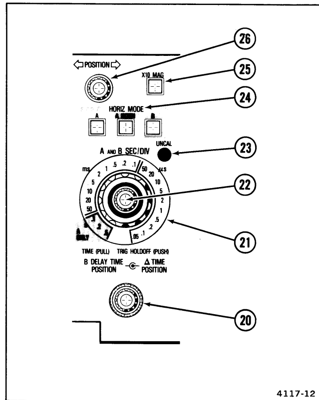
Figure 5. Horizontal controls and indicator.
