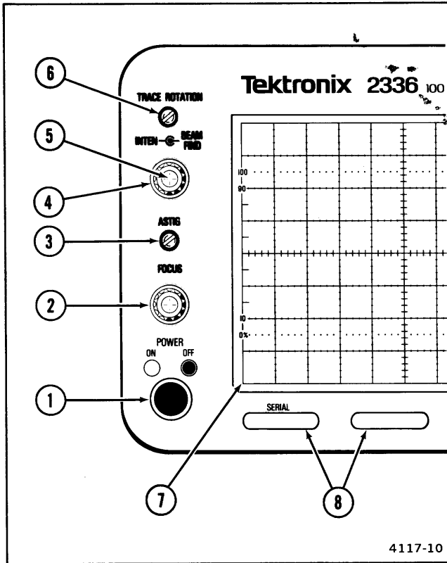
Figure 3. Power and display controls and indicators.
