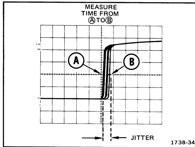
Figure 23. Pulse jitter.
