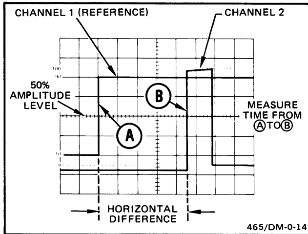
Figure 19. Time difference between two time-related pulses.
