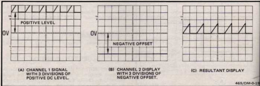
Figure 16. Algebraic addition.
