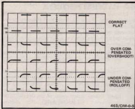
Figure 11. Probe compensation.
