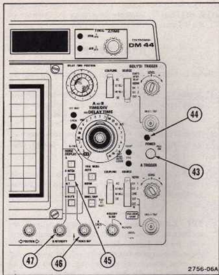
Figure 6. Horizontal and power controls and indicators.
