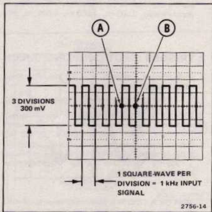
Figure 13. DM44 timing check.
