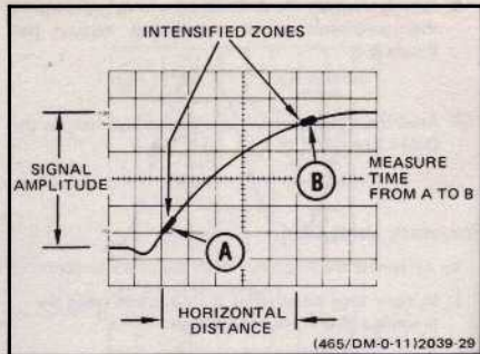
Figure 31. Rise time.
