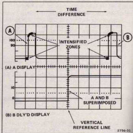
Figure 27. Time difference between repetitive pulses.
