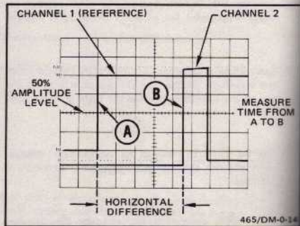
Figure 20. Time difference between two time-related pulses.
