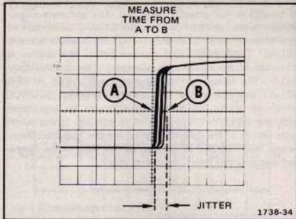
Figure 23. Pulse jitter.
