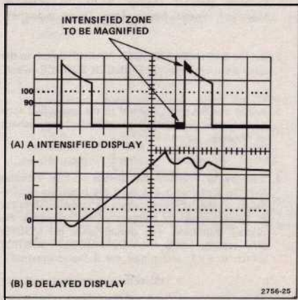
Figure 24. Delayed sweep magnification.
