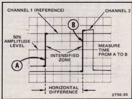
Figure 28. Time difference between two time-related pulses.
