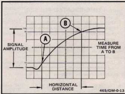
Figure 19. Rise time.
