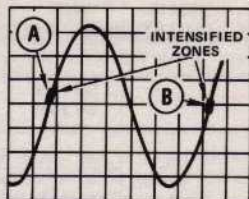
(A) A SWEEP DISPLAY
