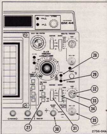
Figure 4. Trigger controls, connectors, and indicators.
