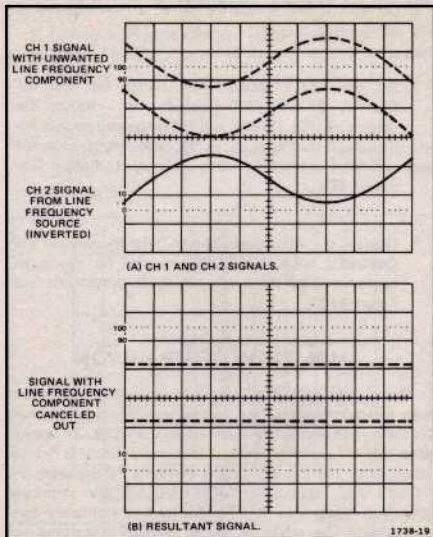
Figure 17. Common-mode rejection.
