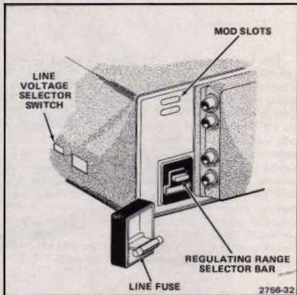
Figure 1. Regulating range selection and line fuse.
