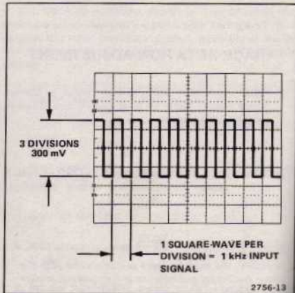
Figure 12. Basic 465B timing check.
