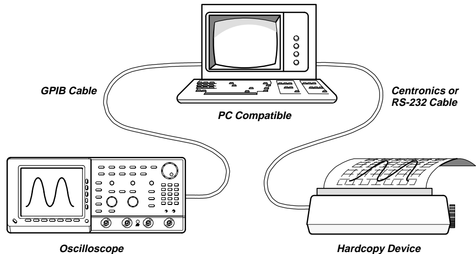
Figure 3-21: Connecting the Oscilloscope and Hardcopy Device Via a PC
