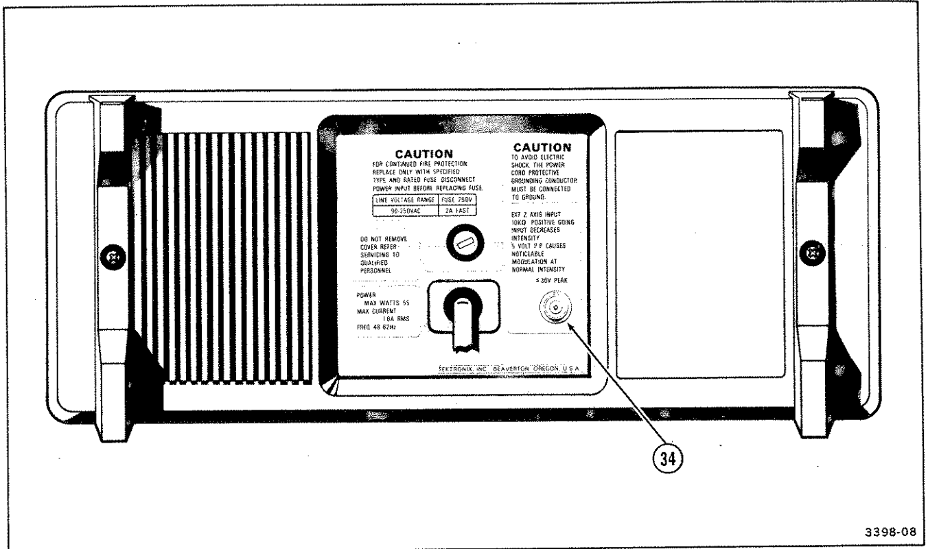
Figure 7. Rear-panel connector.
