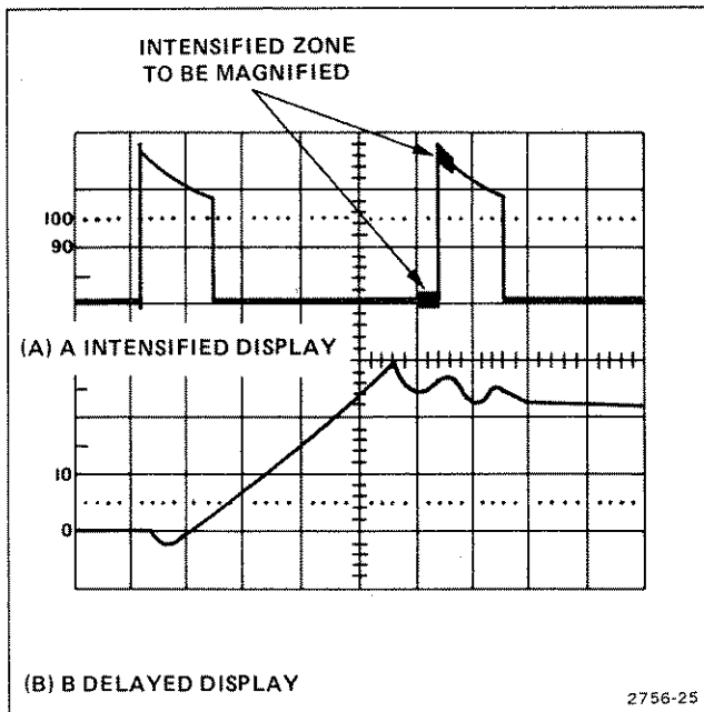
Figure 20. Delayed-sweep magnification.
