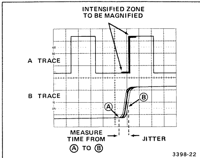
Figure 21. Pulse jitter.
