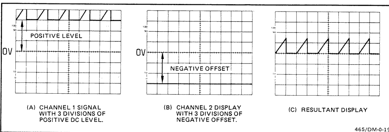
Figure 13. Algebraic addition.
