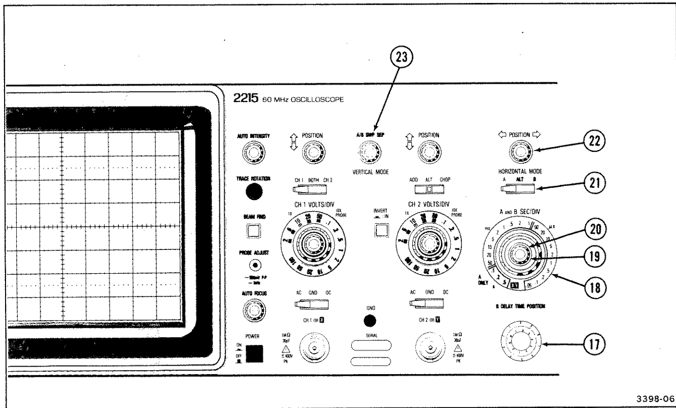
Figure 5. Horizontal controls.
