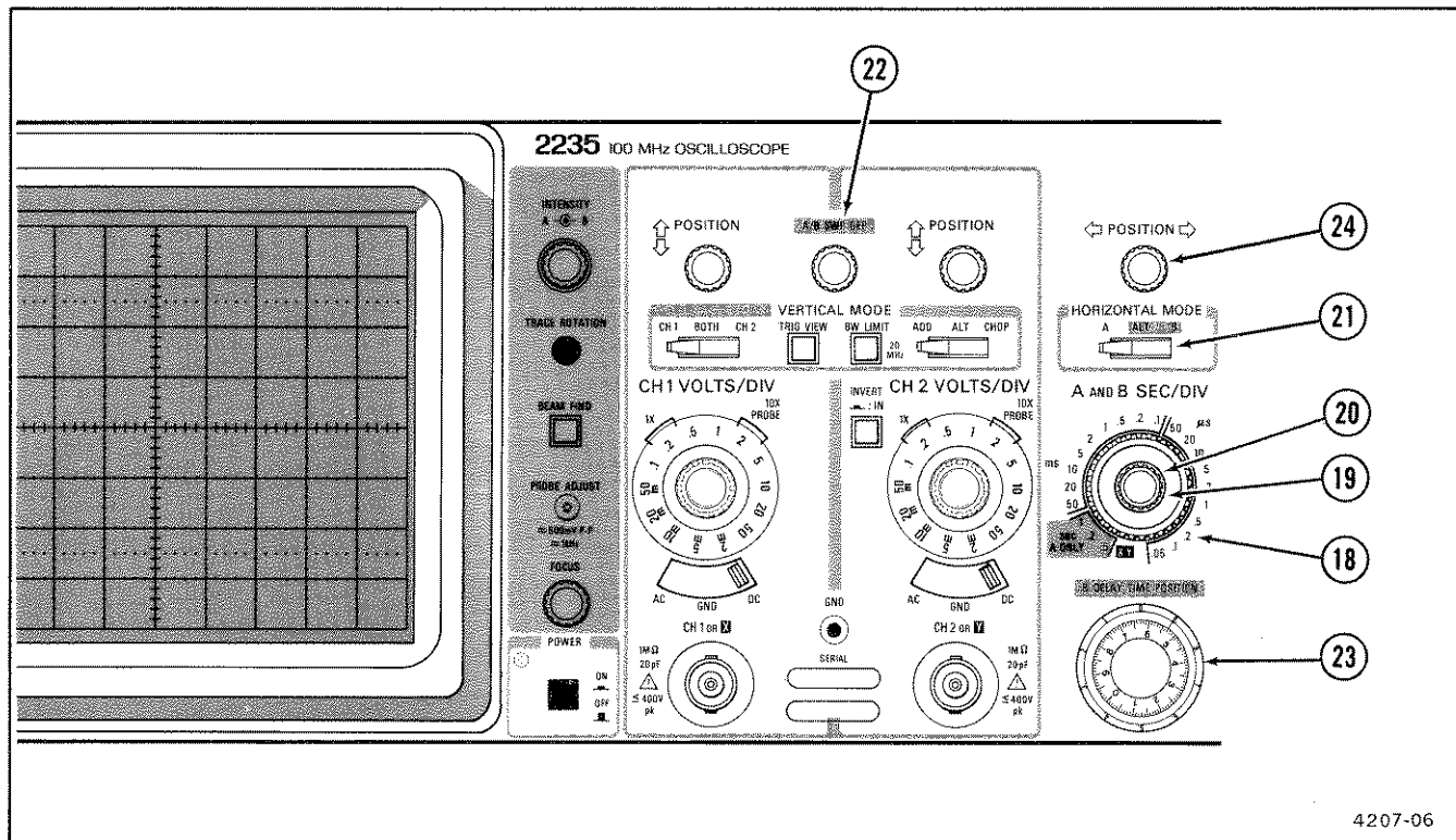
Figure 2-5. Horizontal controls.
