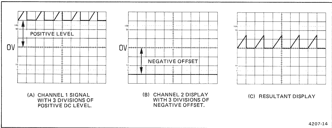
Figure 4-4. Algebraic addition.
