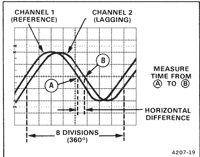
Figure 4-9. Phase difference.
