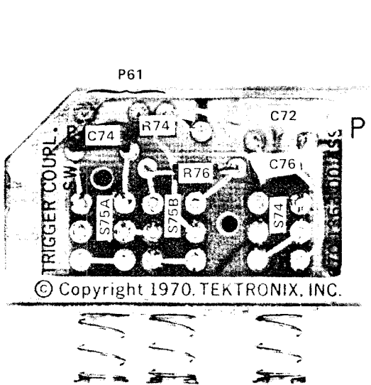
Fig. 8-10. P/O A2. Partial Vertical circuit board.
