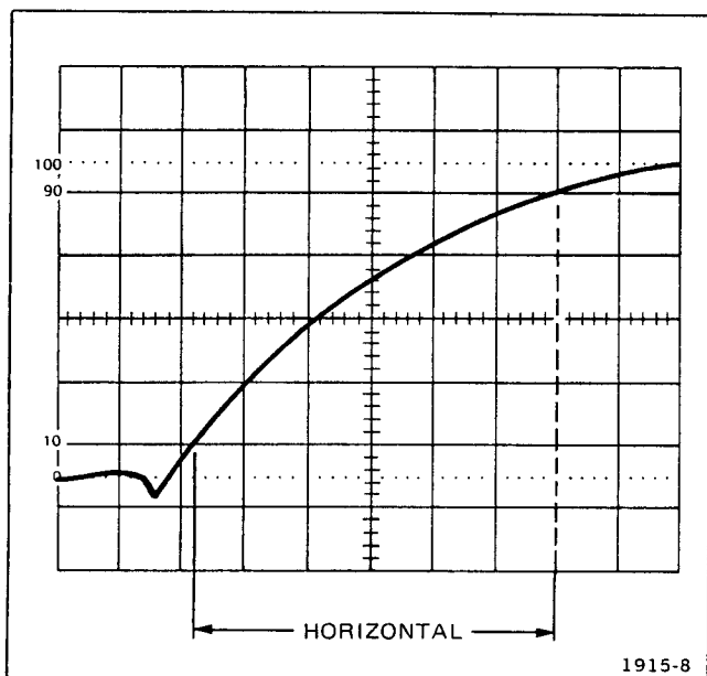
Fig. 2-10. Measuring risetime.
