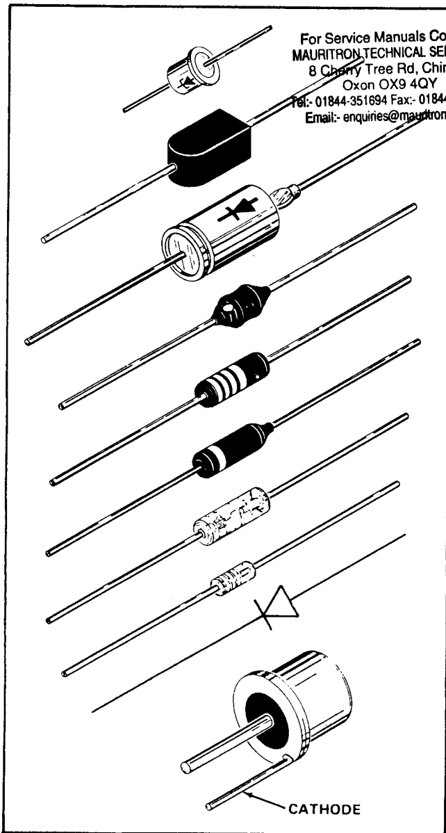
Fig. 4-3. Diode polarity markings.
