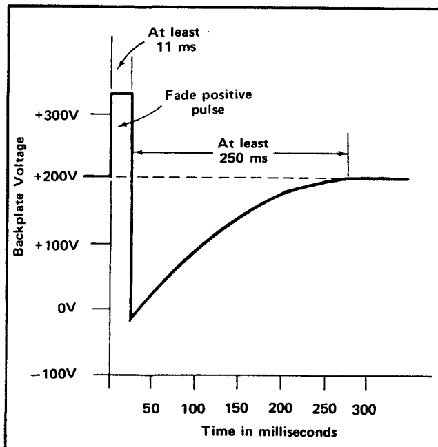
Fig. 3-21. Typical erase cycle waveform.
