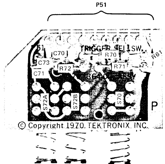
Fig. 8-10. P/O A2. Partial Vertical circuit board.
