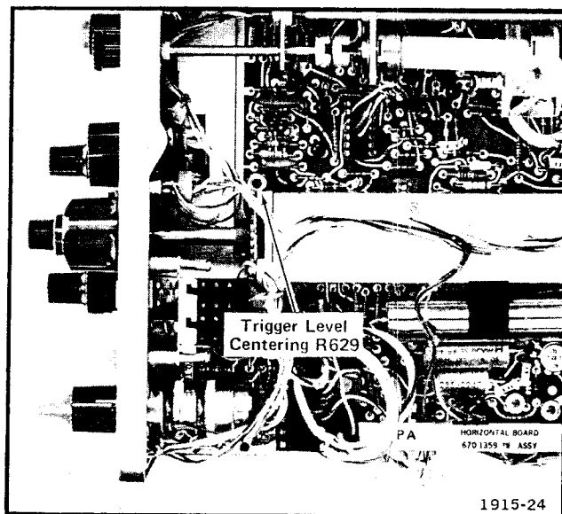
Fig. 5-7. Location of Trigger Level Centering adjustment.
