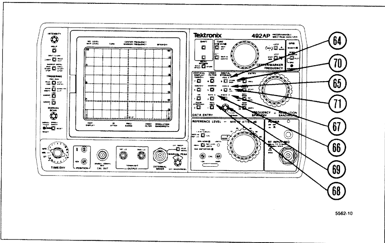
Figure 4-11. Digital Storage.
