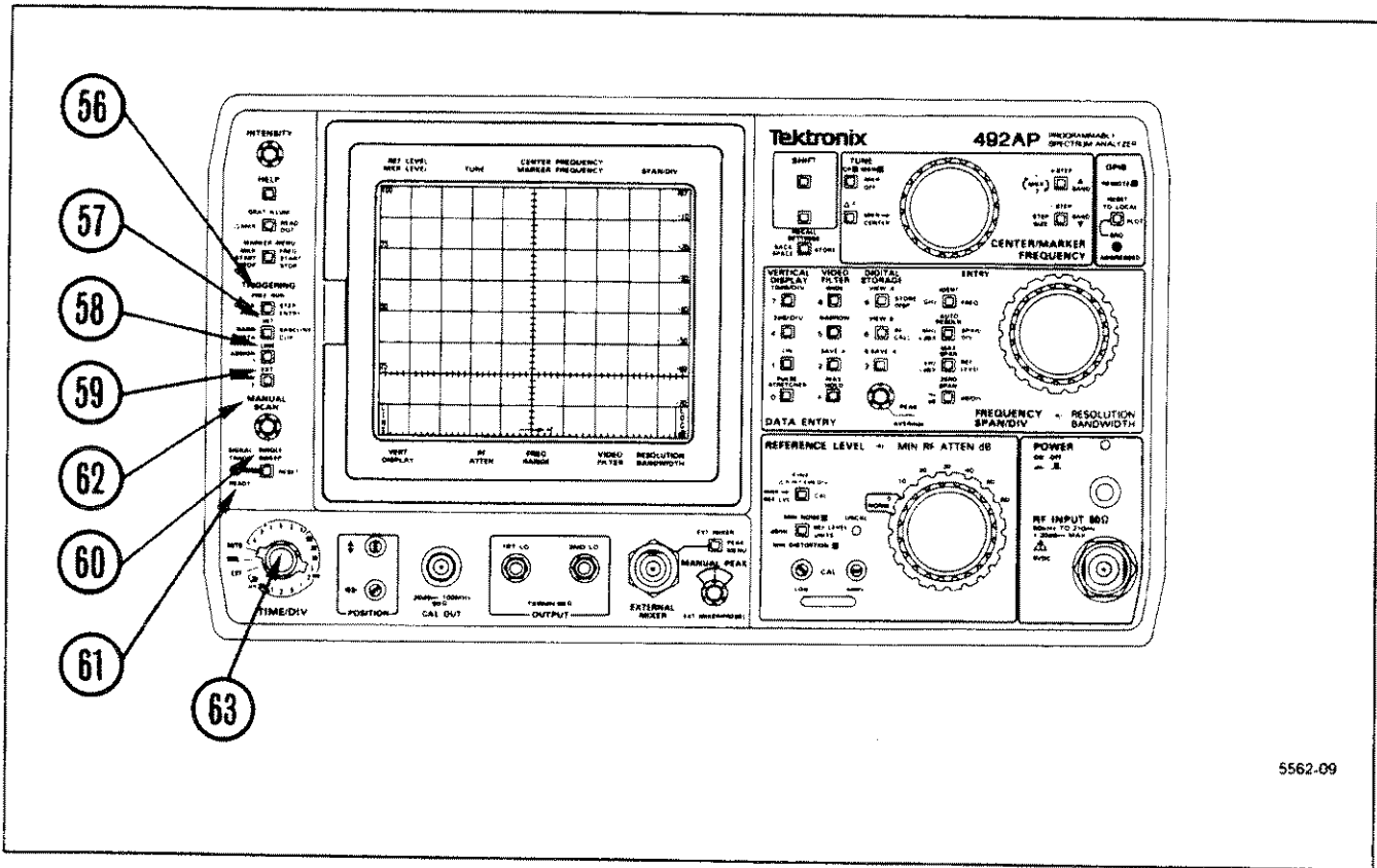
Figure 4-10. Sweep.
