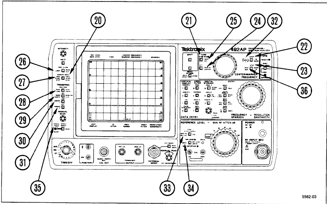
Figure 4-3. Marker Functions.
