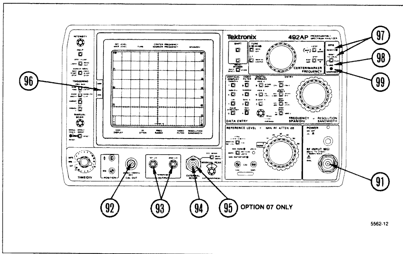
Figure 4-13. Front-panel input/output and GPIB.
