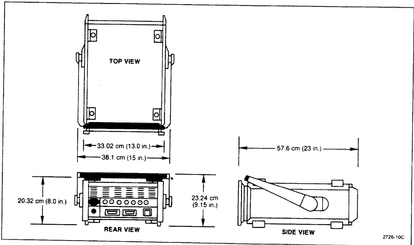
Figure 2-1. Dimensions.
