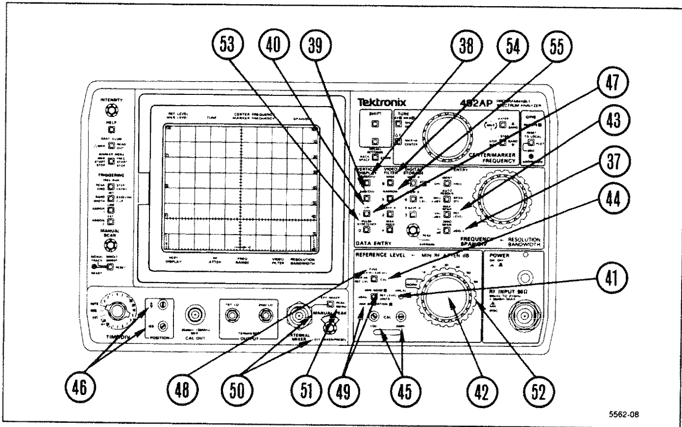
Figure 4-9. Display Parameters.
