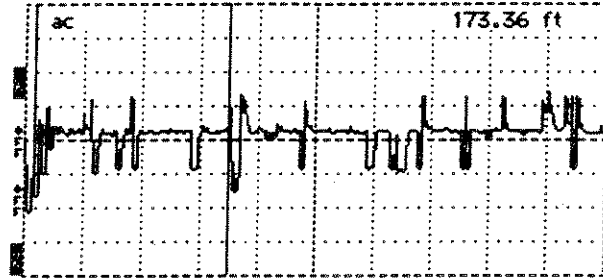
1B - Traffic and tap nearly identical (4 avg, 50 ft/DIV, 35.00 dB gain)
