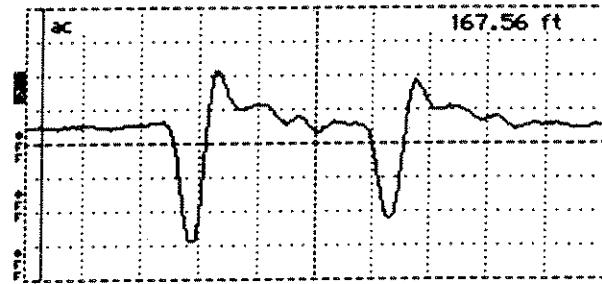
1F - Tap expanded, no traffic (1 avg, 2 ft/DIV, 35.00 gain)
