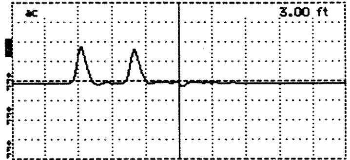
V_p of .30 when it should have been .66 for 3 foot cable.
