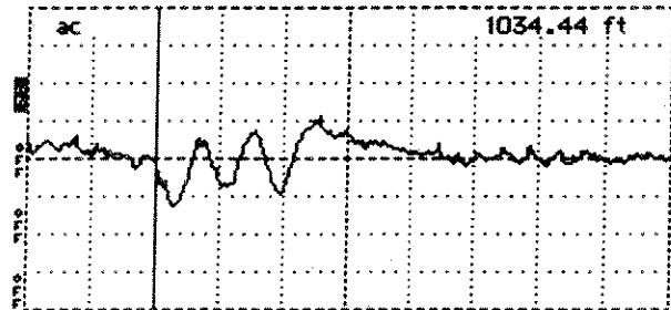
2I - Group of taps expanded (128 avg, 10 ft/DIV, 54.75 dB gain)
