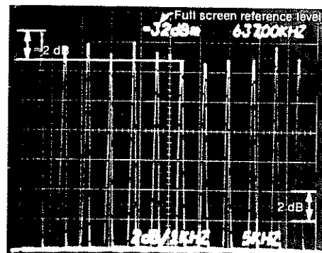
Fig. 1. Spectrum display of unmodulated carriers for 12 channel bank.
