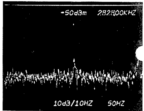
Fig. 6. Three tone intermodulation product at 2828 kHz.
