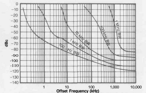
Typical filler shape, phase noise sidebands, and sensitivity factors for fundamental mixing on a preselected 492 (Option 01).
