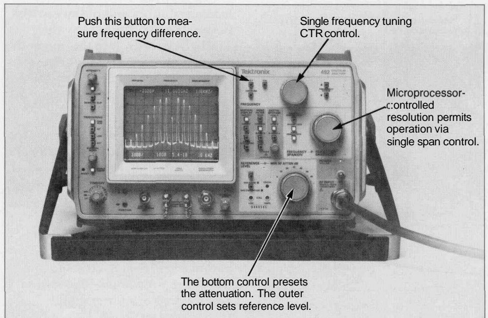
Figure 1. The three main elements, frequency, frequency span and amplitude reference, are controlled by three knobs.
